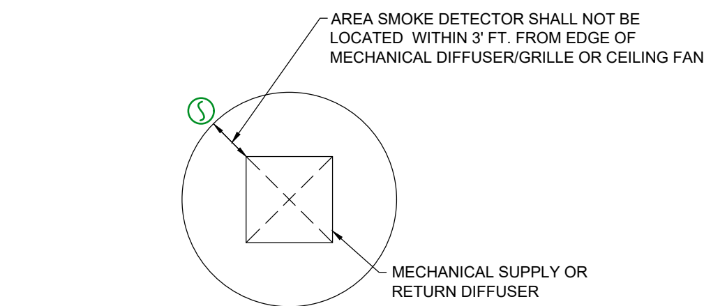
SMOKE DETECTOR INSTALLATION DETAIL SCALE: NTS
