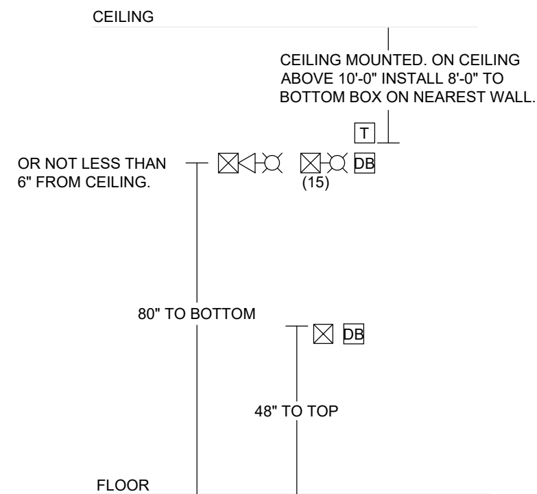
FIRE ALARM DEVICE MOUNTING DETAIL SCALE: NTS
