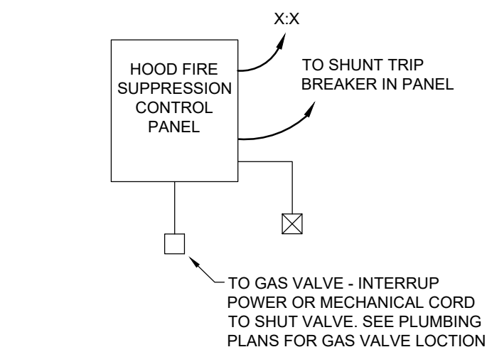
FIRE SUPPRESSION SYSTEM RISER DIAGRAM SCALE: NTS
