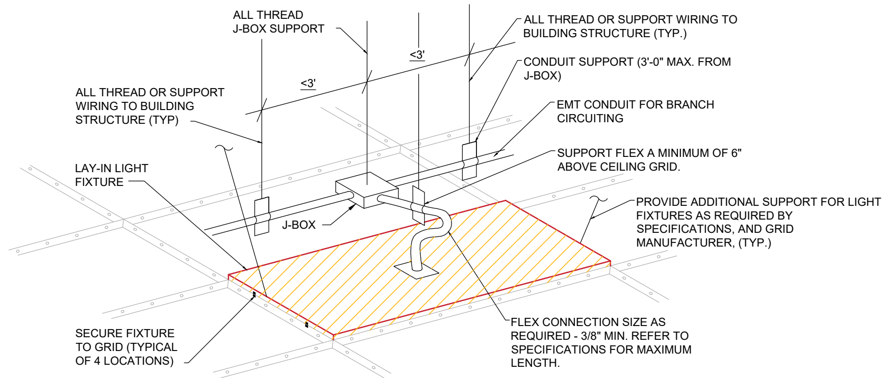
LIGHT FIXTURE INSTALLATION DETAIL SCALE: NTS
