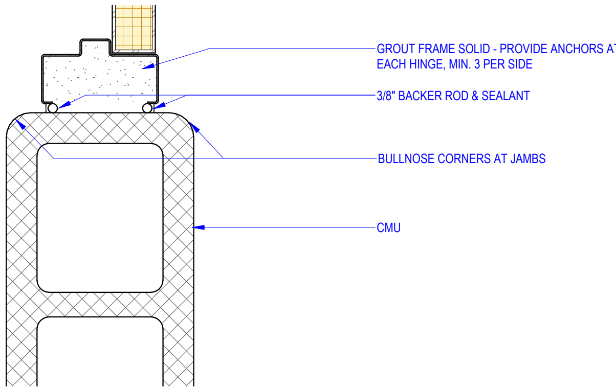
D4 DOOR JAMB 3" = 1'-0"
