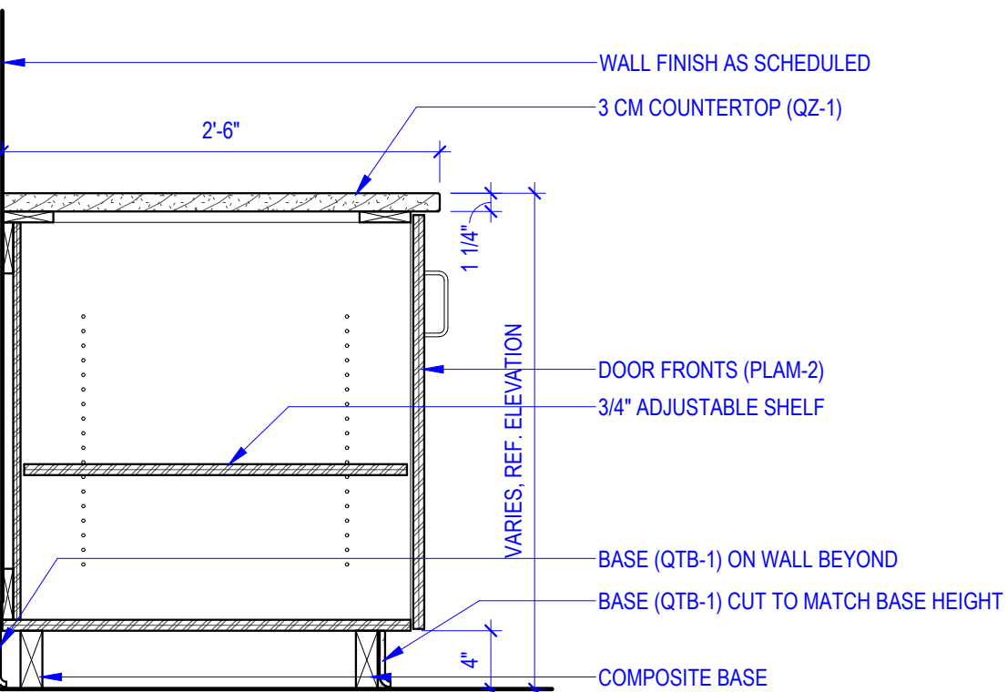
E3 BASE CABINET 1" = 1'-0" BAR
