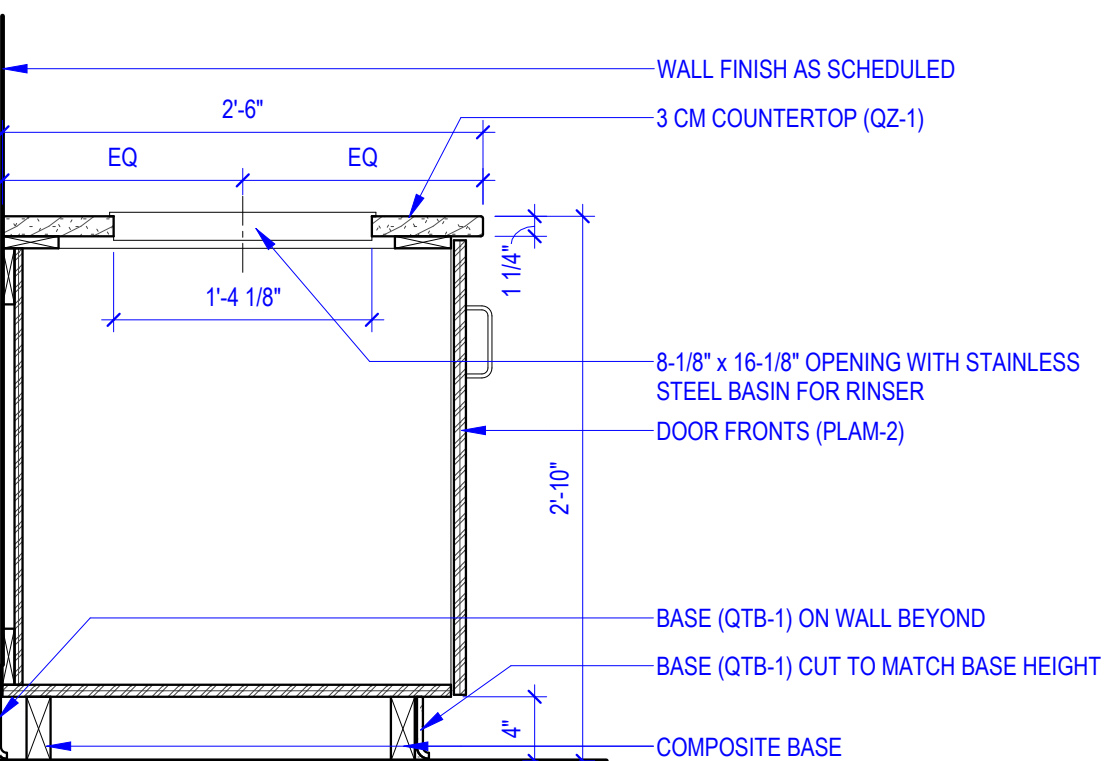
E4 BASE CABINET 1" = 1'-0" BAR RINSER
