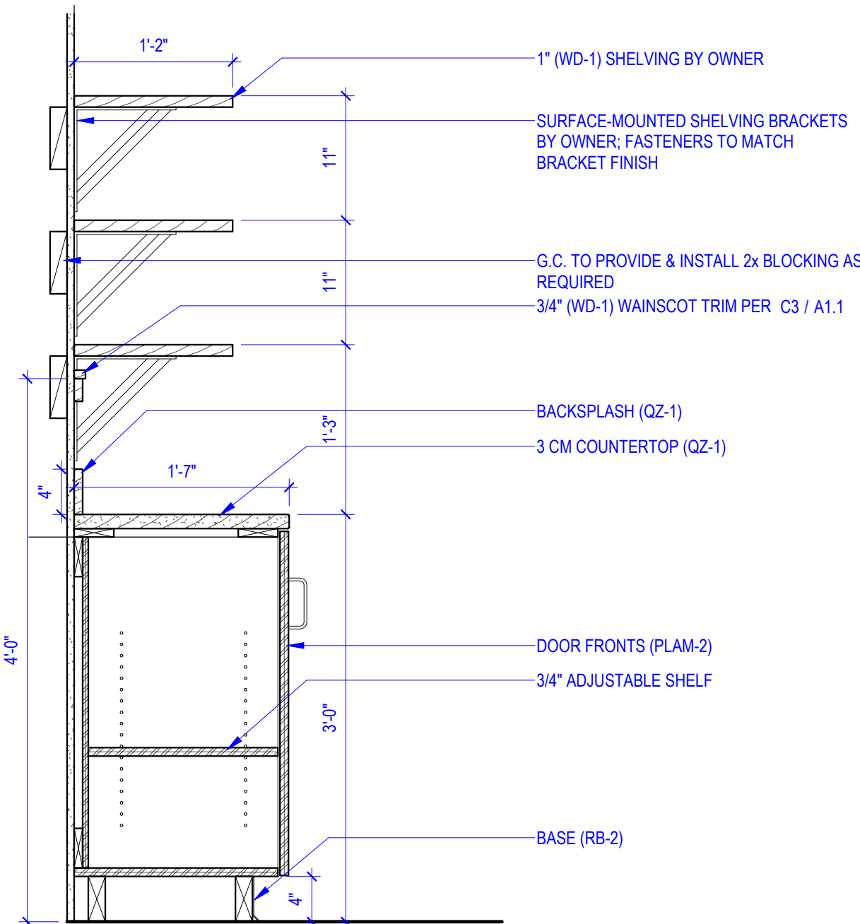
D3 BASE CABINET 1" = 1'-0" HUTCH
