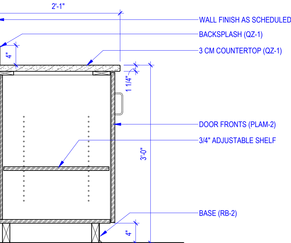
D4 BASE CABINET 1" = 1'-0" P.O.S.
