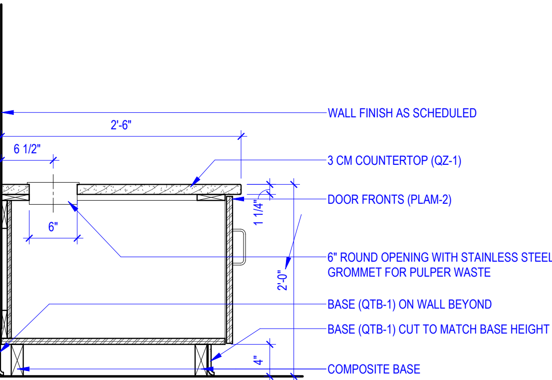
E2 BASE CABINET 1" = 1'-0" BAR PULPER
