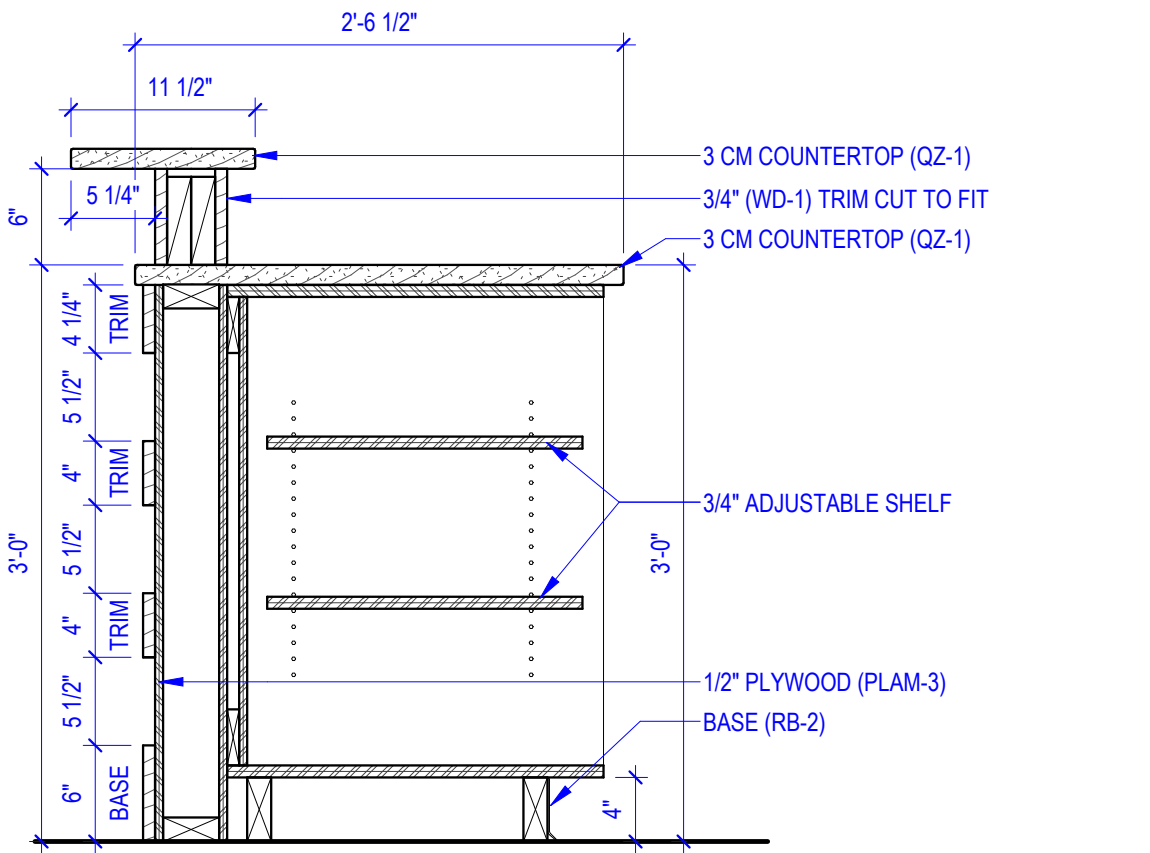
C2 BASE CABINET 1" = 1'-0" HOST OPEN BASE
