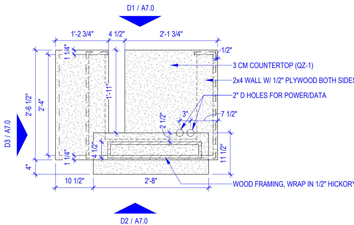
D4 HOST STAND PLAN 3/4" = 1'-0"
