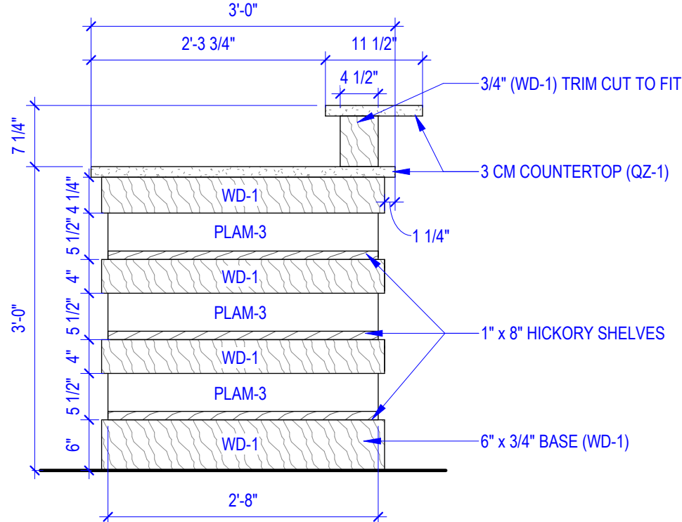
D2 HOST STAND ELEVATION 3/4" = 1'-0" FRONT
