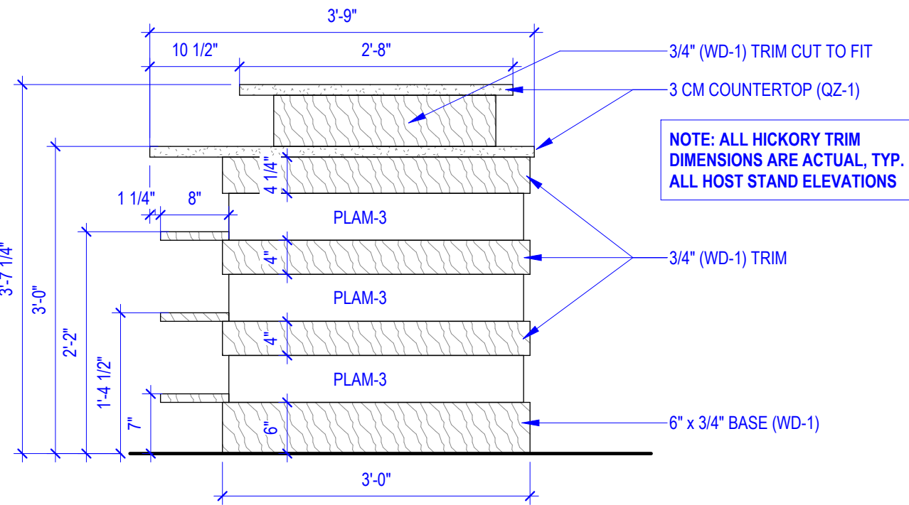
D1 HOST STAND ELEVATION 3/4" = 1'-0" REAR
