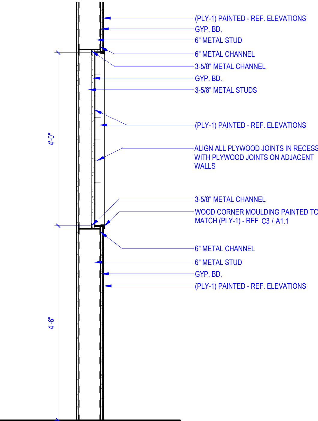
E2 WALL SECTION 3/4" = 1'-0" ARTWORK DISPLAY
