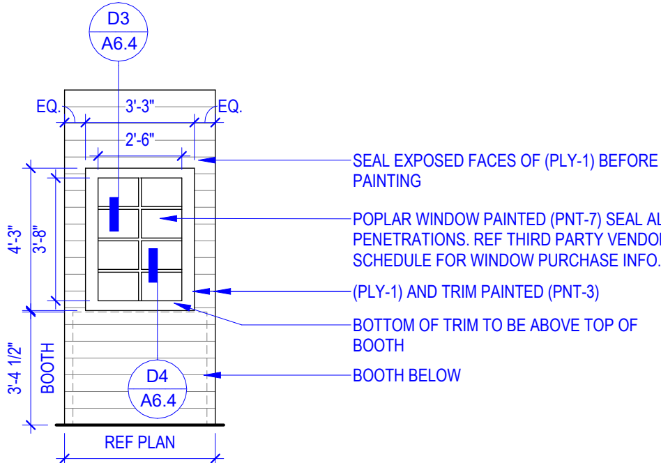
D1 WOODEN WINDOW 1/4" = 1'-0"
