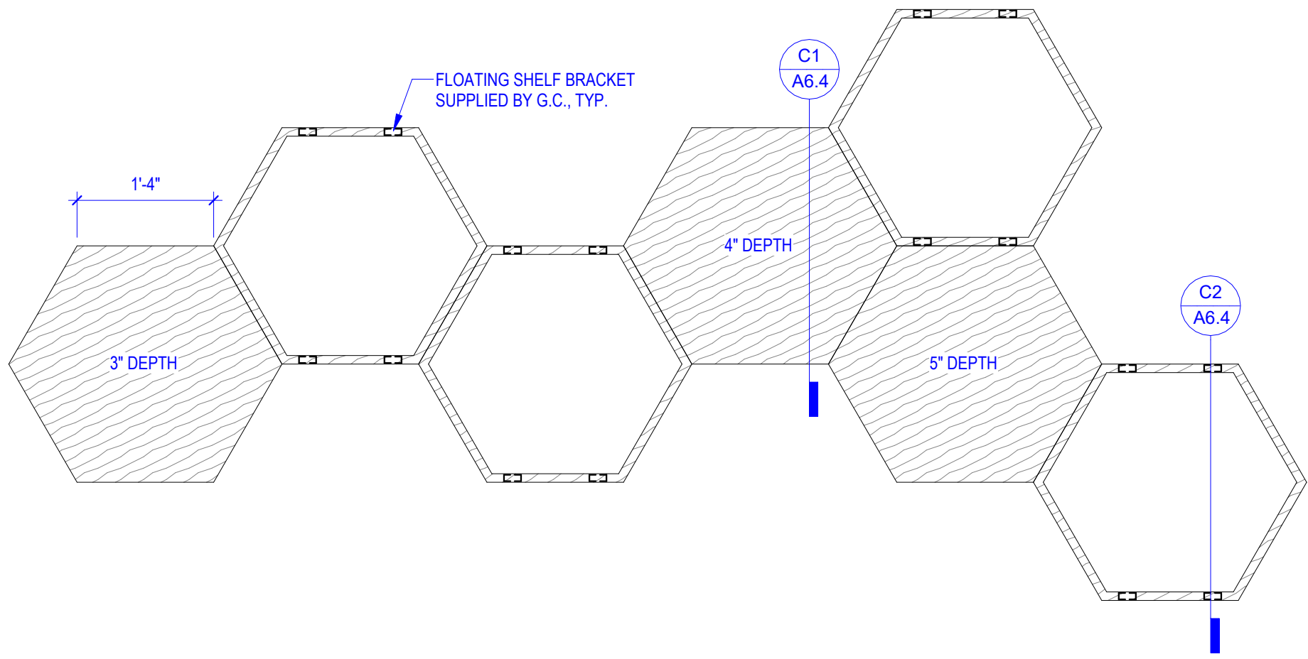
1 HEXAGON WALL FEATURE 3/4" = 1'-0"
