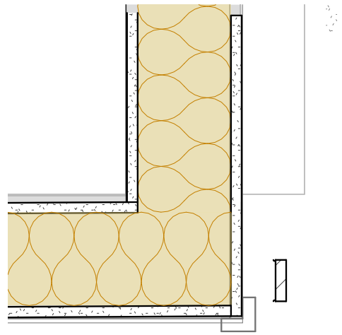
1 HEXAGON WALL FEATURE 3/4" = 1'-0"
