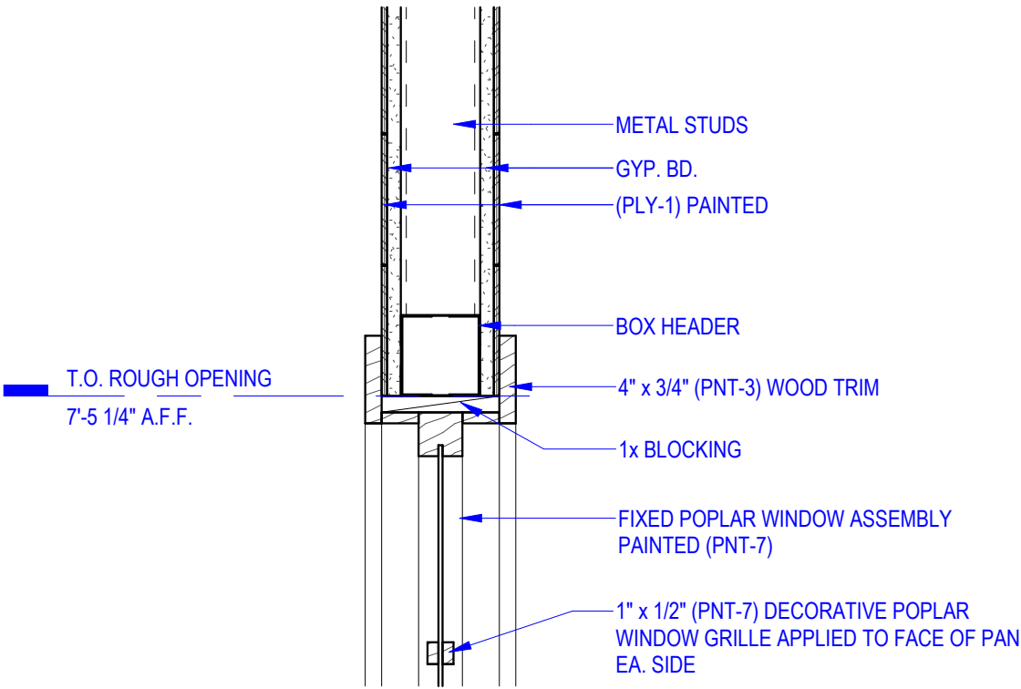
D3 POLAR WINDOW HEAD 1 1/2" = 1'-0"
