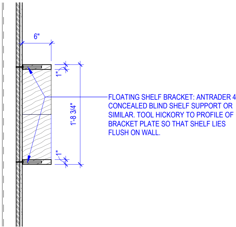
C2 HEXAGON SHELF 1" = 1'-0"
