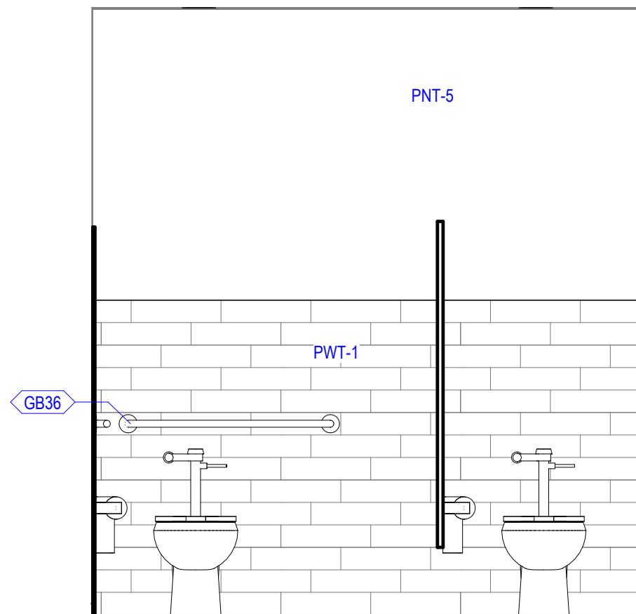
D5 INTERIOR ELEVATION 1/2" = 1'-0" @ WOMEN'S WEST
