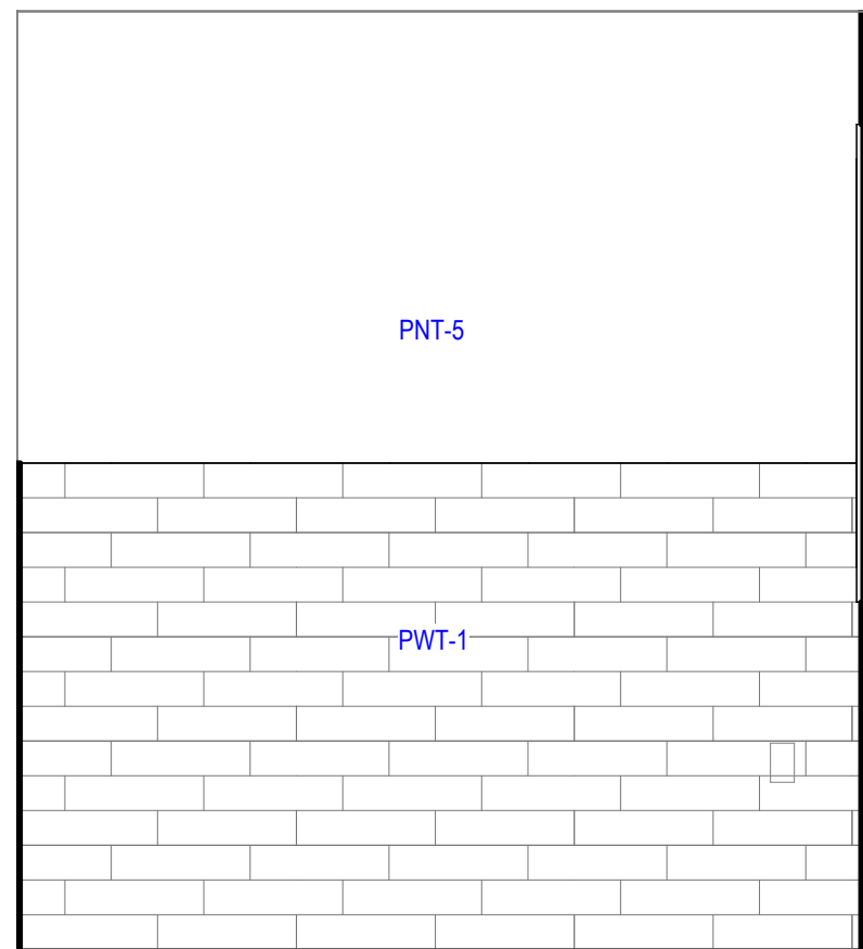
B5 INTERIOR ELEVATION 1/2" = 1'-0" @ WOMEN'S EAST
