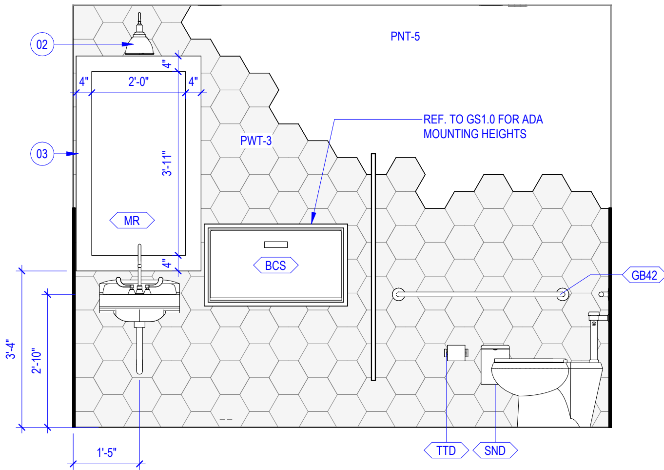
C5 INTERIOR ELEVATION 1/2" = 1'-0" @ WOMEN'S SOUTH
