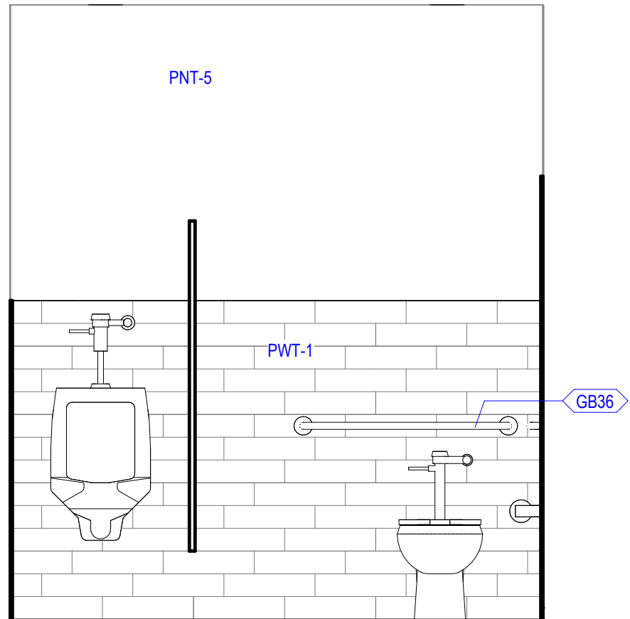
C4 INTERIOR ELEVATION 1/2" = 1'-0" @ MEN'S SOUTH
