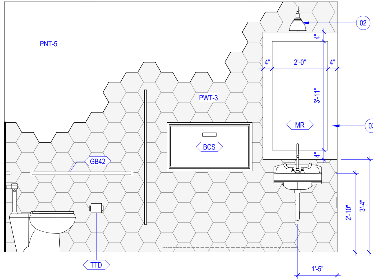
D4 INTERIOR ELEVATION 1/2" = 1'-0" @ MEN'S WEST
