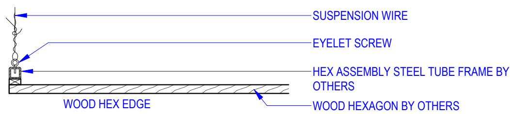
A2 ACT CLOUD EDGE 1 1/2" = 1'-0"
