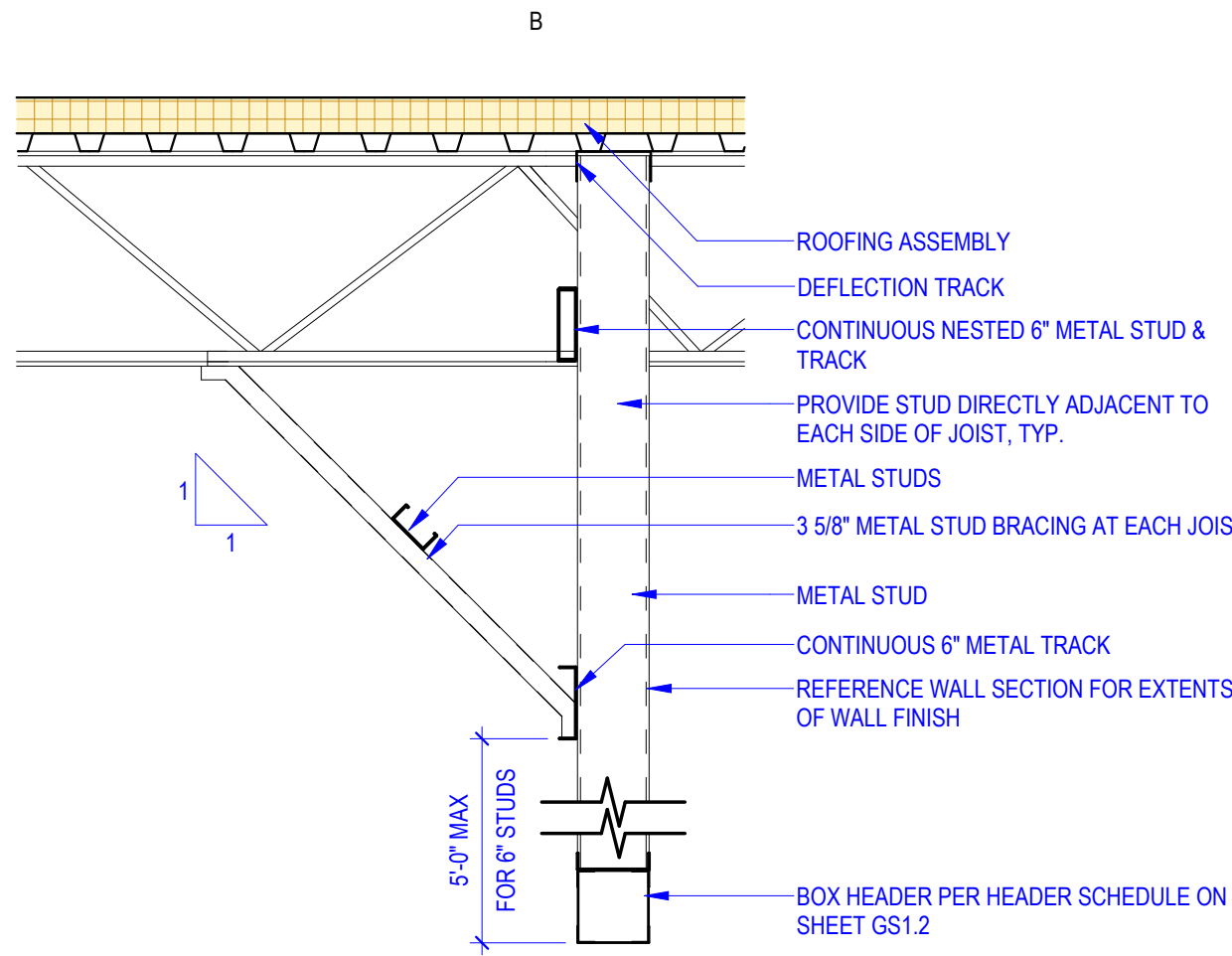
B1 BULKHEAD ATTACHMENT 3/4" = 1'-0"
