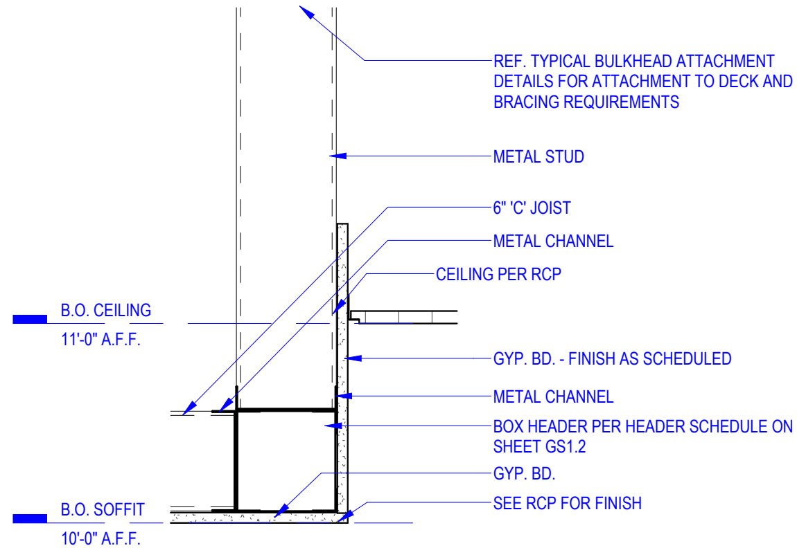
B2 SOFFIT 1 1/2" = 1'-0"
