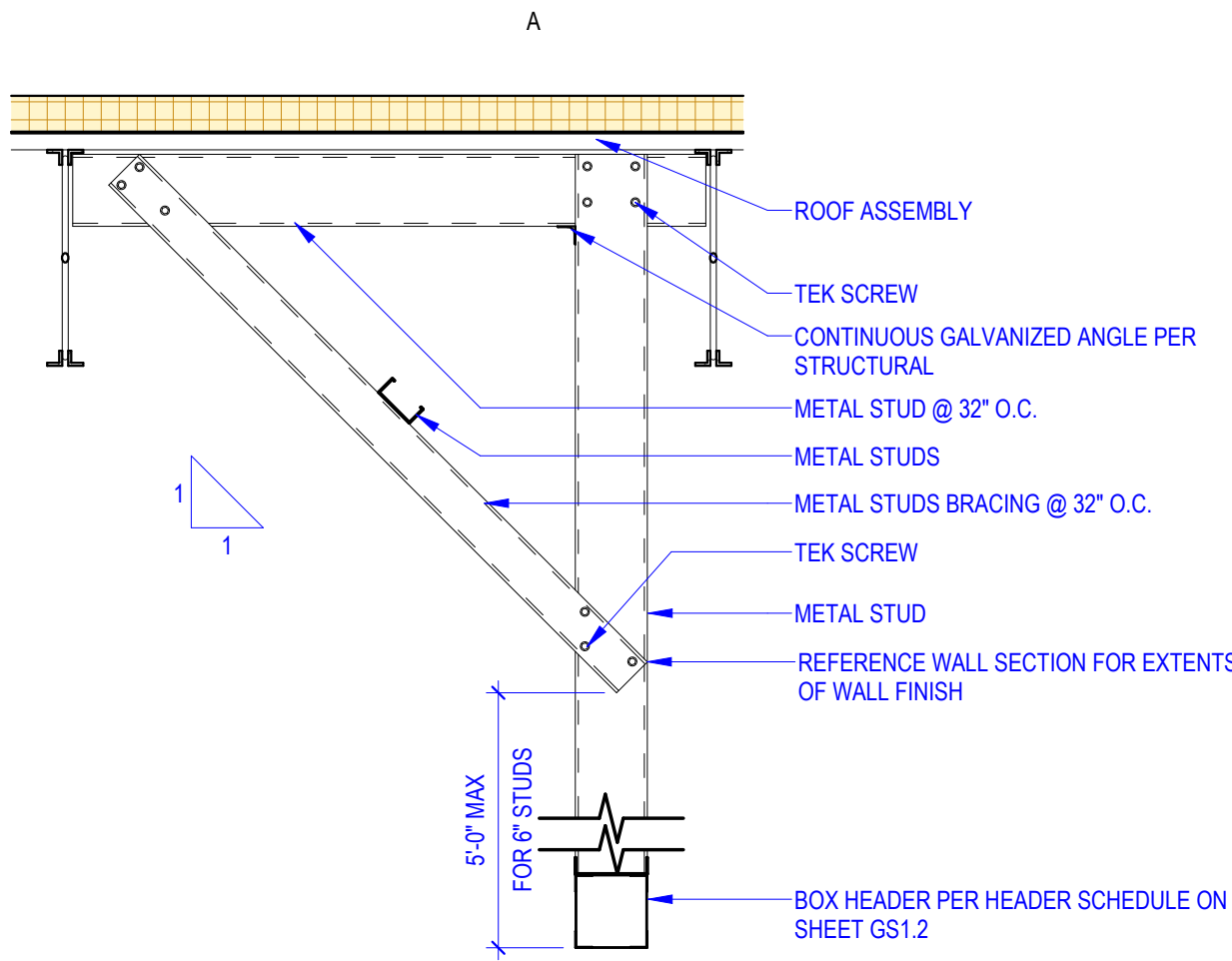
A1 BULKHEAD ATTACHMENT 3/4" = 1'-0"
