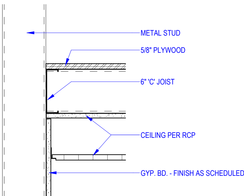
B3 CEILING JOIST AT ATTACHMENT 1 1/2" = 1'-0"
