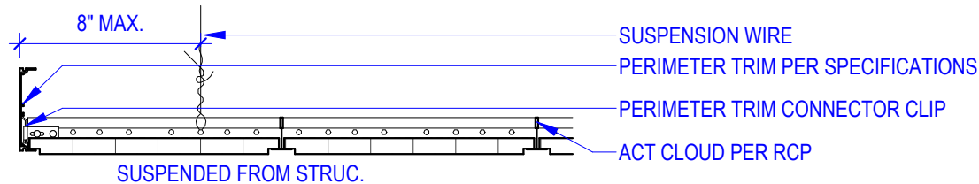
A1 BULKHEAD ATTACHMENT 3/4" = 1'-0"
