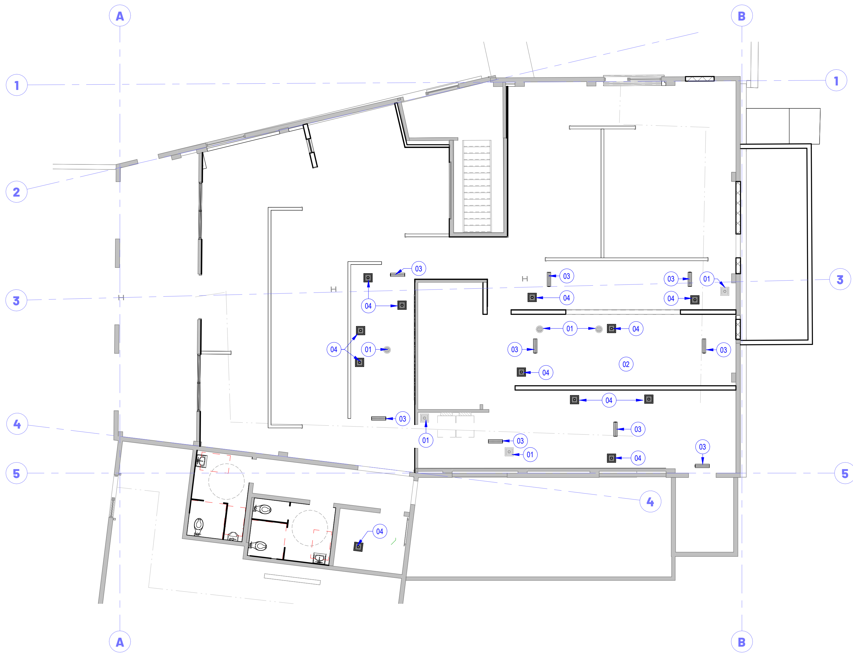
B SLAB PLAN 1/8" = 1'-0" 0' 4' 8' 16'
