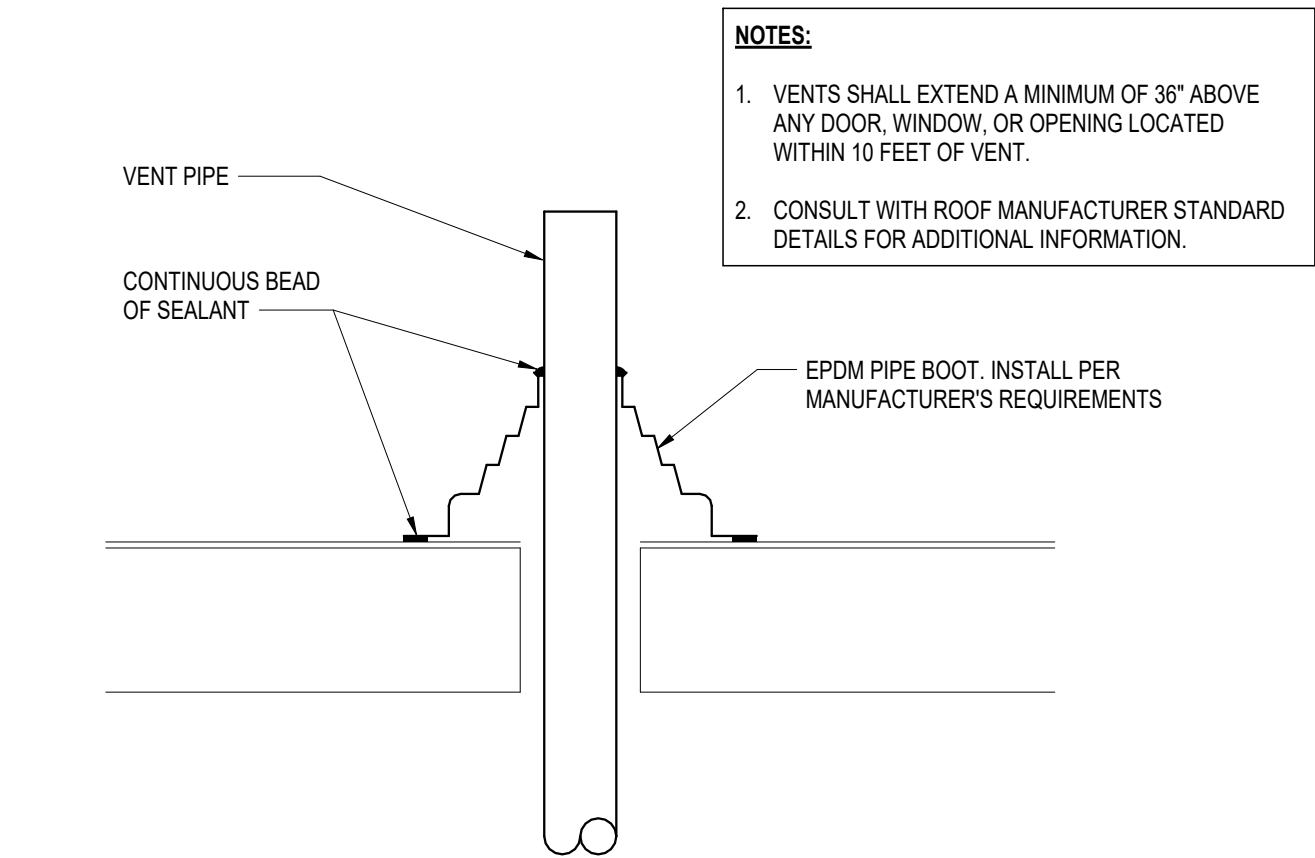
5 VENT THROUGH ROOF NOT TO SCALE
