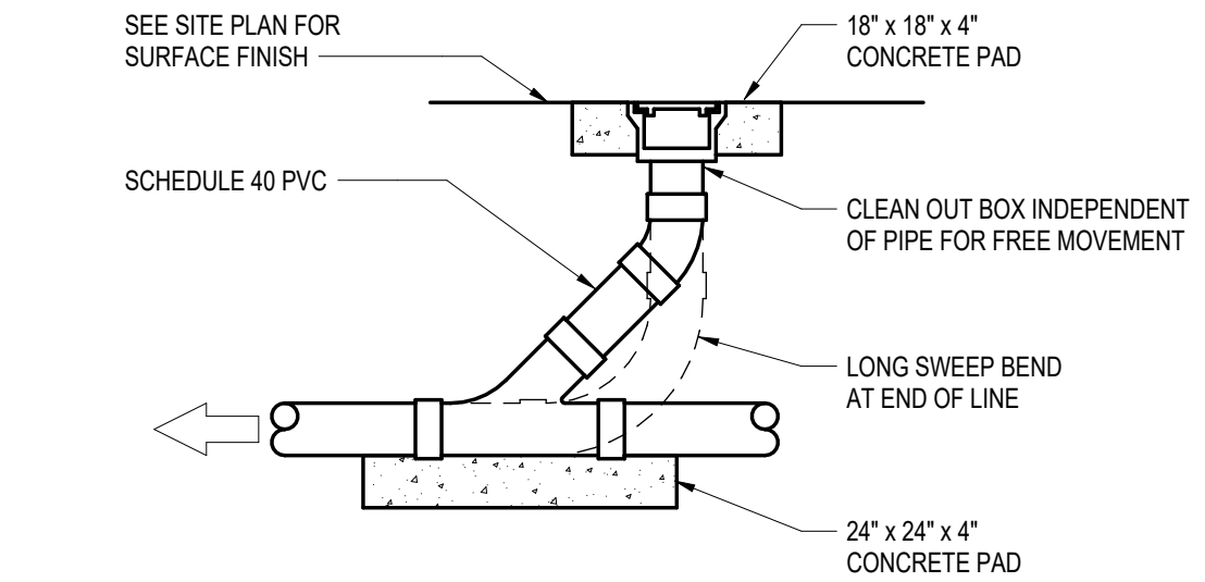
3 CLEANOUT TO GRADE DETAIL NOT TO SCALE
