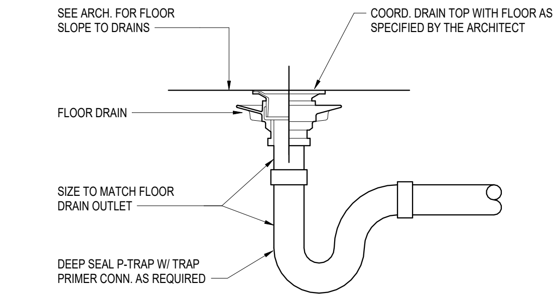
1 FLOOR DRAIN DETAIL NOT TO SCALE
