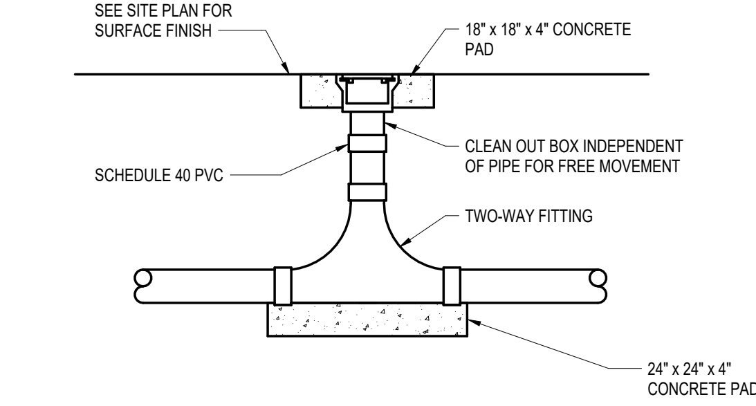
2 2-WAY CLEANOUT TO GRADE DETAIL NOT TO SCALE
