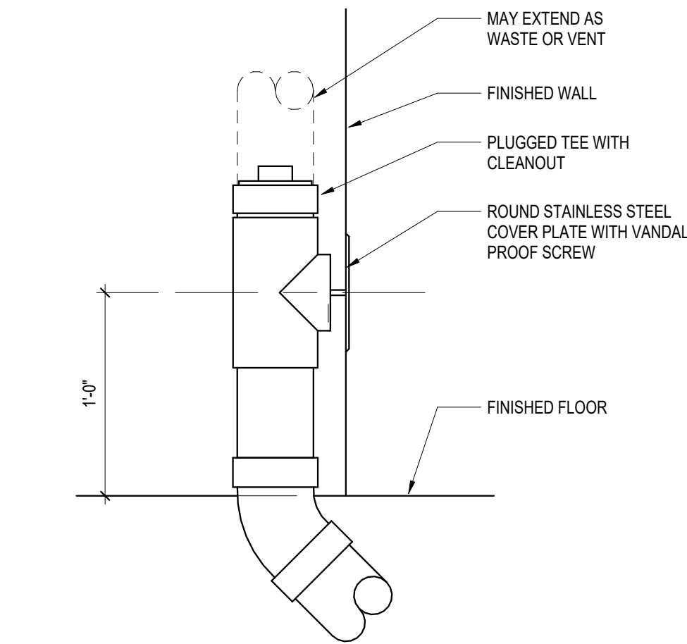
6 WALL CLEANOUT DETAIL NOT TO SCALE
