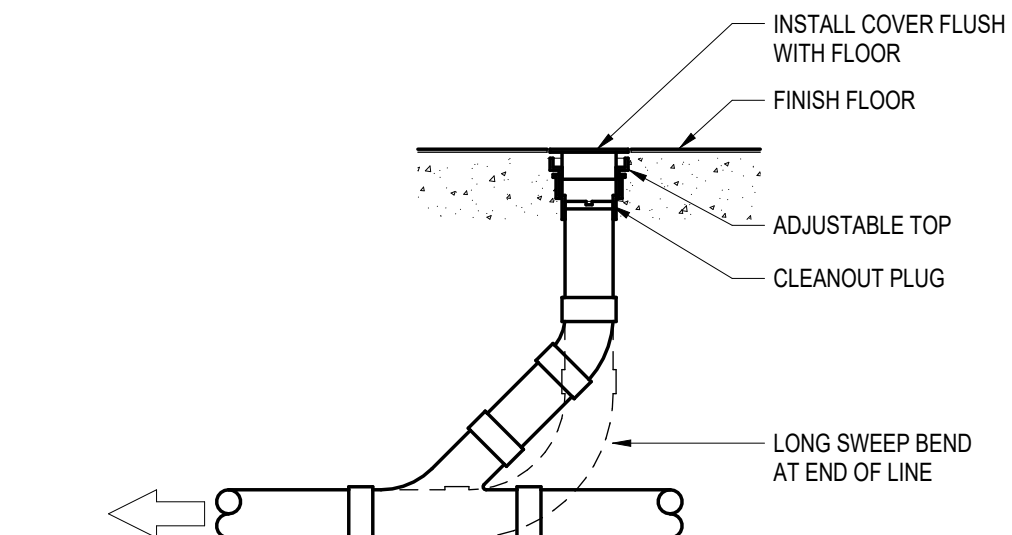
4 FLOOR CLEANOUT DETAIL NOT TO SCALE
