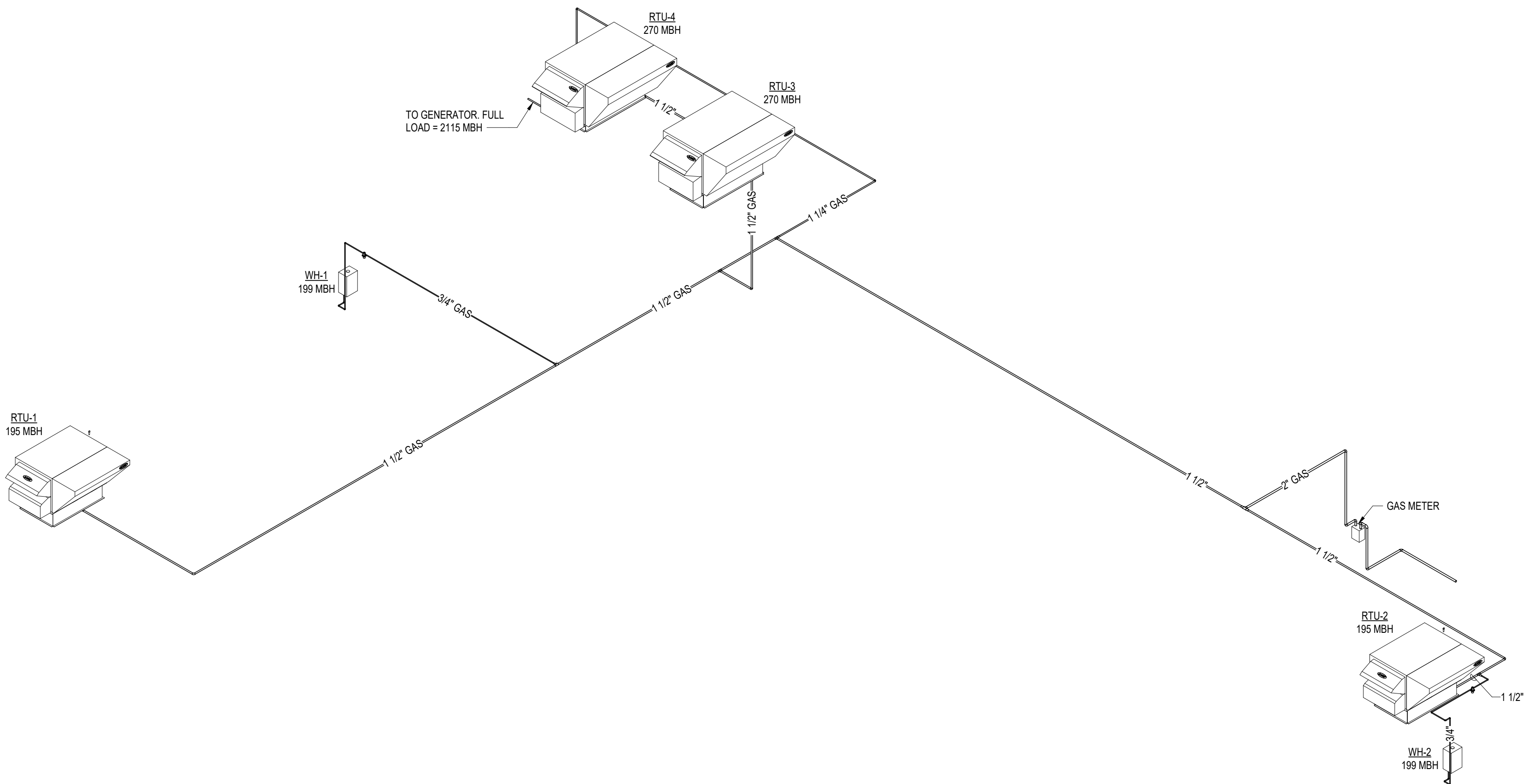
1 GAS RISER DIAGRAM
