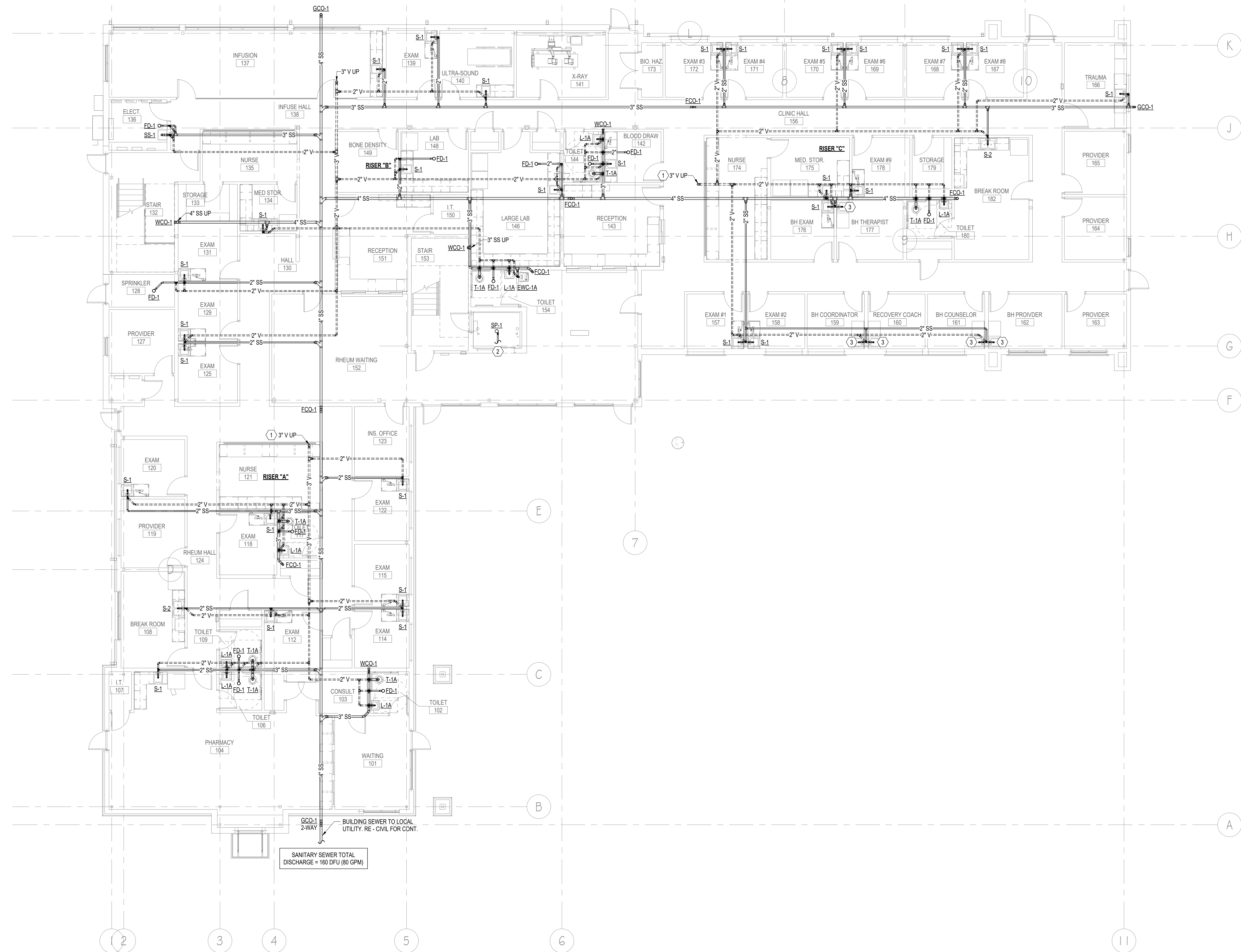
1 1ST FLOOR DWV PLAN 1/8" = 1'-0" RE: 1/M501
