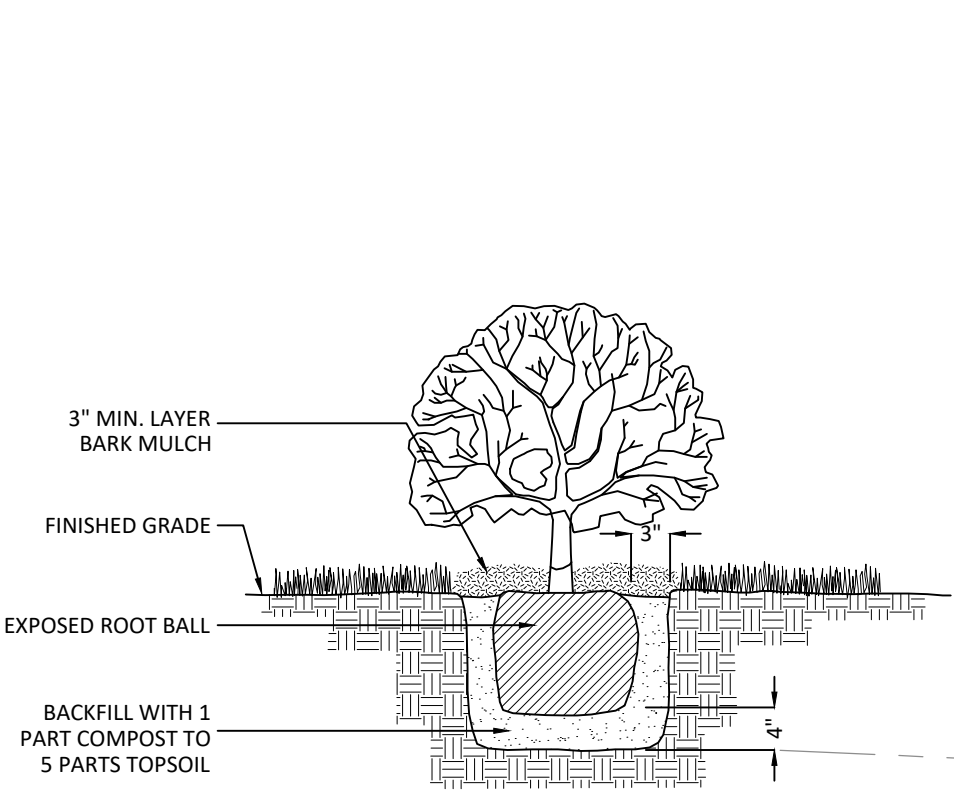
DETAIL - SHRUB PLANTING SCALE - NTS
