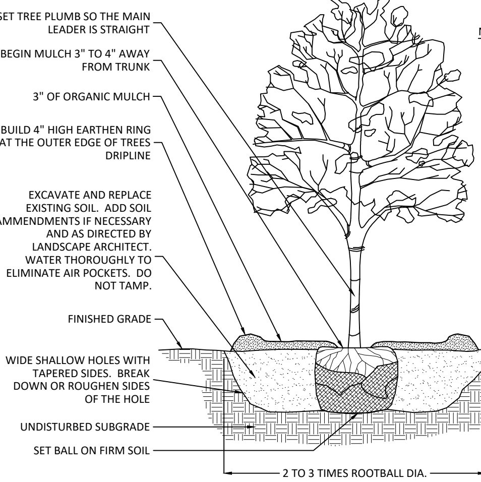
DETAIL - TREE PLANTING SCALE - NTS
