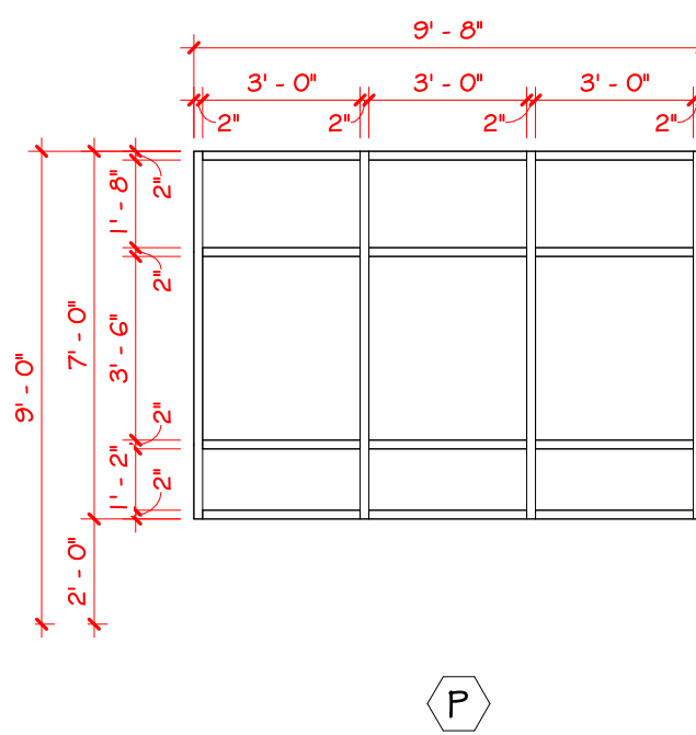
DARK BRONZE ALUMINUM STOREFRONT 1" INSULATED GLAZING W/ LOW-E 70% TINTED GLAZING T = TEMPER
