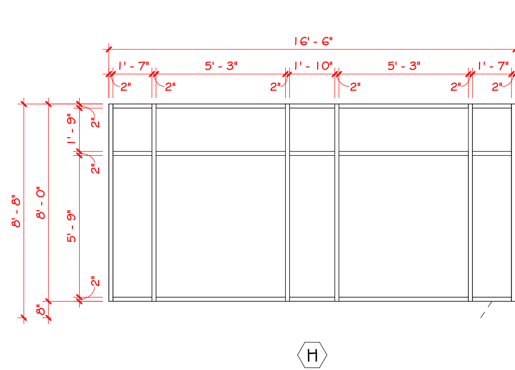
DARK BRONZE ALUMINUM STOREFRONT 1" INSULATED GLAZING W/ LOW-E 70% TINTED GLAZING T = TEMPER
