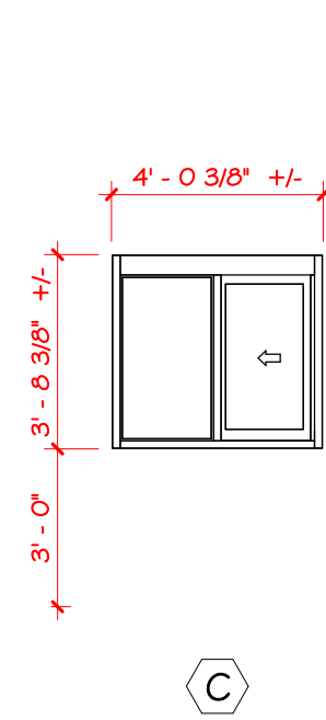
TRANSACTION WINDOW QUIKSERV SC-4844-9190-BL LEFT HAND SLIDE DARK BRONZE
