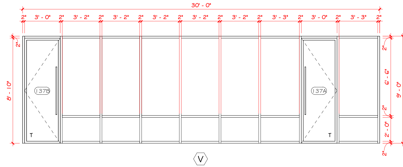
DIRTT MODULAR GLASS WALL SYSTEM CLEAR - SINGLE-PANE GLAZING T = TEMPER
