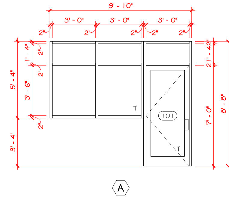
DARK BRONZE ALUMINUM STOREFRONT 1" INSULATED GLAZING W/ LOW-E 70% TINTED GLAZING T = TEMPER
