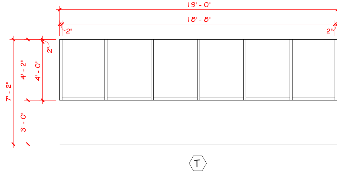
DIRTT MODULAR GLASS WALL SYSTEM DARK BRONZE CLEAR - SINGLE-PANE GLAZING T = TEMPER
