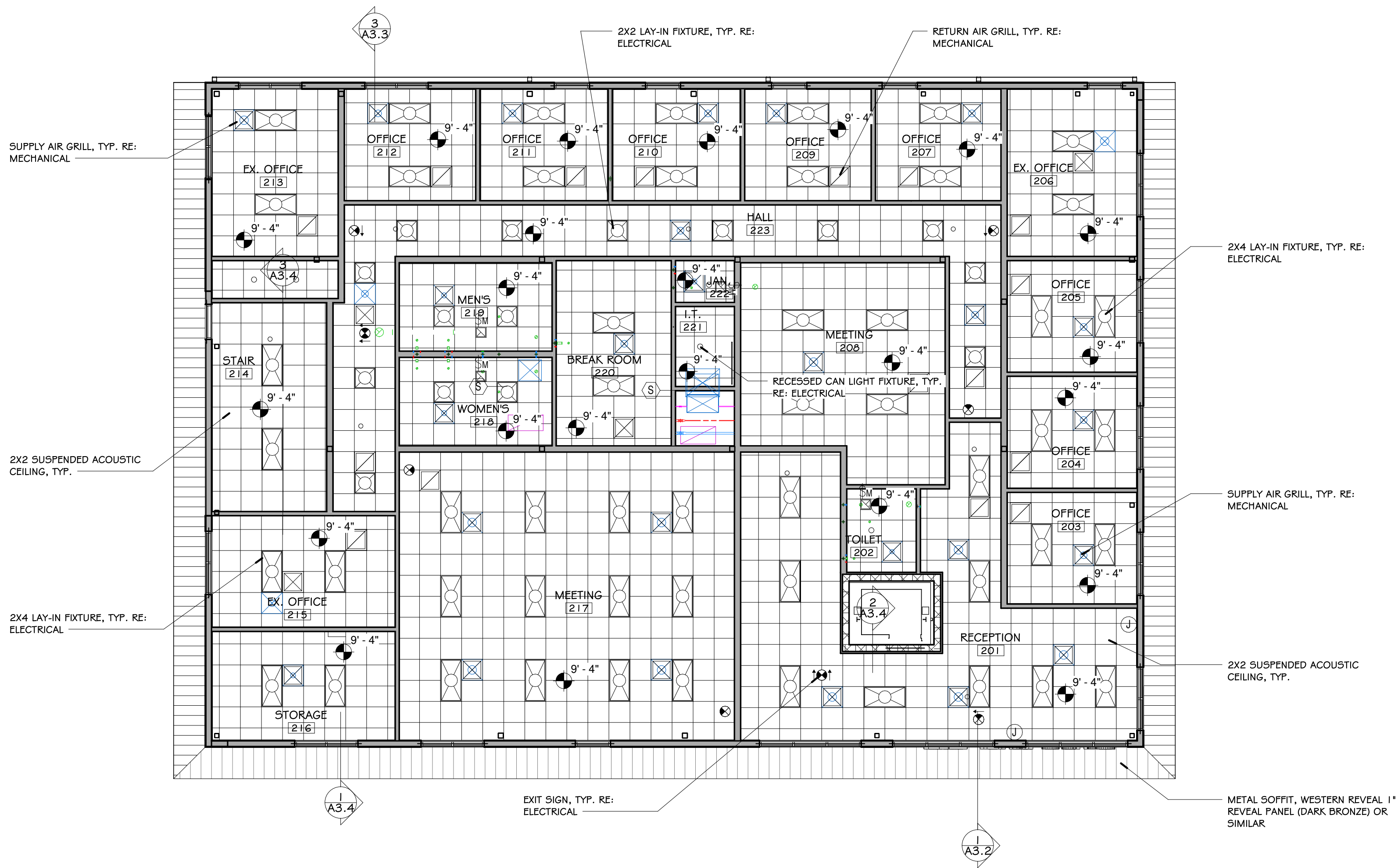
1 2ND FLOOR CEILING PLAN SCALE = 1/8" = 1'-0"
