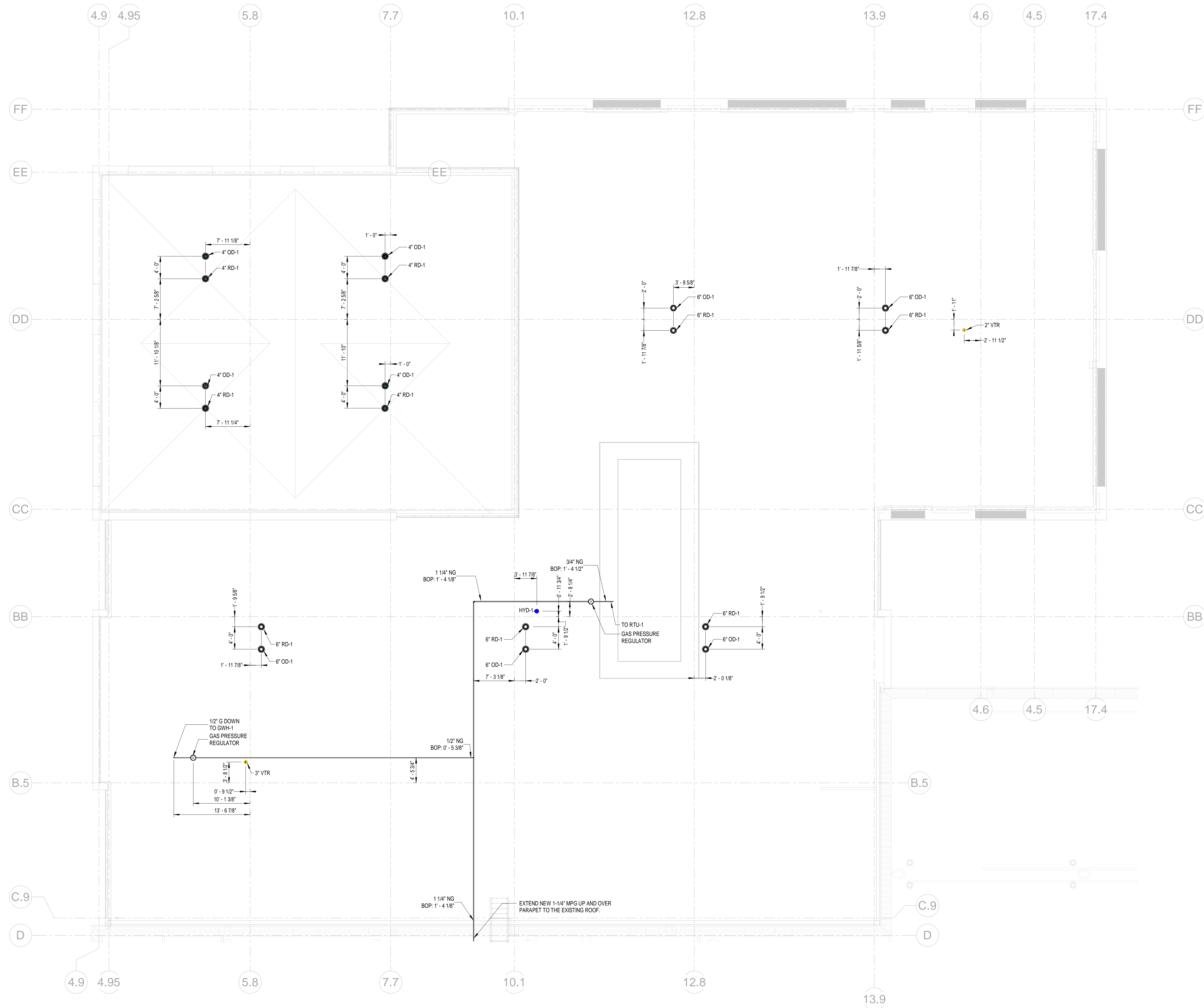
1 PLUMBING ROOF LEVEL SHOP DRAWING 1/8" = 1'-0"
