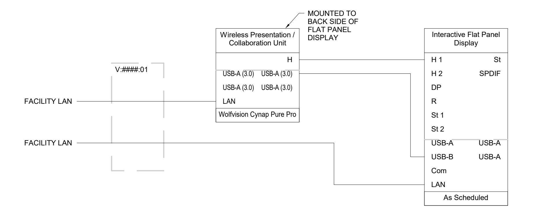
4 SIGNAL FLOW DIAGRAM FOR OPEN GATHERING SPACES GENERAL CORRIDORS, SITTING AREAS, LIBRARY, BREAK ROOMS, WELLNESS STUDIO 3318, STUDENT RECREATION 3310, & OFFICE 4142
