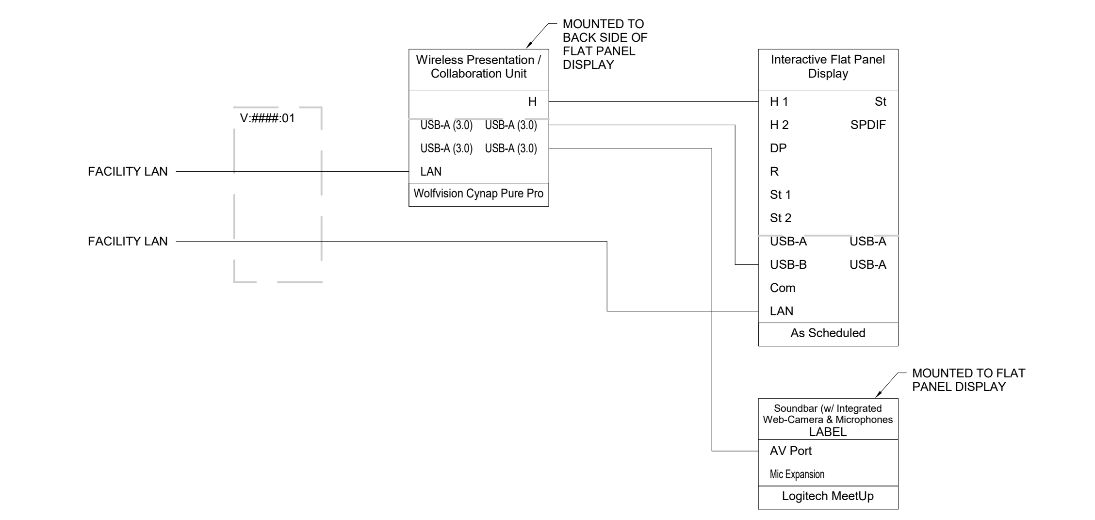
5 SIGNAL FLOW DIAGRAM FOR STUDY SPACES STUDY ROOMS
