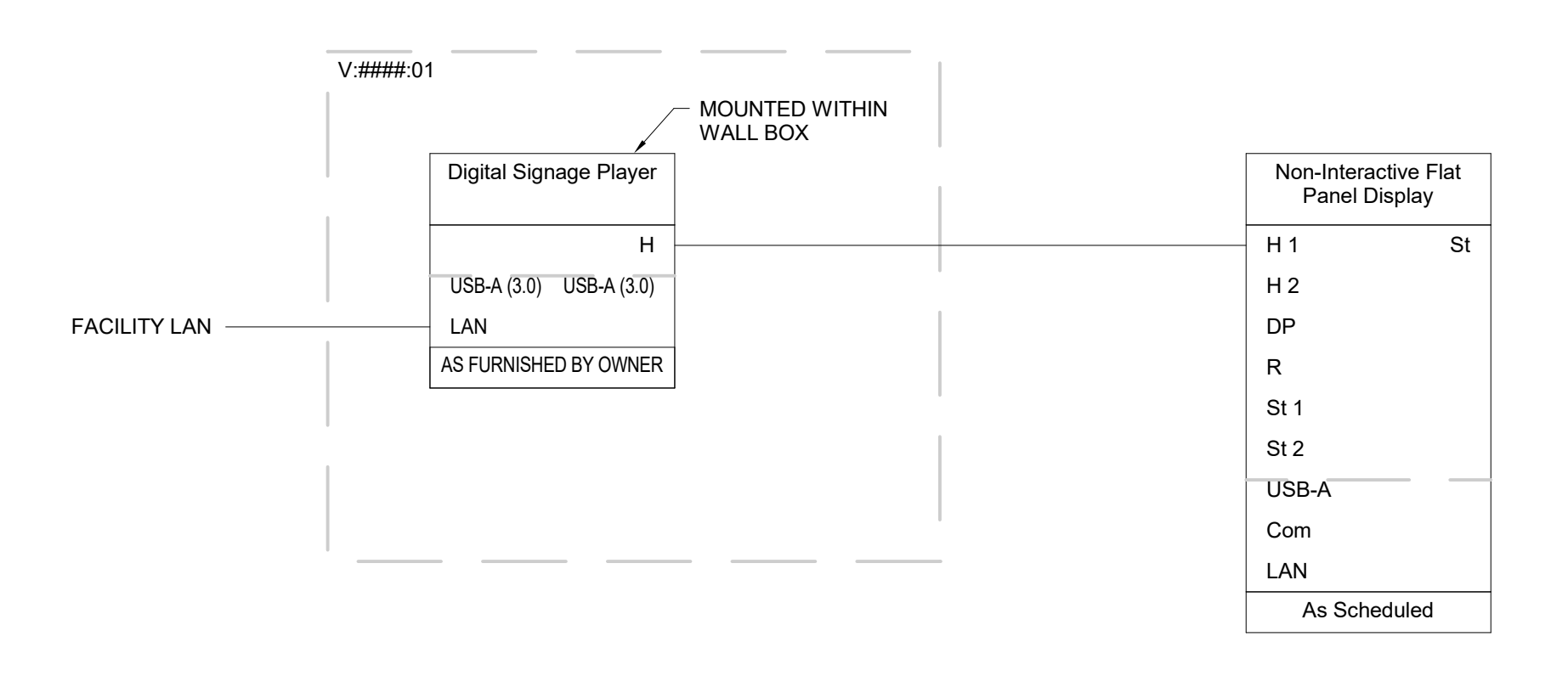
1 SIGNAL FLOW DIAGRAM FOR NON-INTERACTIVE DIGITAL SIGNAGE CAFE DINING, GAME ROOMS, PUBLIC LOBBIES, STUDENT LOUNGES, CLINIC WAITING, GYMNASIUM
