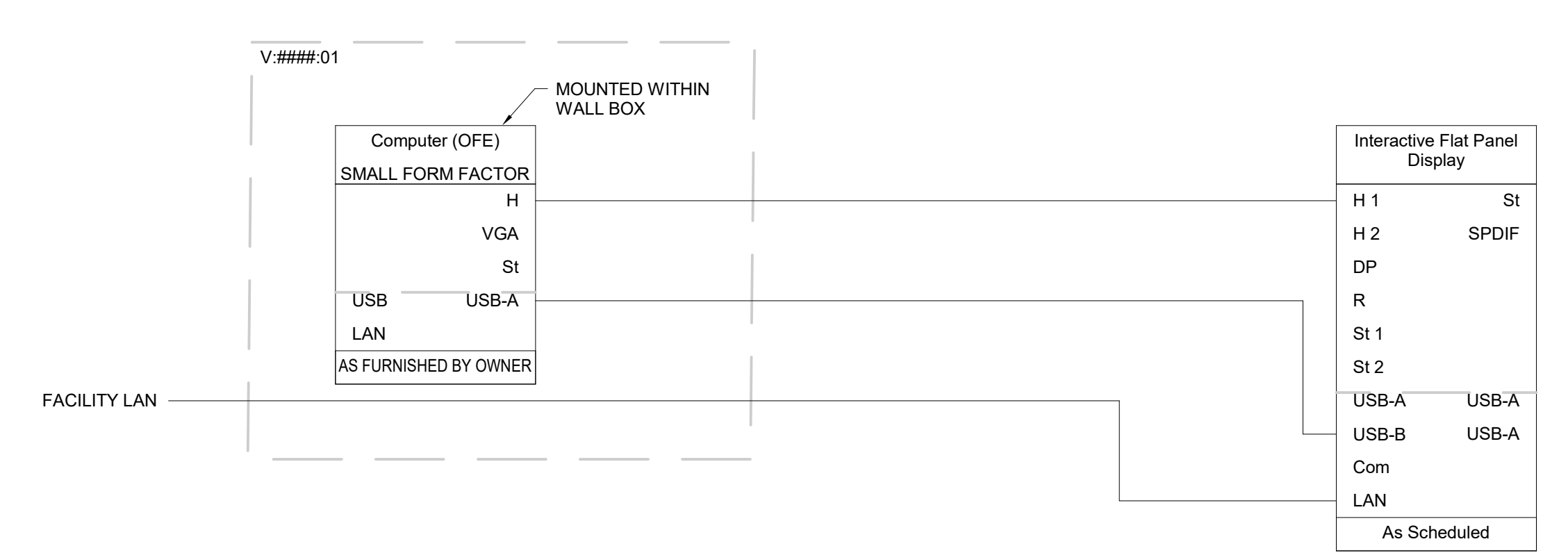
2 SIGNAL FLOW DIAGRAM FOR SECURITY SECURITY OFFICE 1528
