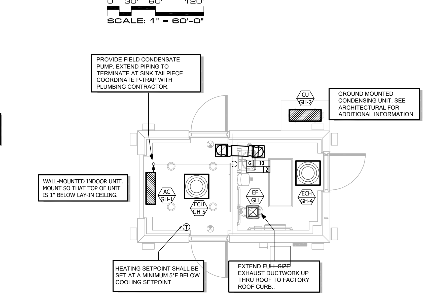
OVERALL HVAC PLAN
