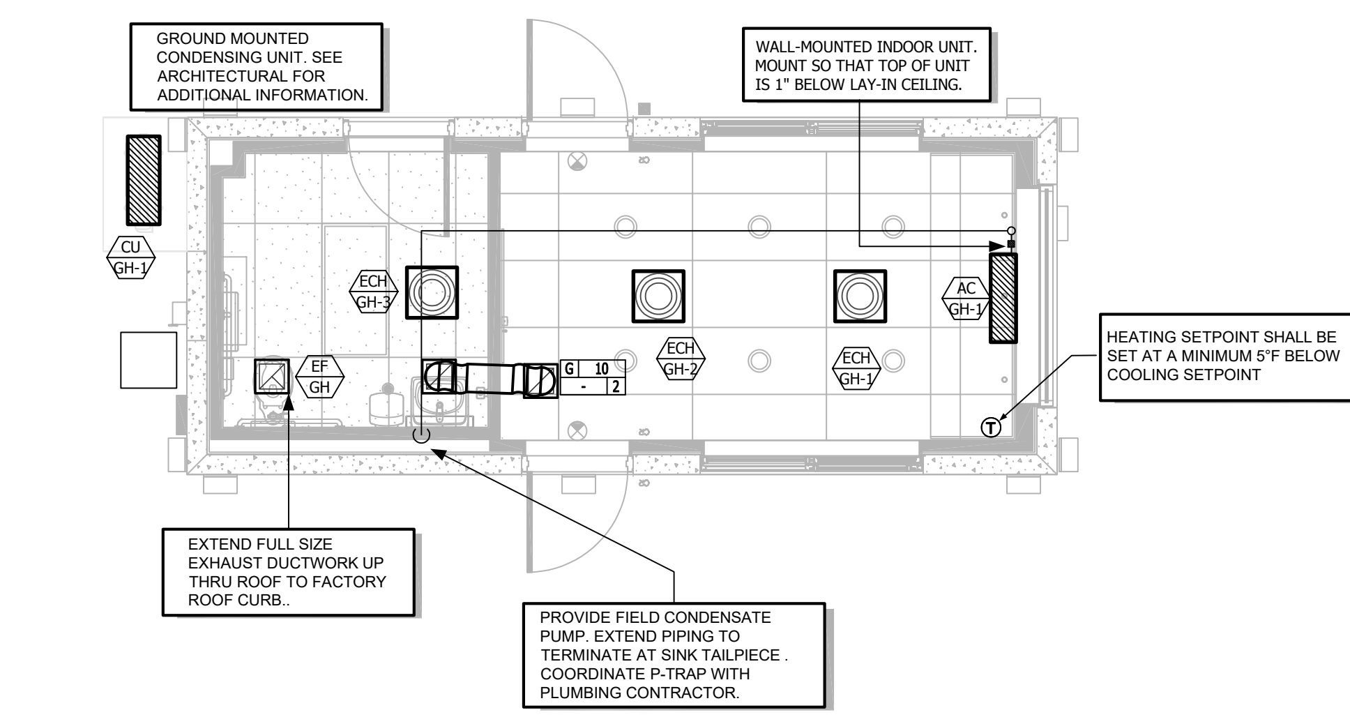
OVERALL HVAC PLAN
