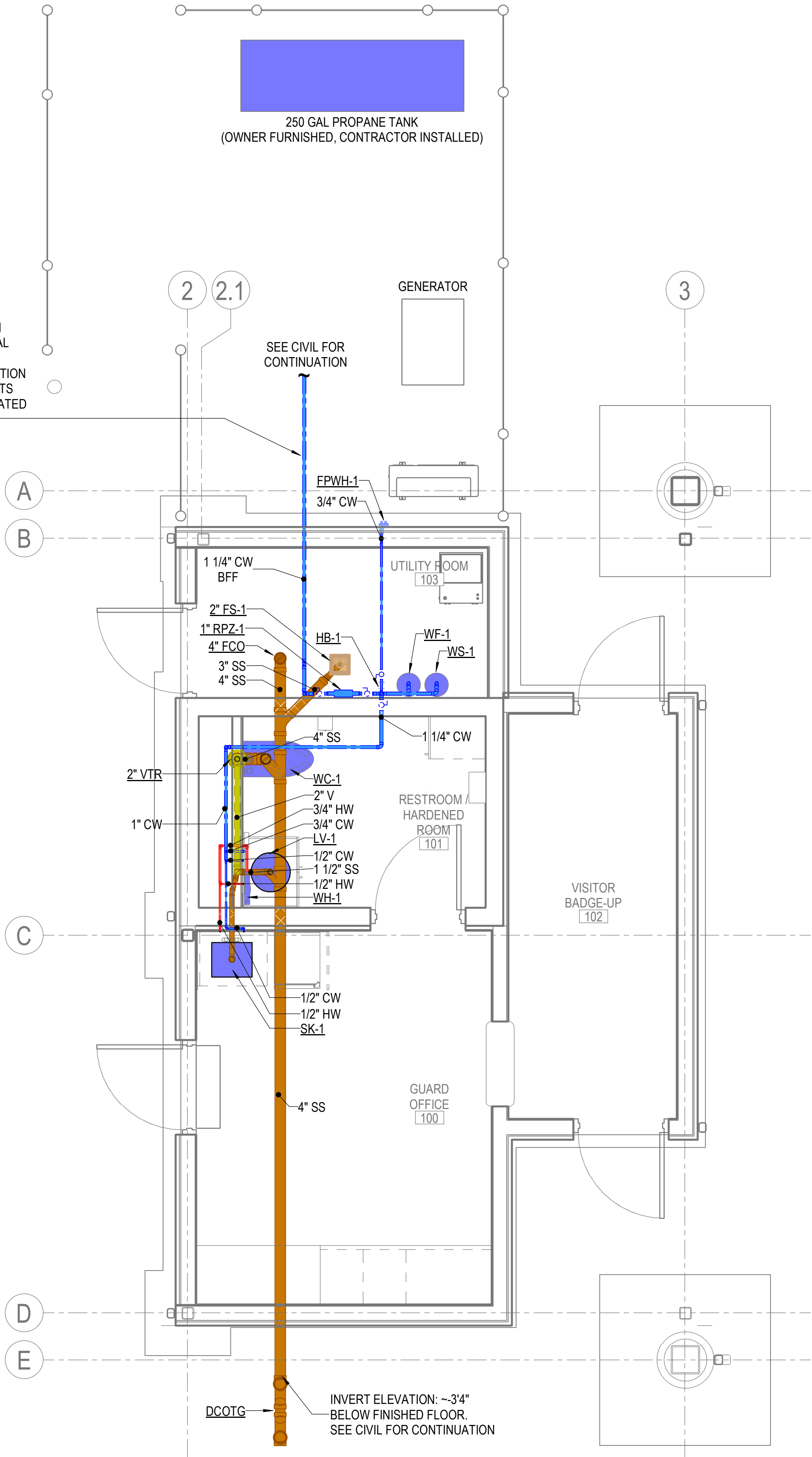
1 OVERALL PLUMBING PLAN 3/8" = 1'-0"
