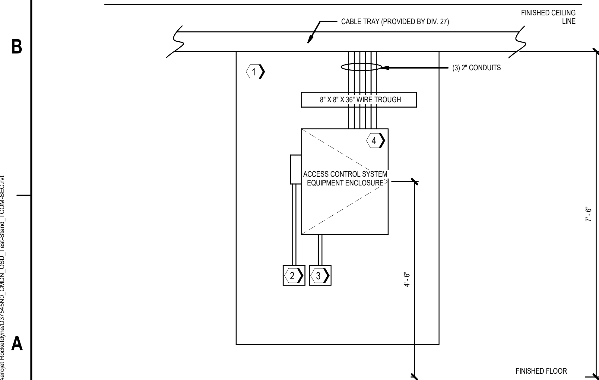
A1 TYPICAL ACP ENCLOSURE ELEVATION SCALE NOT TO SCALE
