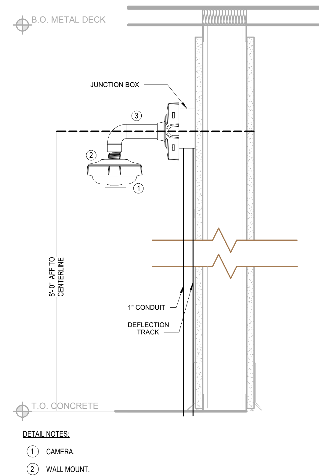
C4 WALL MOUNTED CAMERA SCALE NTS
