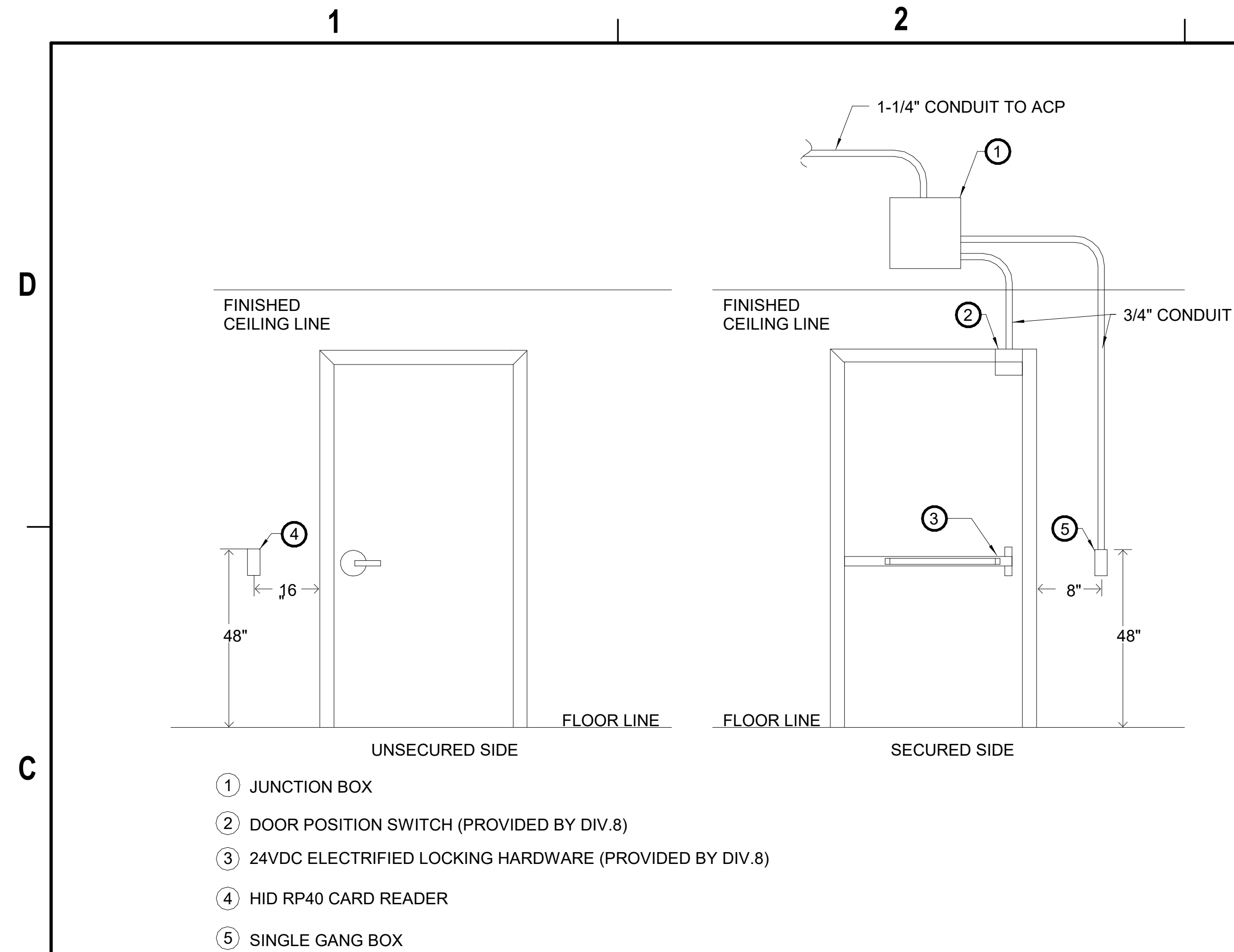
C1 SINGLE DOOR WITH KEYPAD SCALE NTS
