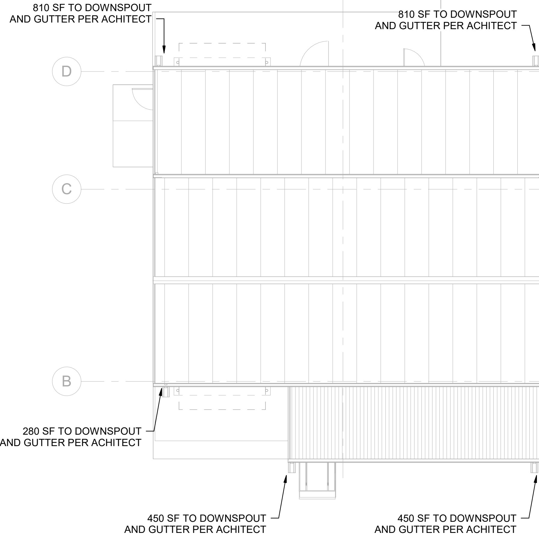
A3 ROOF PLAN SCALE 1/8" = 1'-0"
