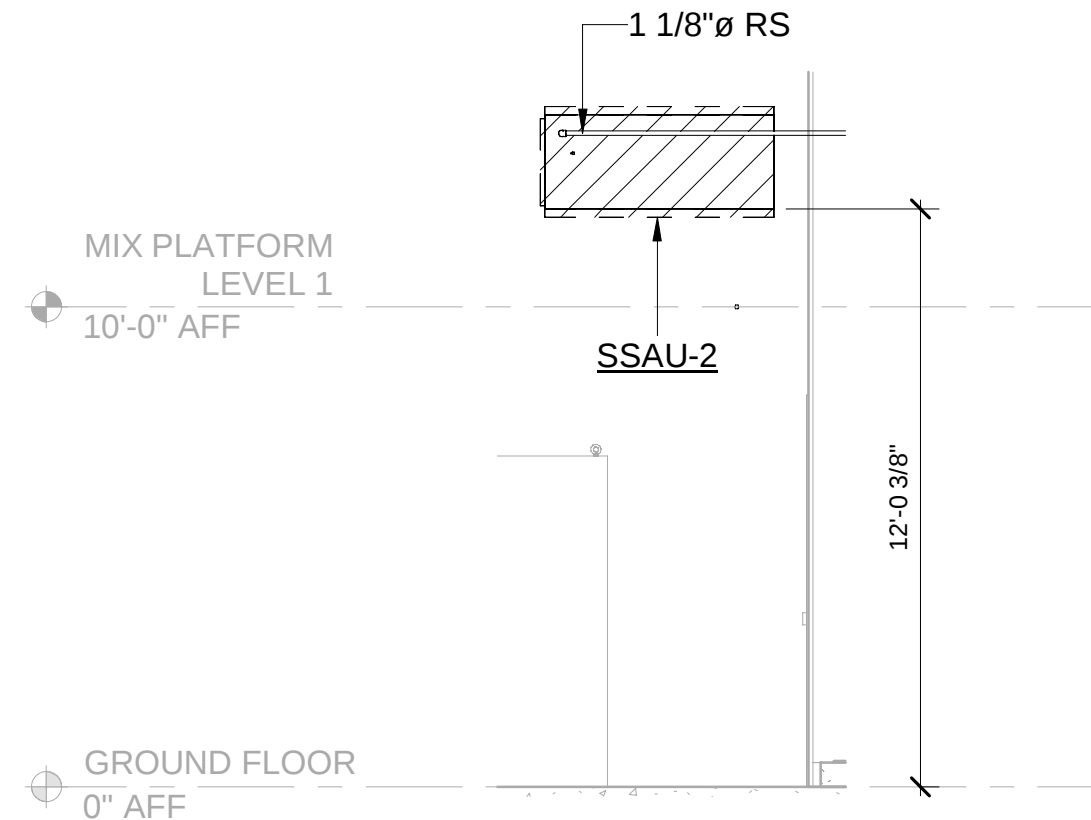
3 SSAU-2 SECTION VIEW SCALE 1/4" = 1'-0"
