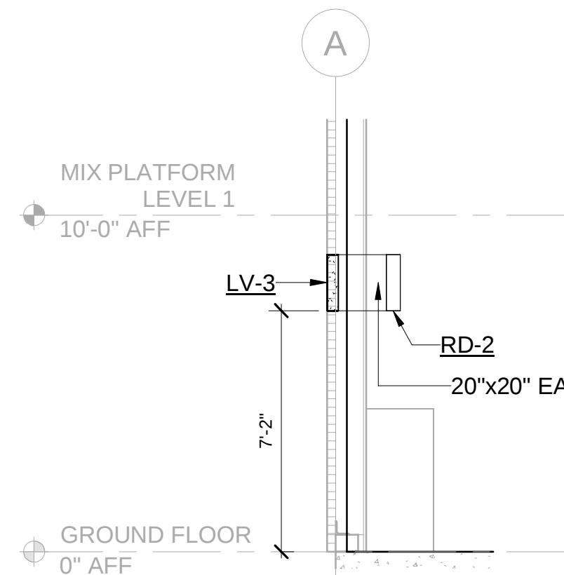
2 LOUVER SECTION VIEW SCALE 1/4" = 1'-0"
