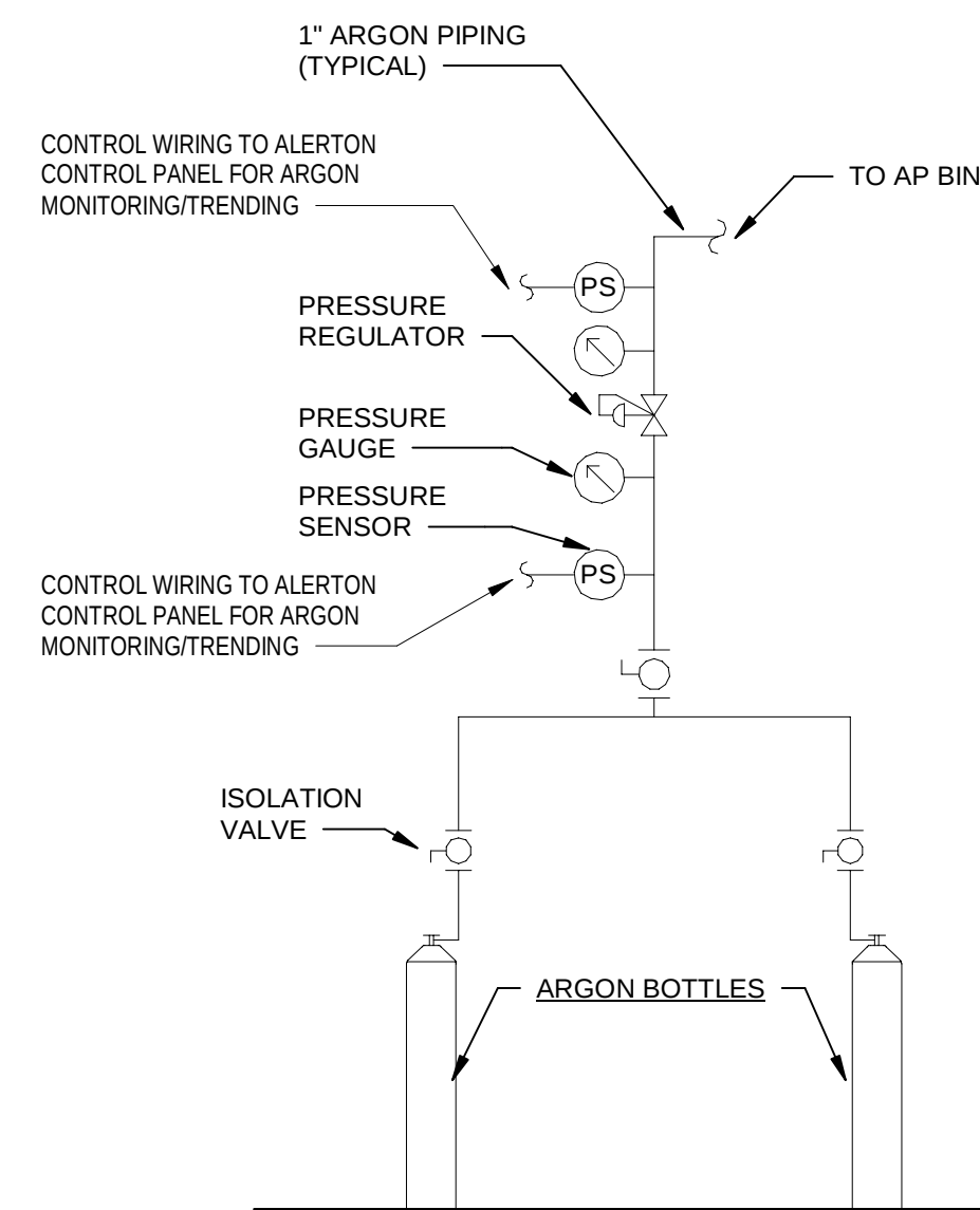
1 ARGON SCHEMATIC DIAGRAM SCALE NTS
