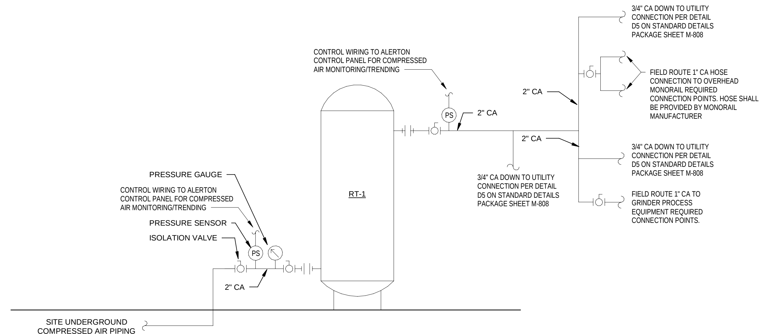
2 COMPRESSED AIR SCHEMATIC DIAGRAM SCALE NTS
