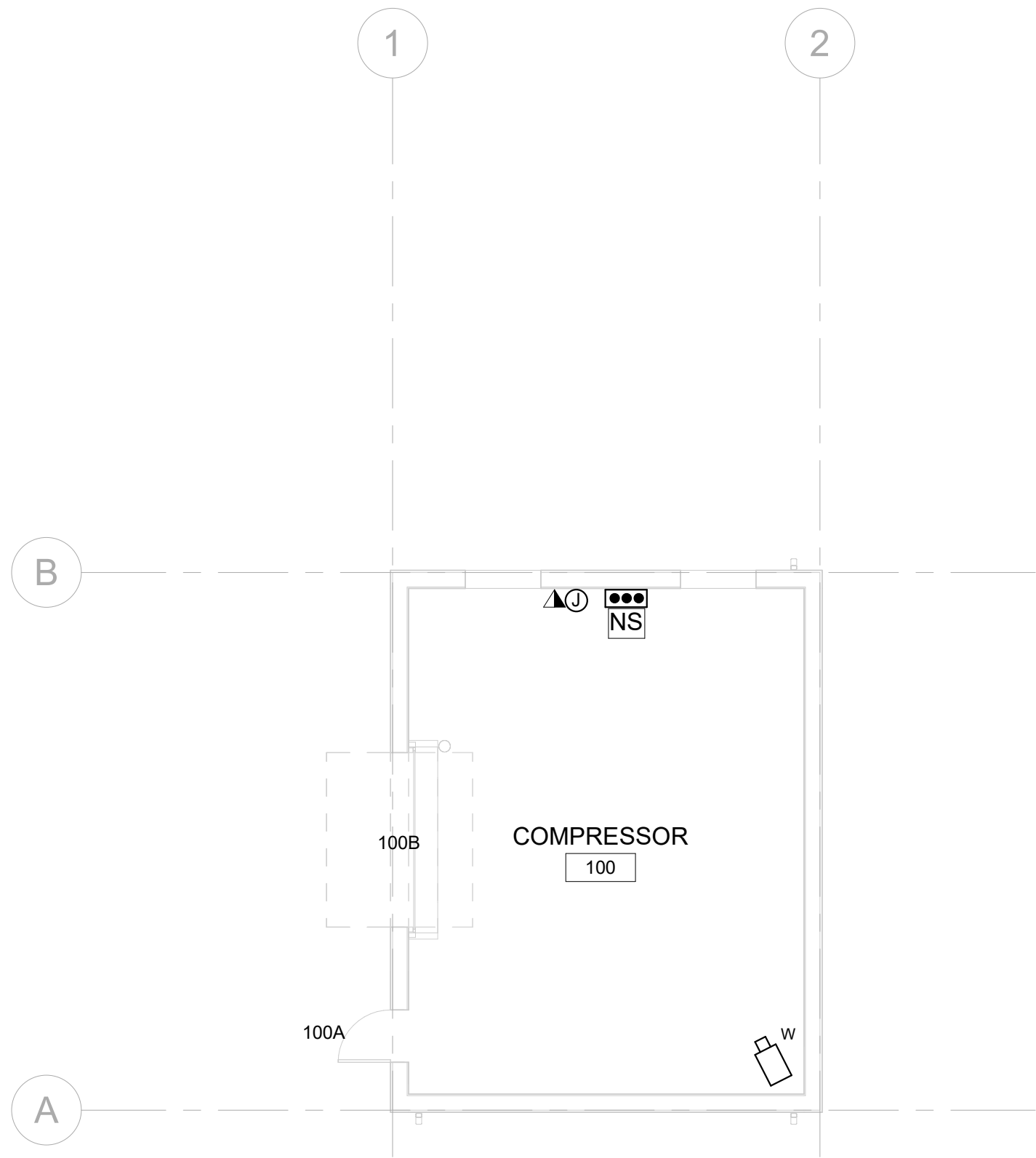
A1 GROUND FLOOR ELECTRONIC SECURITY SYSTEM PLAN SCALE 1/8" = 1'-0"
