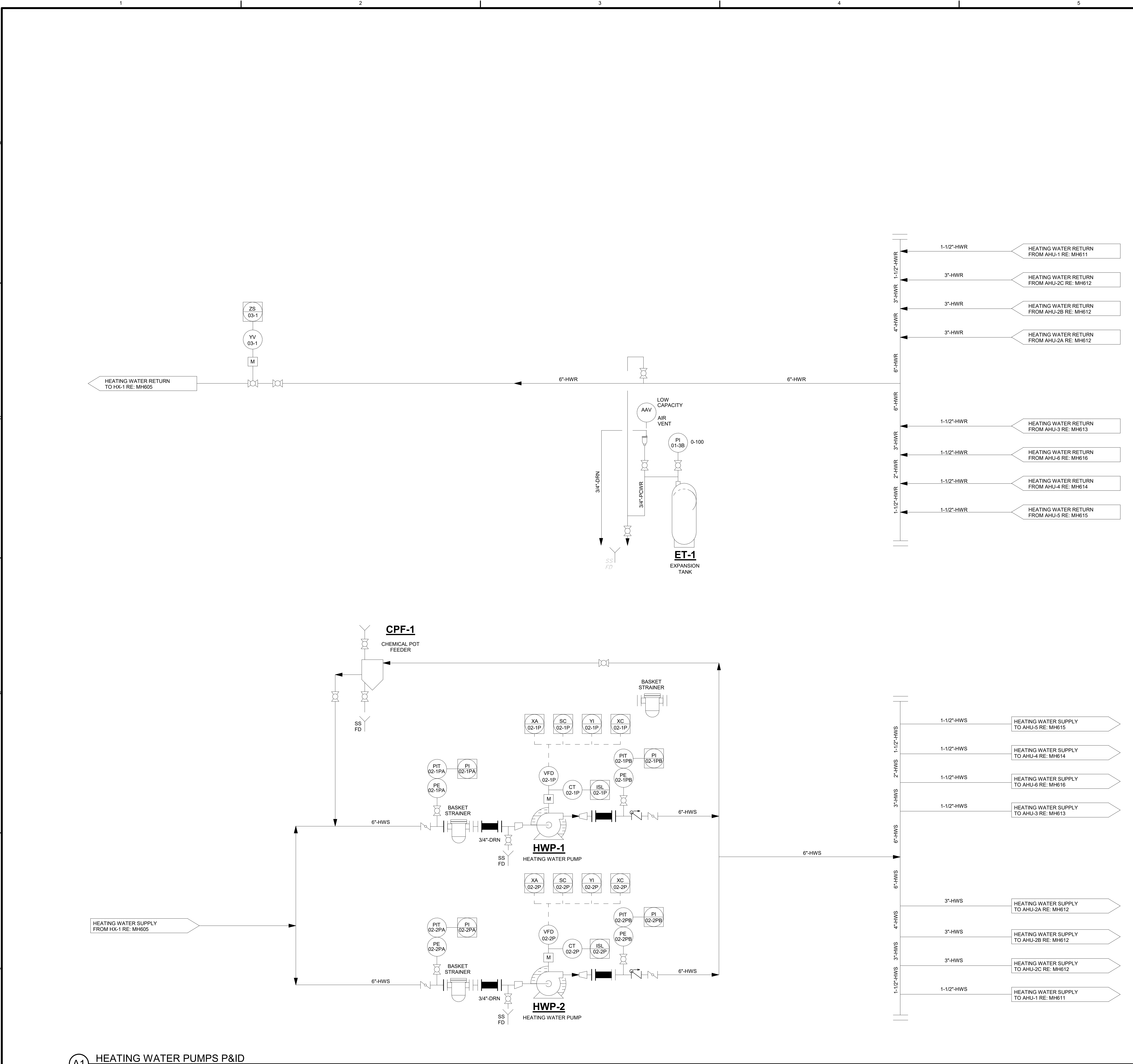
A1 HEATING WATER PUMPS P&ID SCALE: NTS
