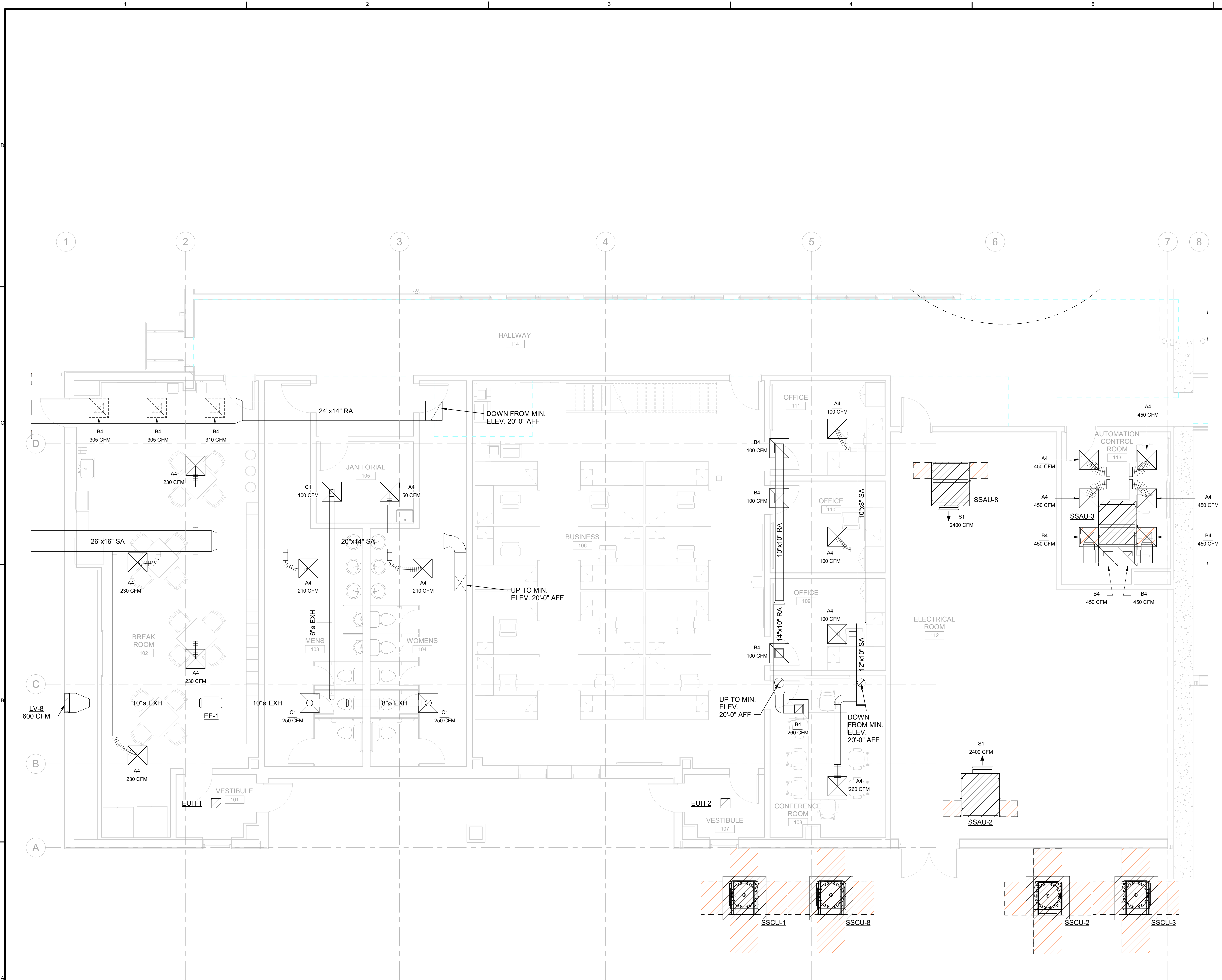
1 ENLARGED HVAC DUCT FLOOR PLAN-OFFICE LEVEL 1 SCALE 1/4" = 1'-0"
