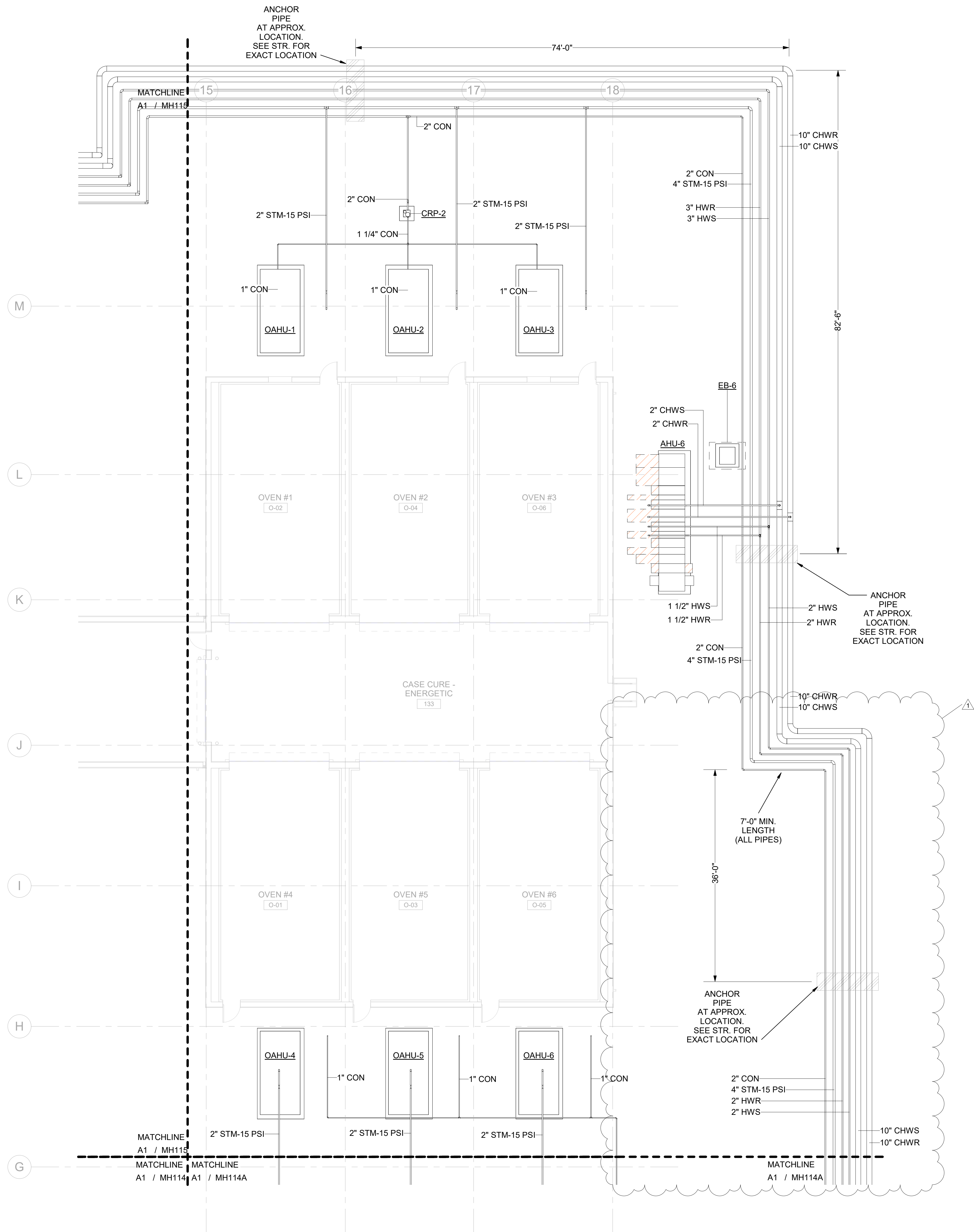
(A1) HVAC PIPING FLOOR PLAN-AREA 'D' EAST SCALE 1/8" = 1'-0"
