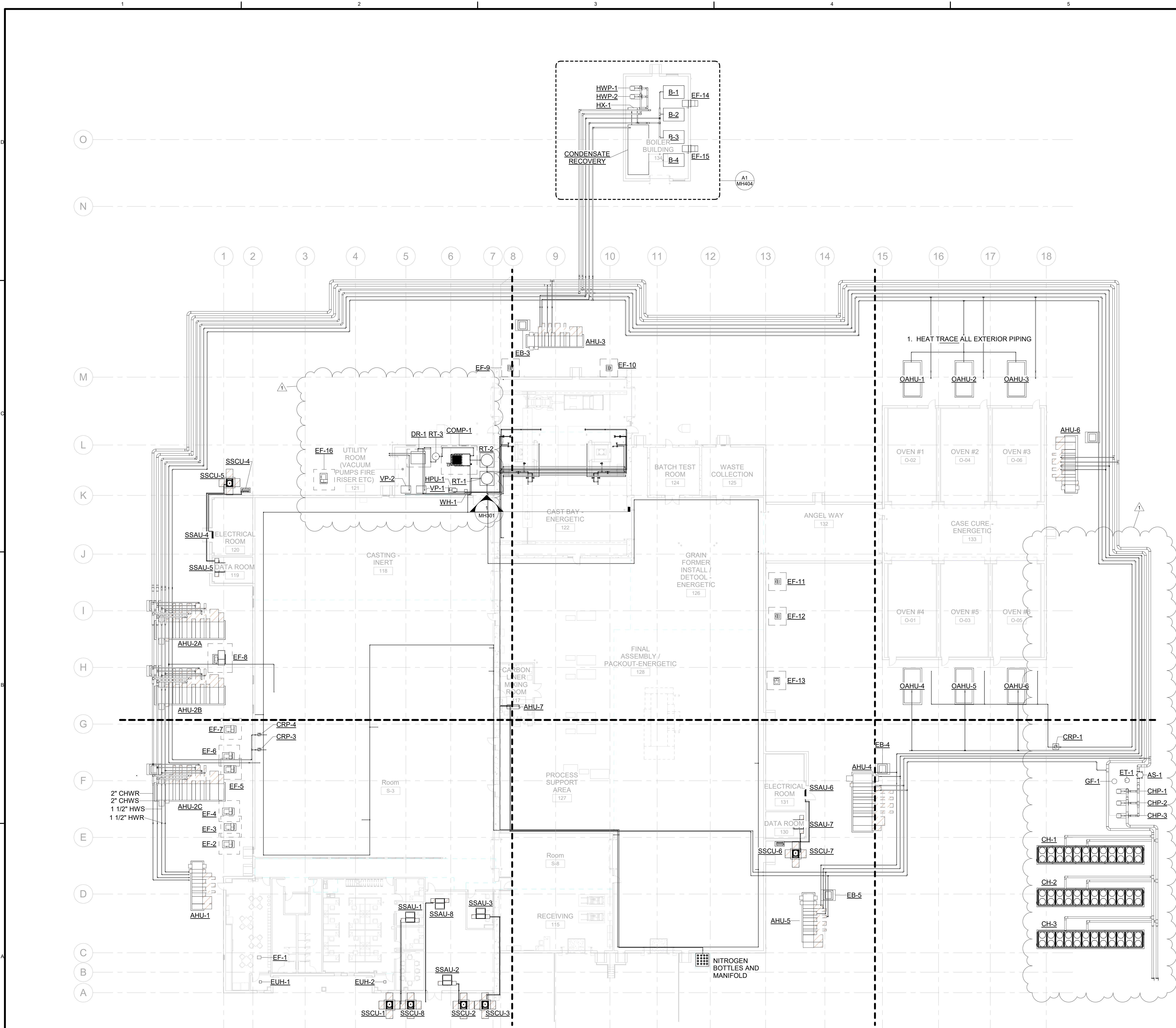
A1 HVAC OVERALL PIPING FLOOR PLAN SCALE 1/16" = 1'-0"
