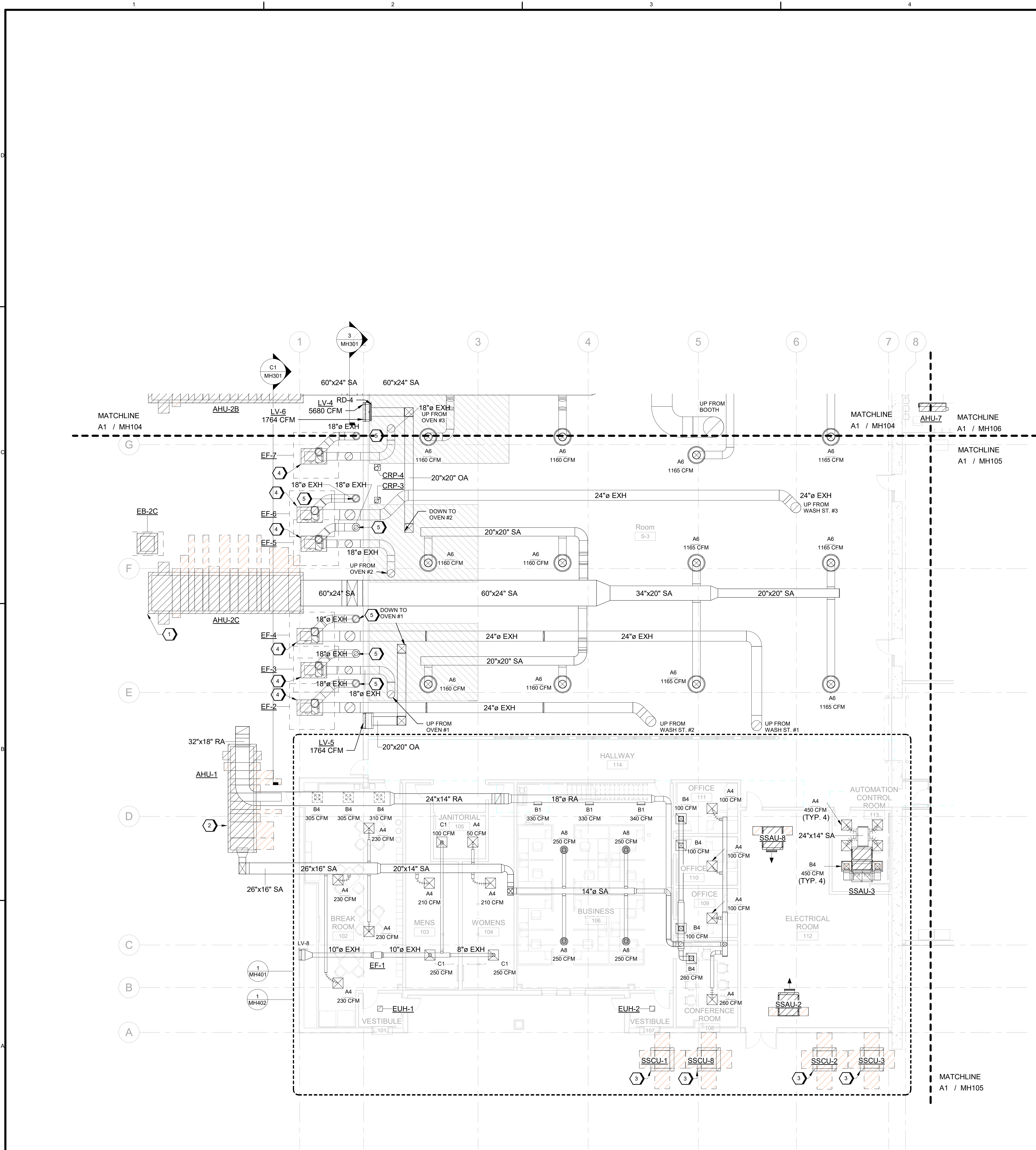
A1 HVAC DUCT FLOOR PLAN-AREA 'A' SCALE 1/8" = 1'-0"
