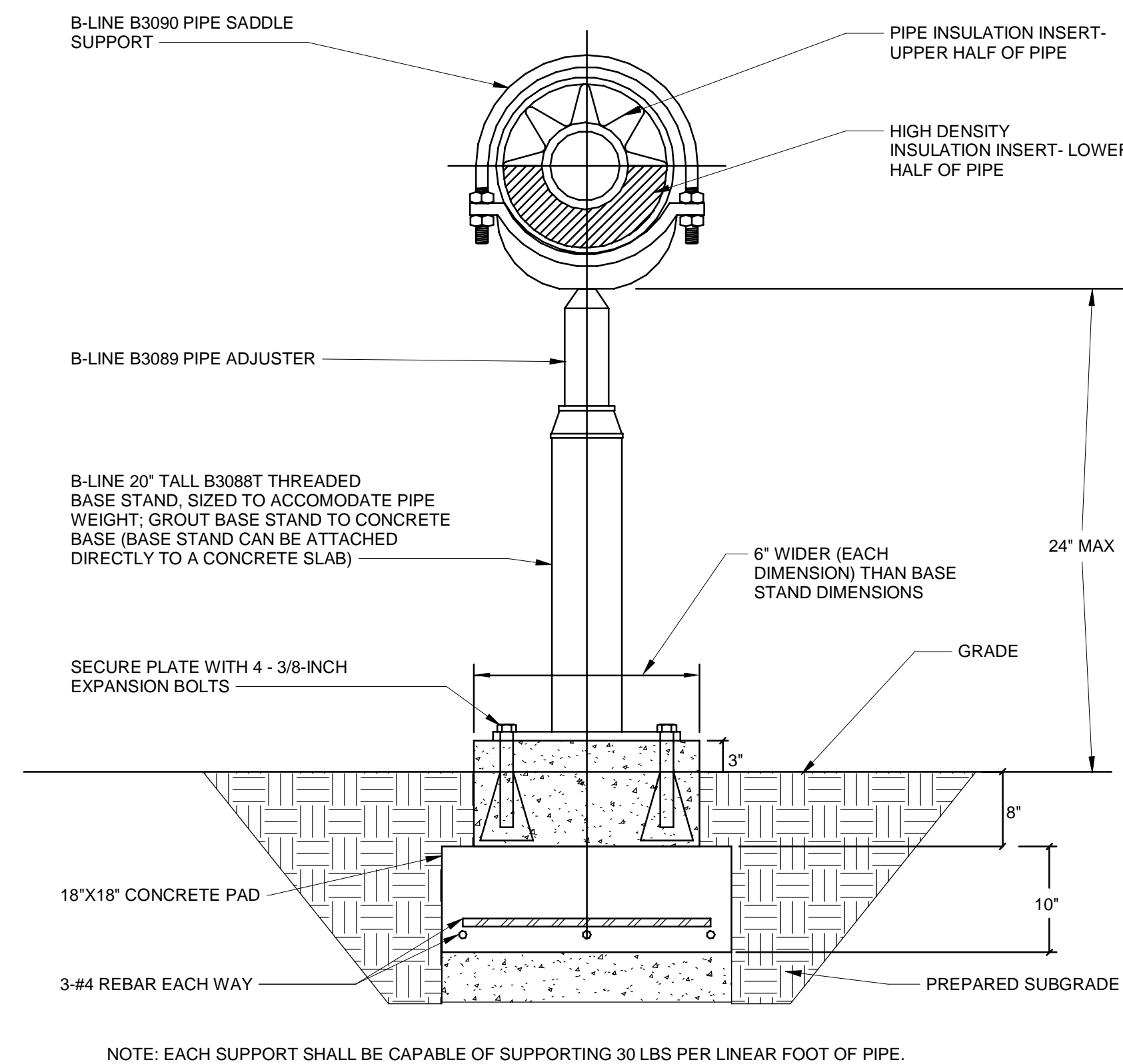
A5 TYPICAL FLOOR/GRADE PIPE SUPPORT DETAIL SCALE NTS
