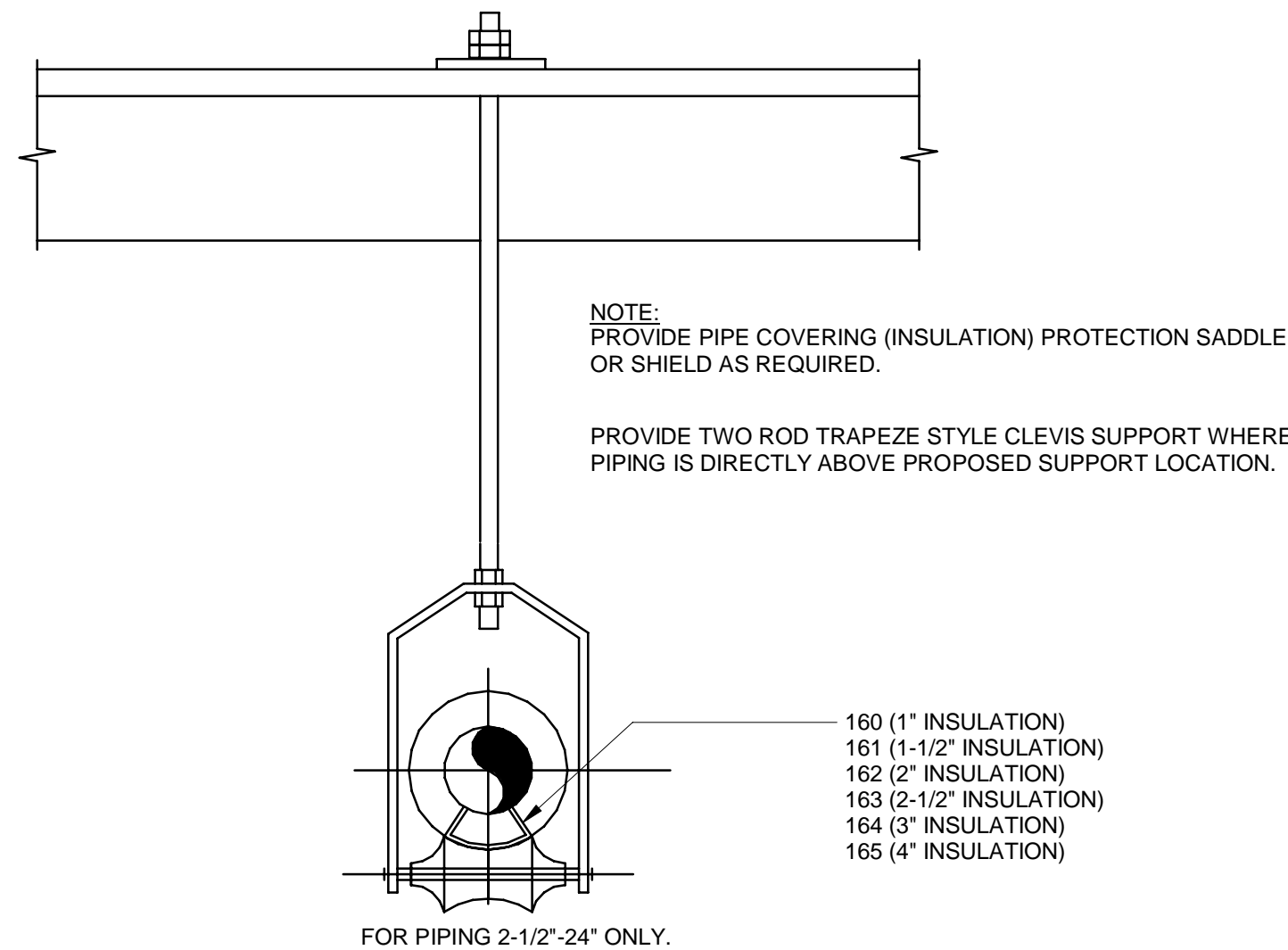
C1 TYPICAL CLEVIS SUPPORT SCALE NTS
