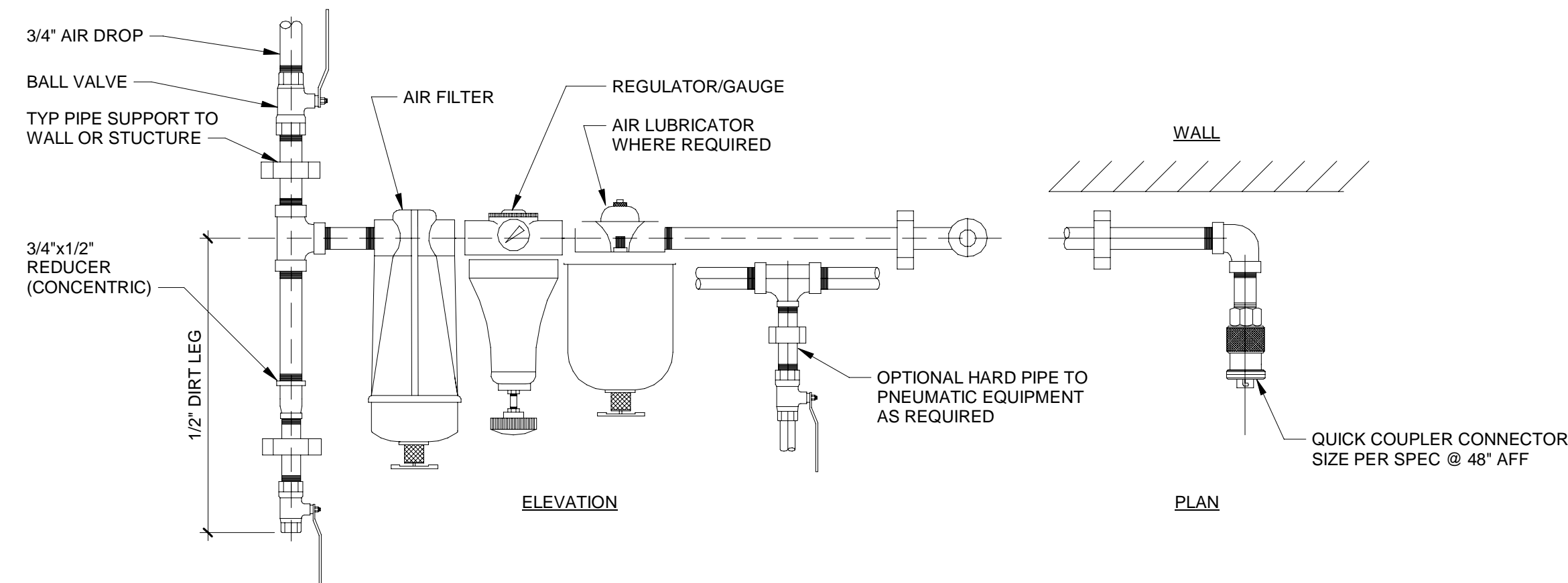
D5 TYP COMPRESSED AIR OUTLET DETAIL SCALE 3/16" = 1'-0"
