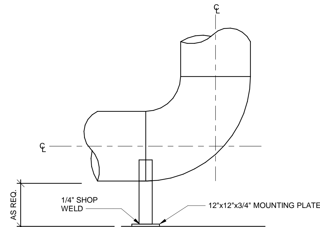
C5 TYPICAL PUMP DISCHARGE ELBOW PIPE SUPPORT DETAIL SCALE NTS
