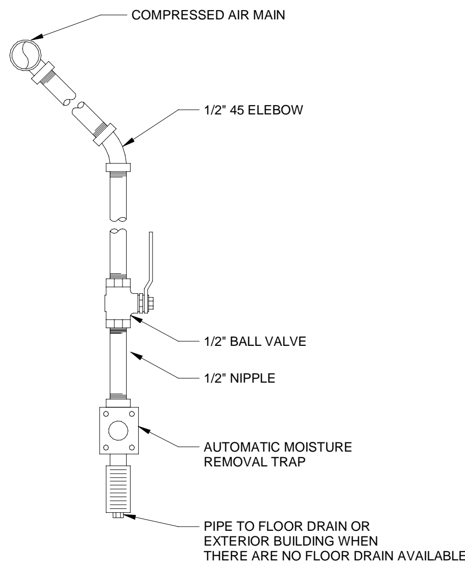
D3 TYP COMPRESSED AIR END OF MAIN DRAIN DETAIL SCALE 3/4" = 1'-0"
