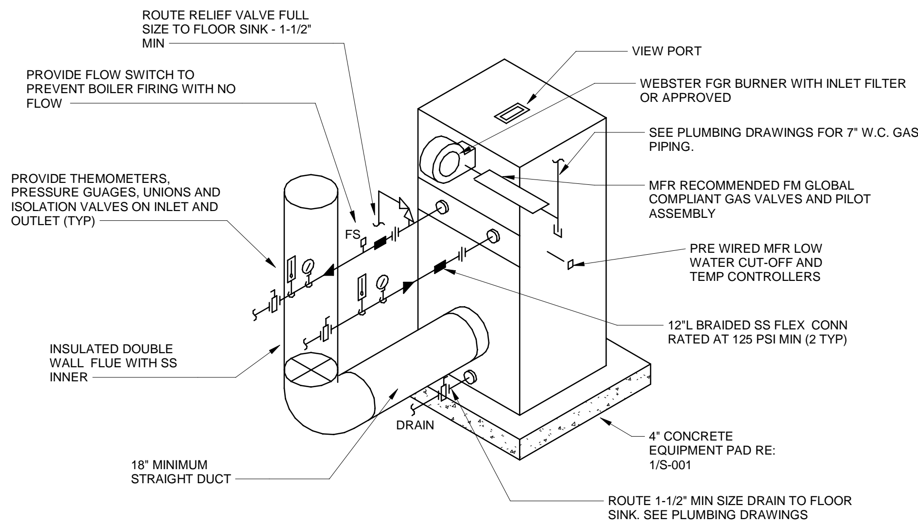
C1 HOT WATER BOILER PIPING DETAIL SCALE NTS
