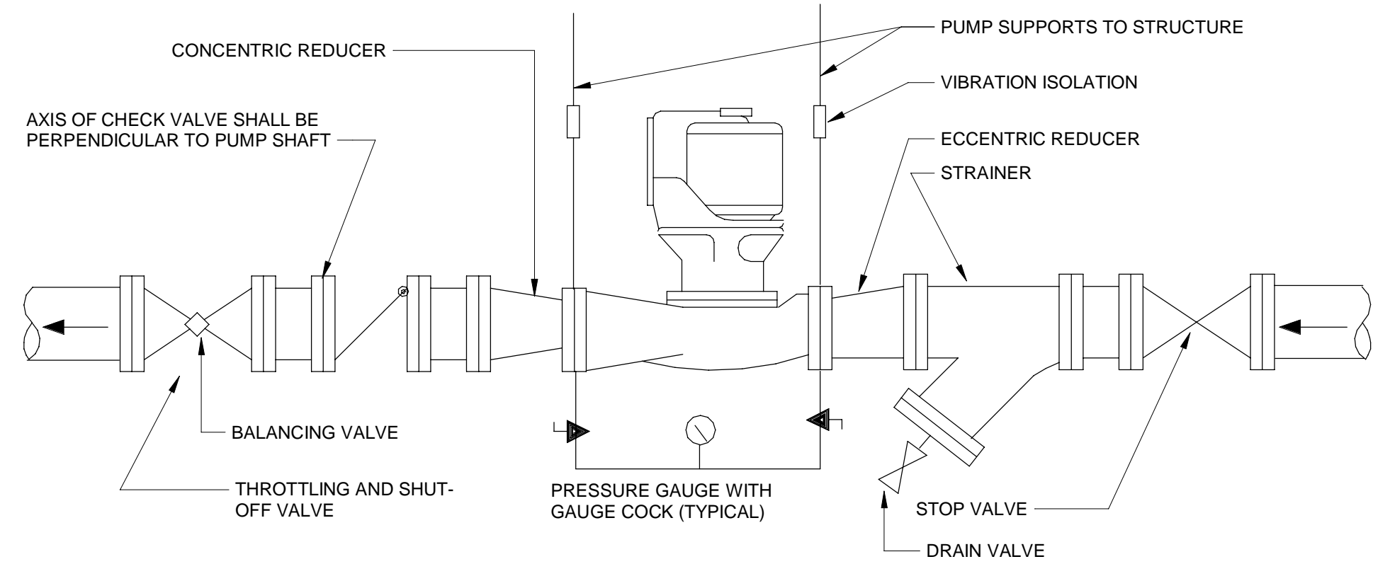
D1 INLINE PUMP PIPING SCALE NTS
