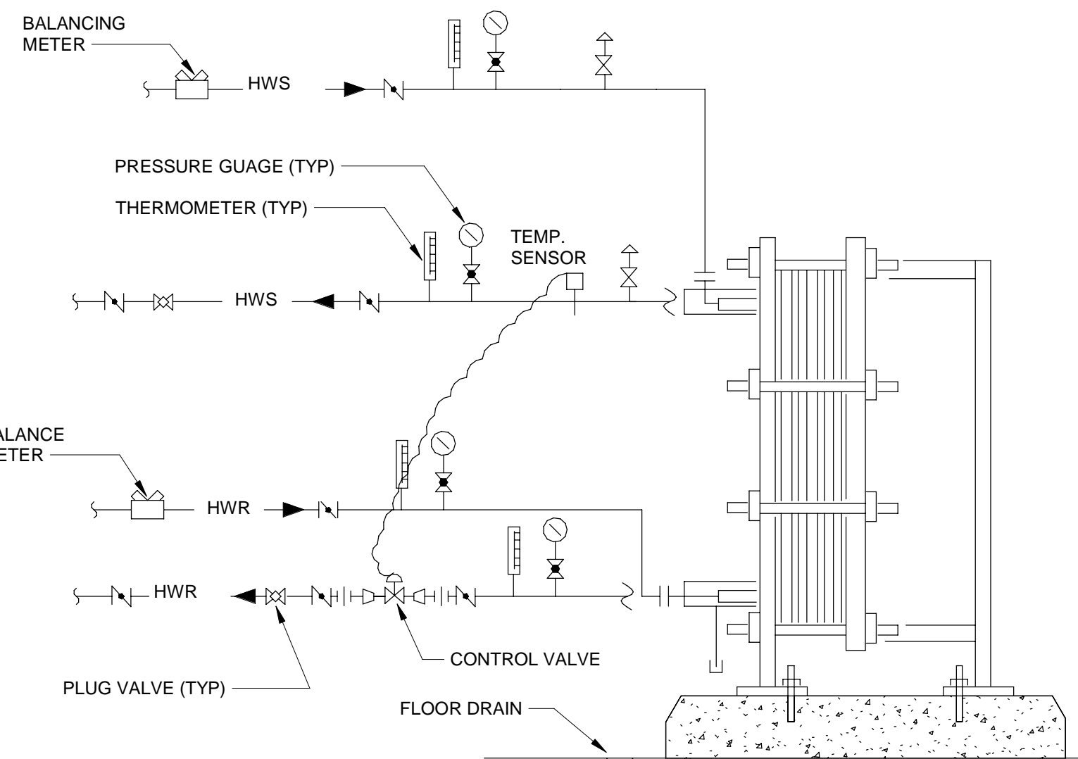
C3 PLATE AND FRAME HEAT EXCHANGER PIPING DETAIL SCALE NTS
