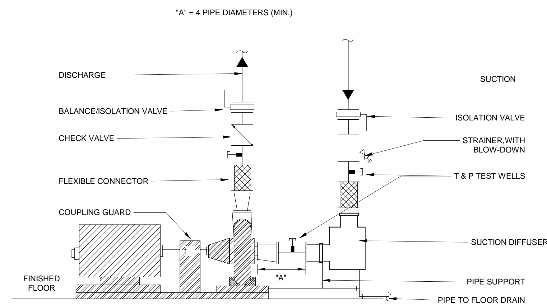
C5 END SUCTION PUMP SCALE NTS
