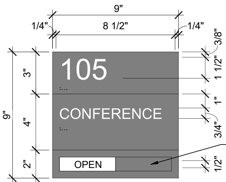
B1 RESTROOM IDENTIFICATION SIGN BB7 SCALE 3" = 1'-0"
