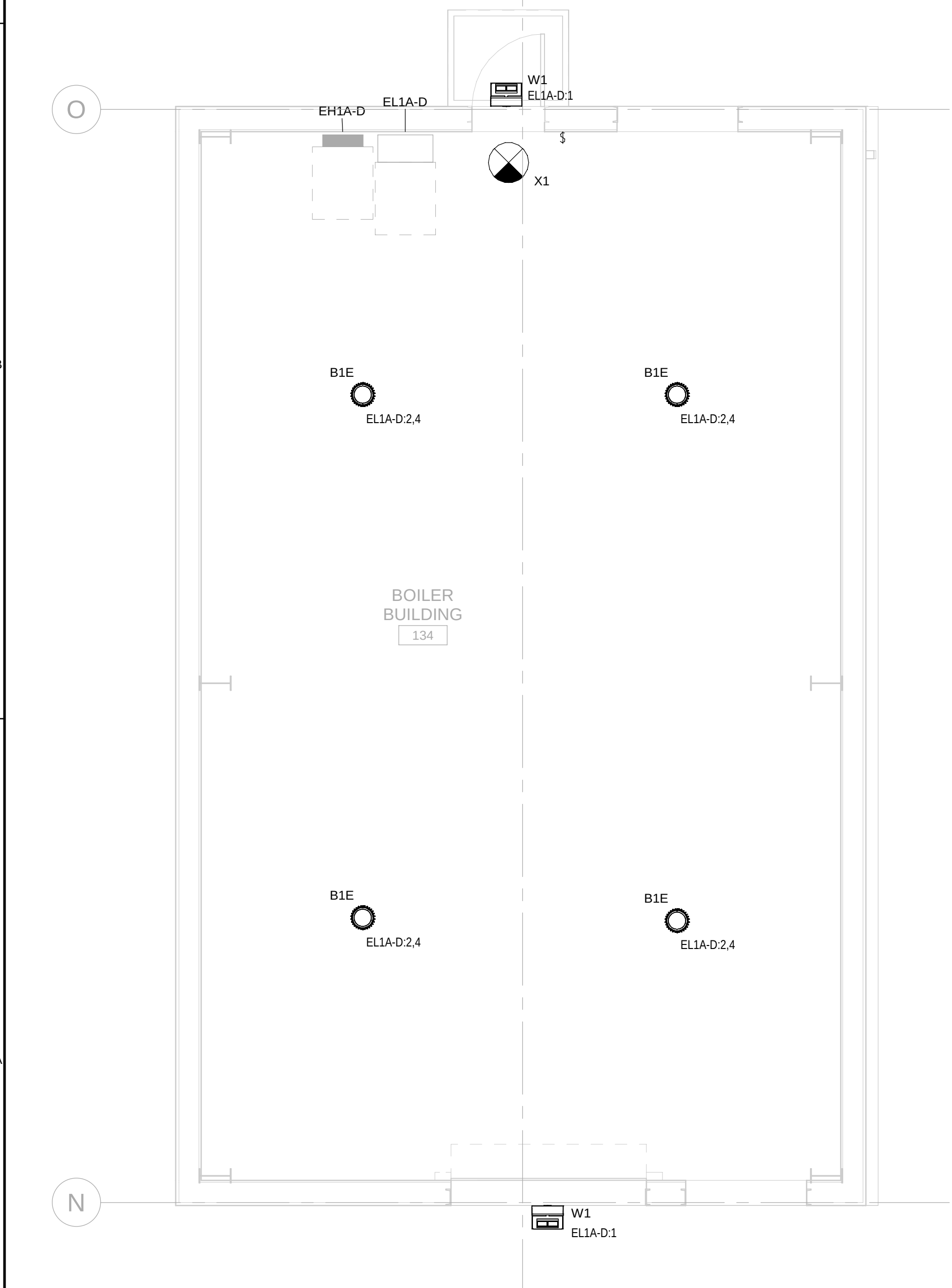
A1 ENLARGED LIGHTING PLAN - BOILER BLDG SCALE 1/4" = 1'-0"
