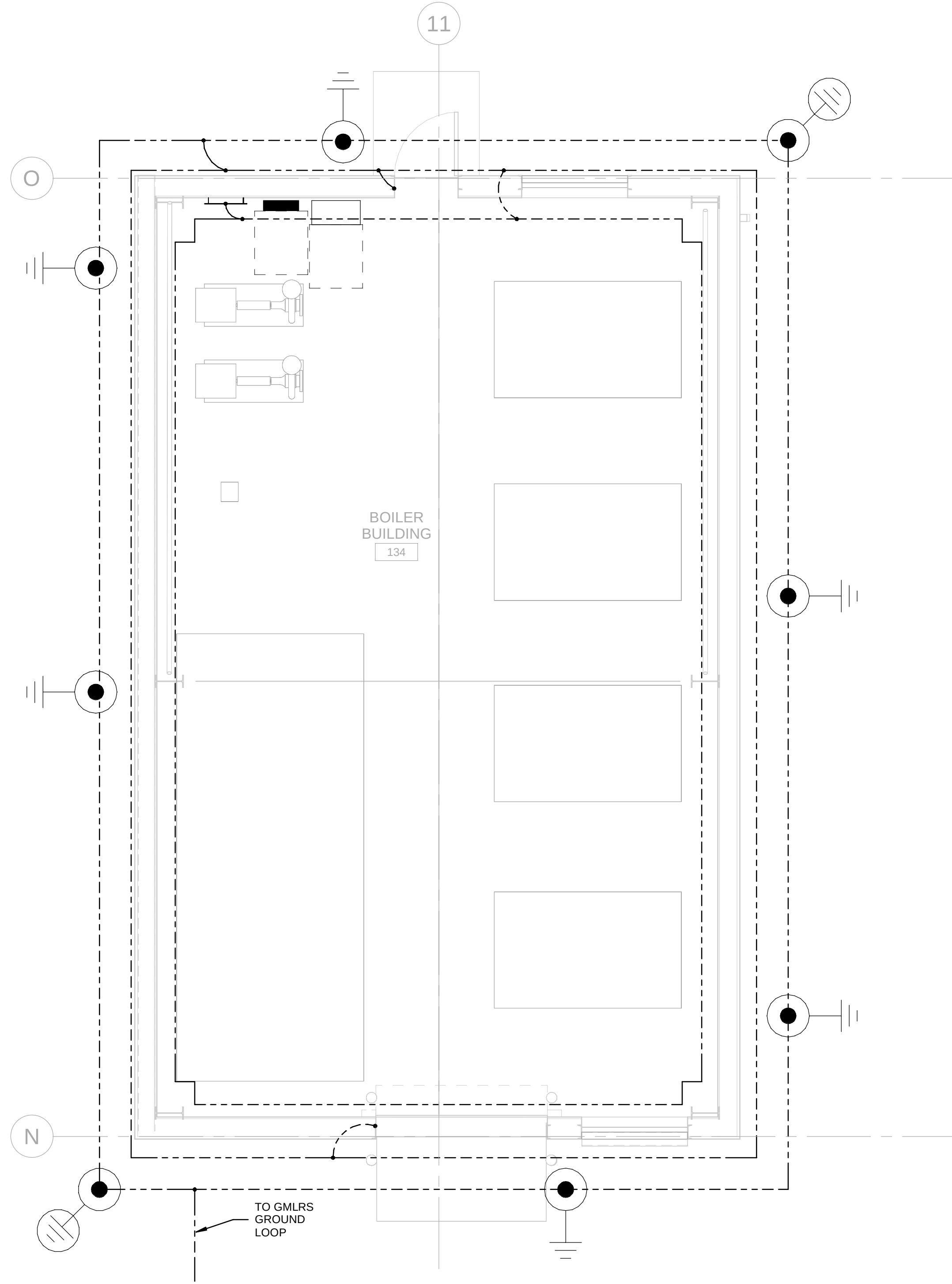
A3 ENLARGED GROUNDING PLAN - BOILER BLDG SCALE 1/4" = 1'-0"
