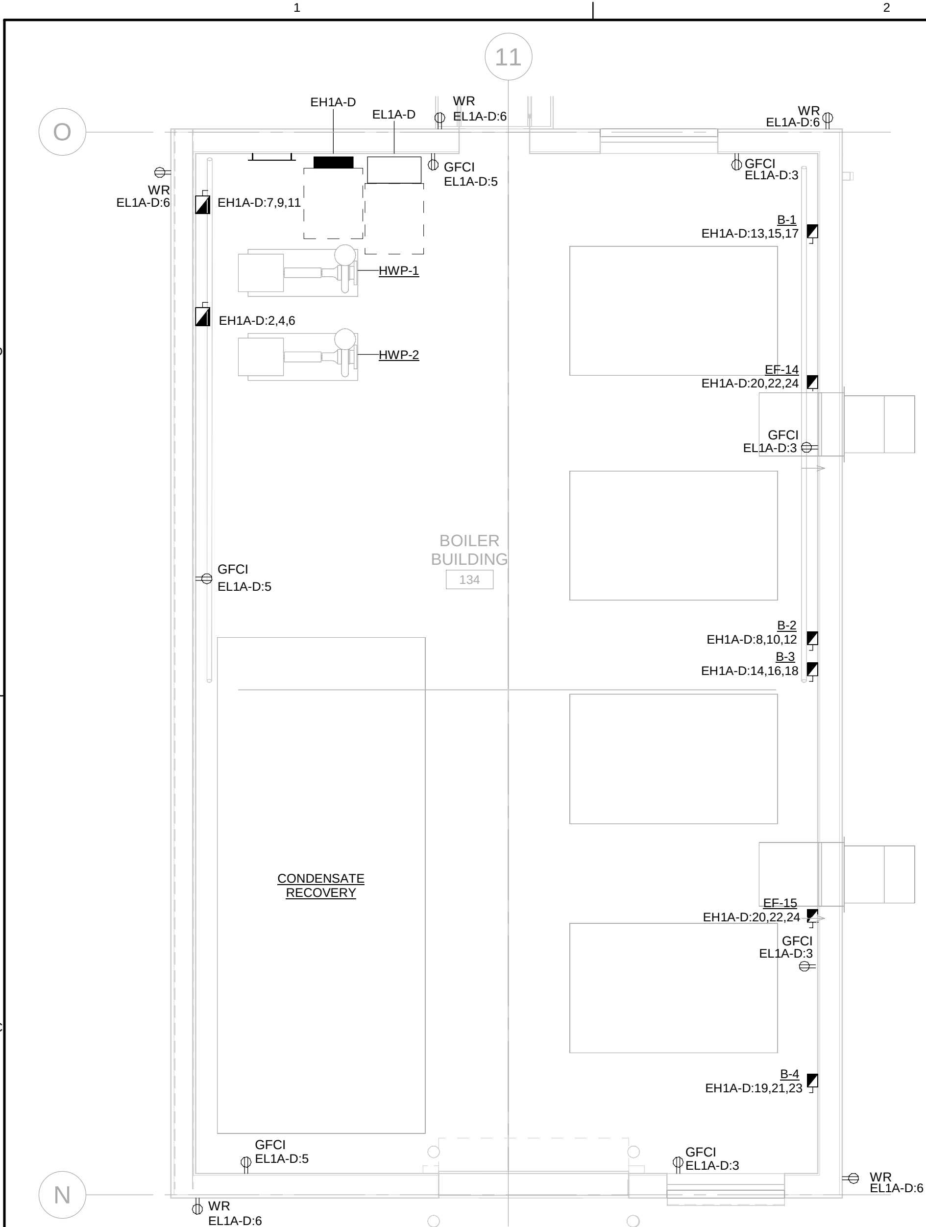
C1 ENLARGED POWER PLAN - BOILER BLDG SCALE 1/4" = 1'-0"
