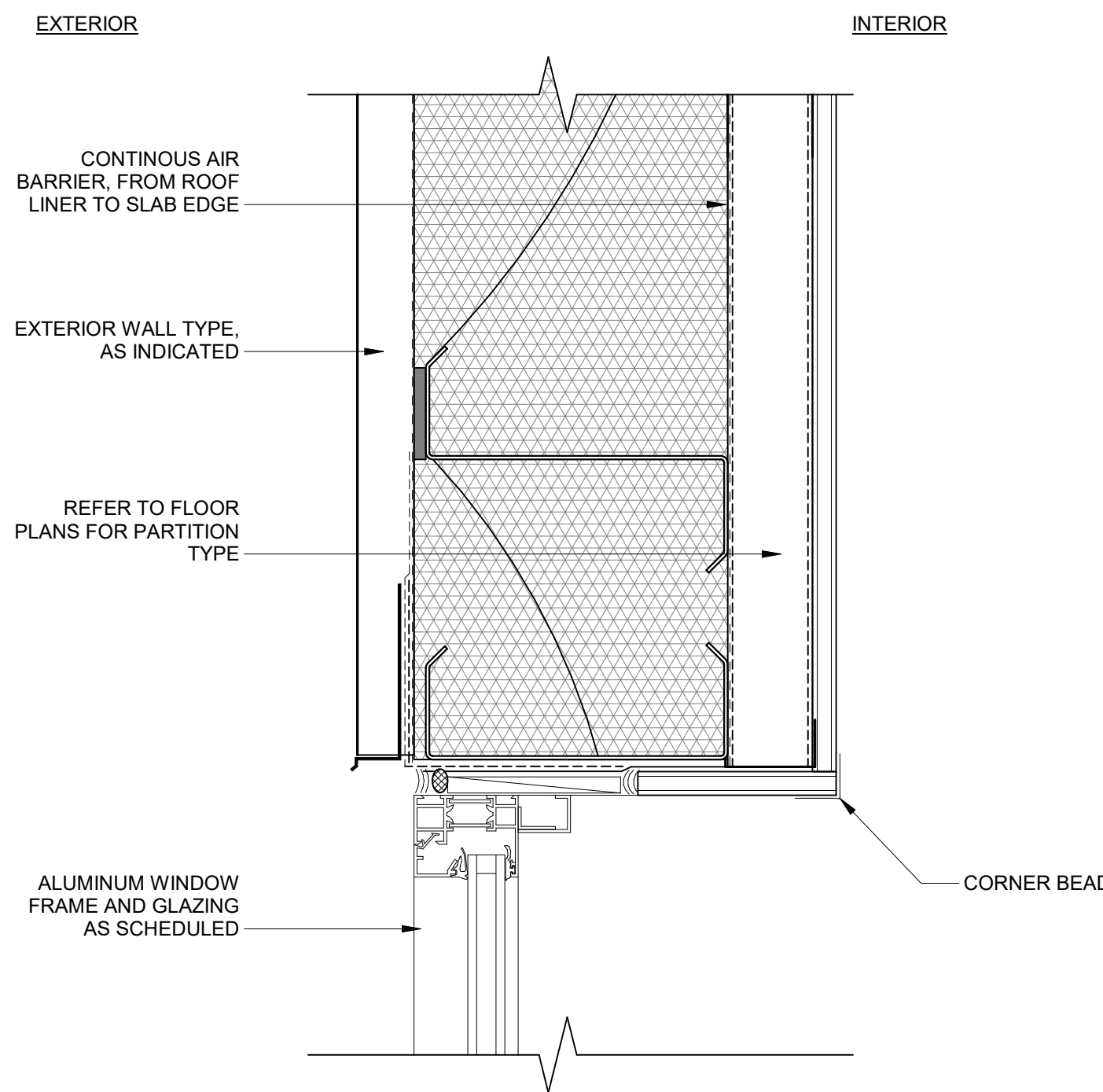
C4 WINDOW HEAD AT MP-3 SCALE 3" = 1'-0"
