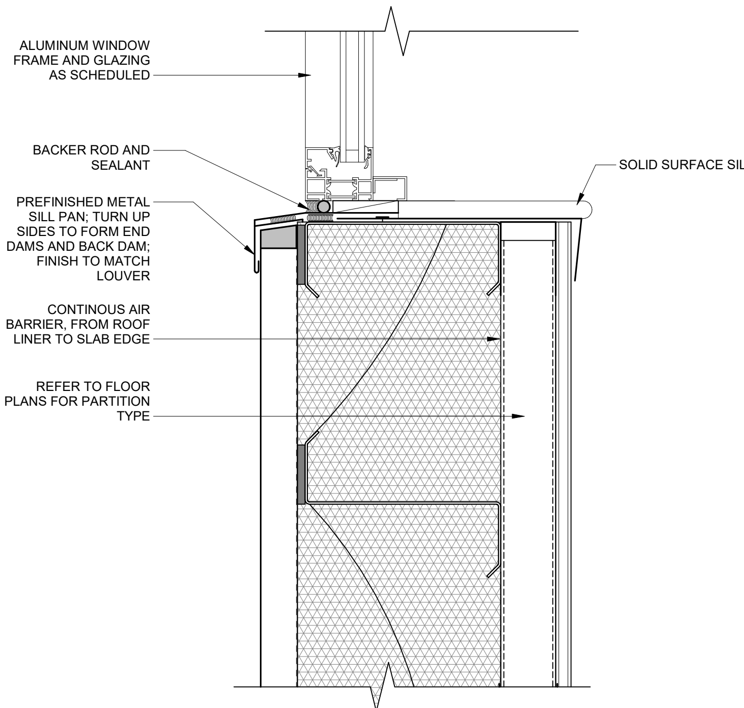
A4 WINDOW SILL AT MP-3 SCALE 3" = 1'-0"
