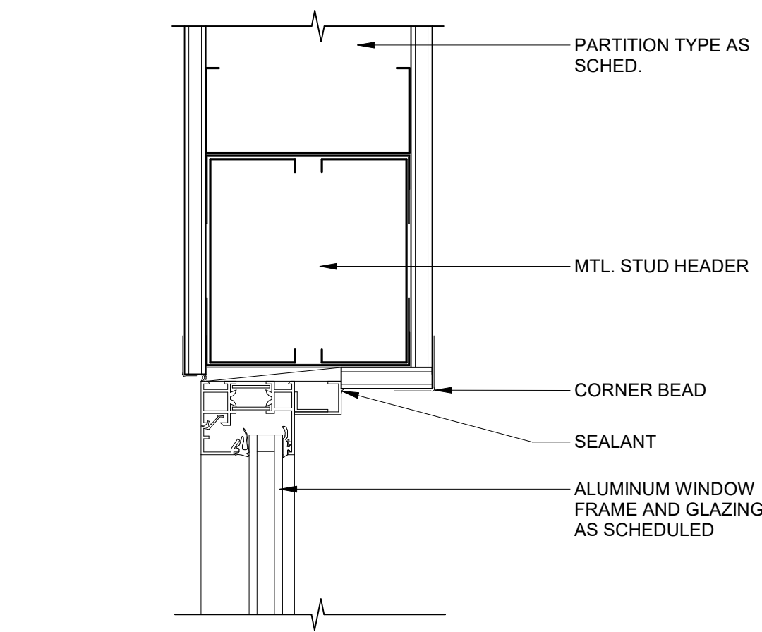
C3 WINDOW HEAD AT INTERIOR PARTITION SCALE 3" = 1'-0"
