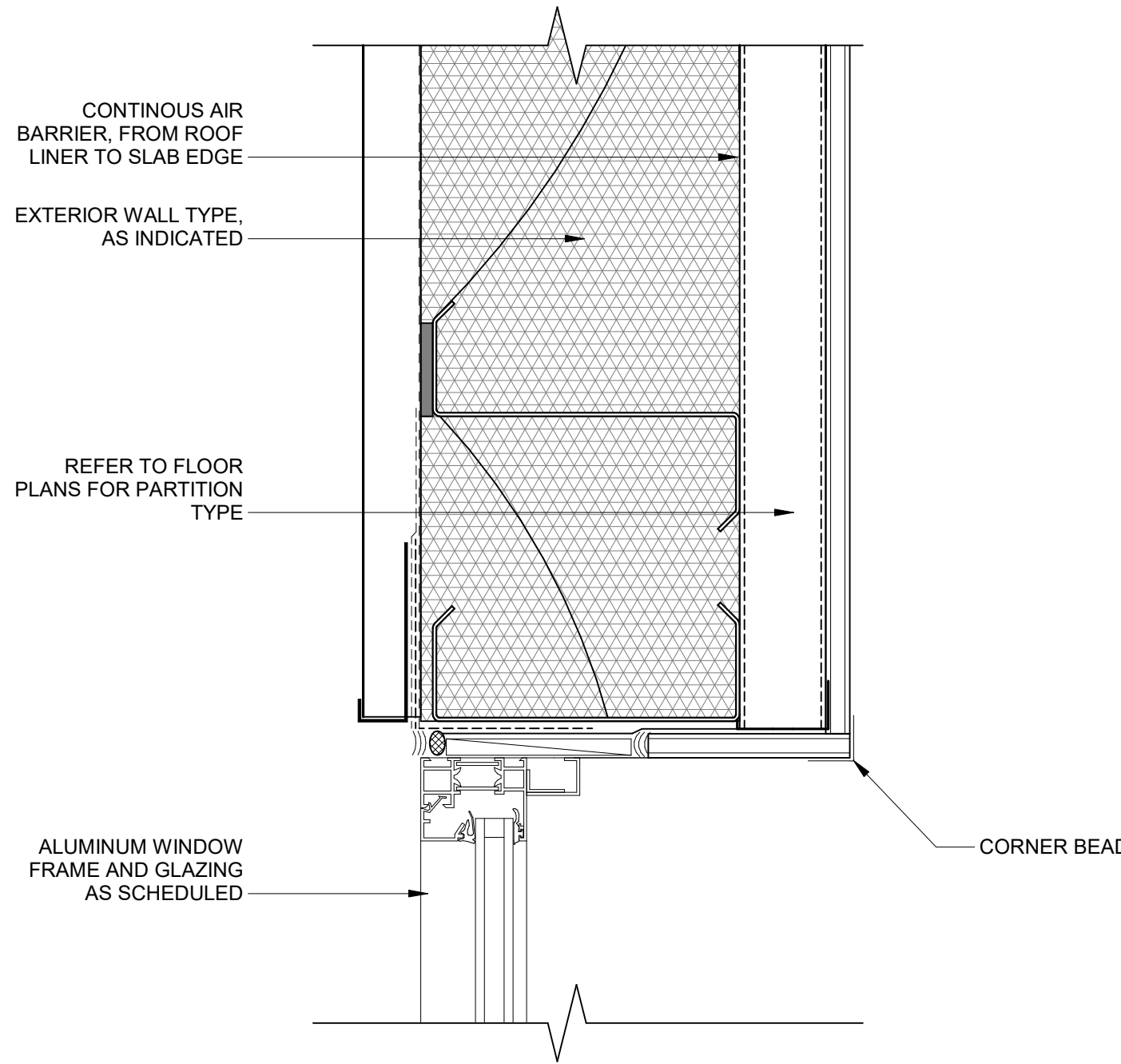
B4 WINDOW JAMB AT MP-3 SCALE 3" = 1'-0"
