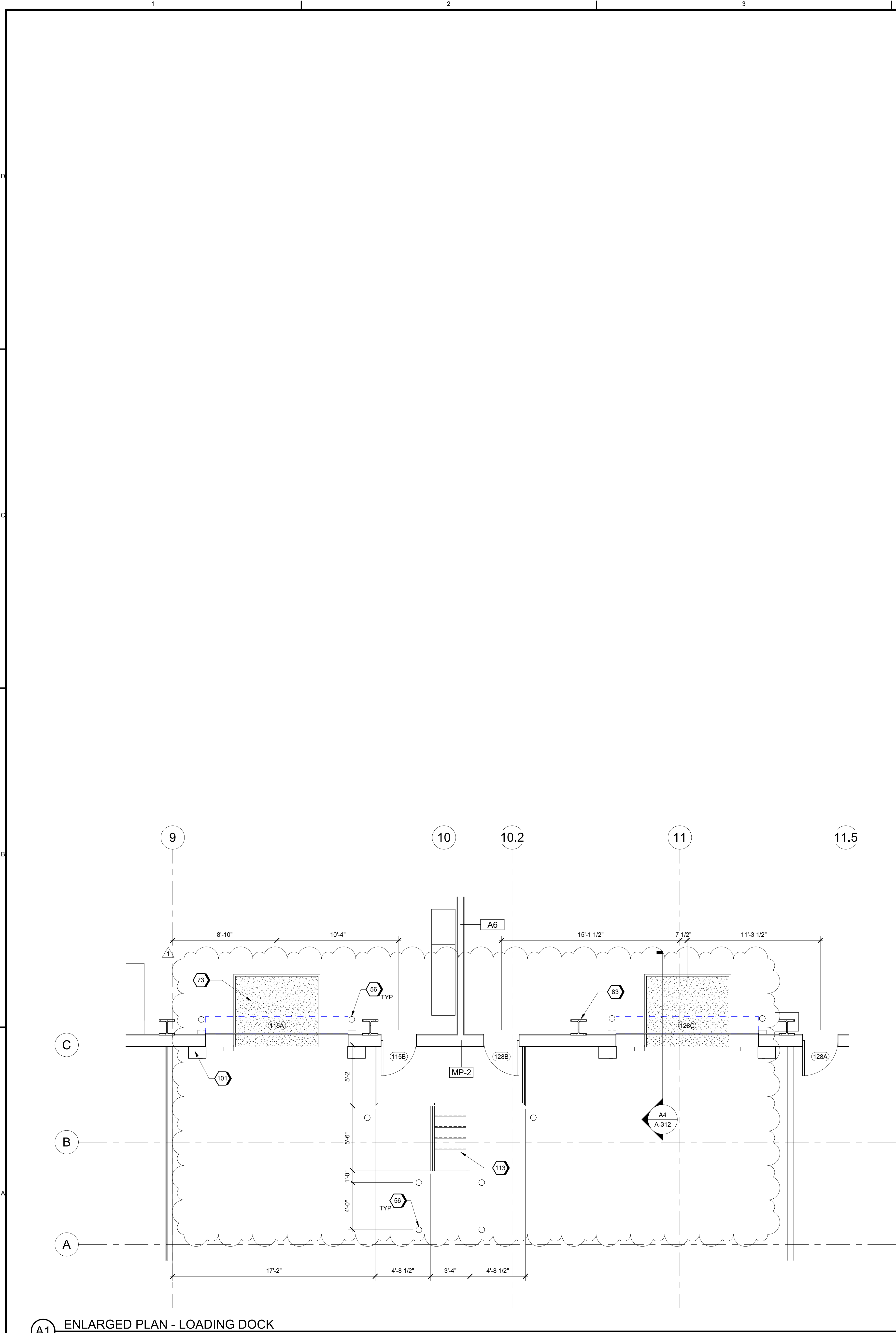
A1 ENLARGED PLAN - LOADING DOCK SCALE 1/4" = 1'-0"
