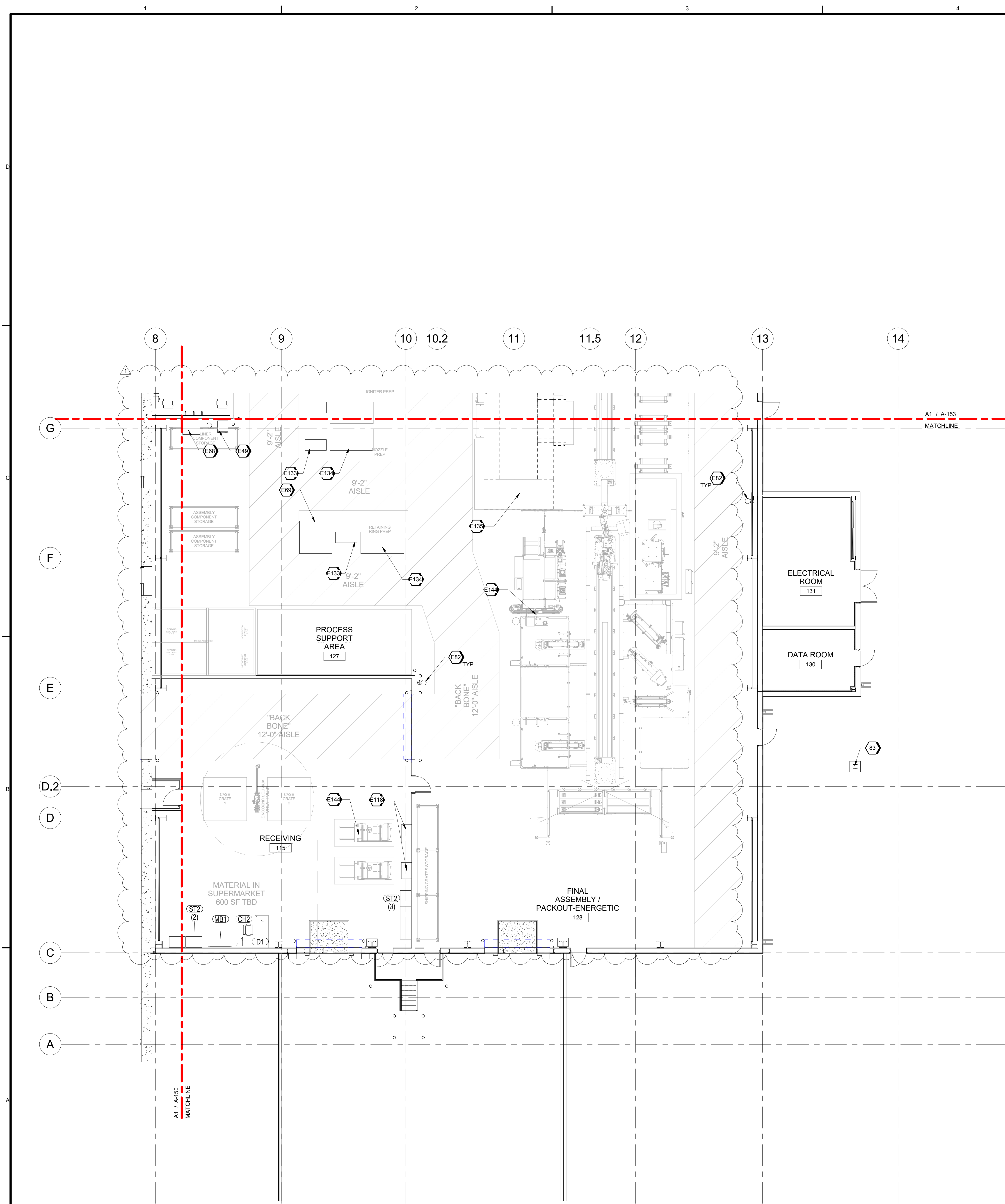
A1 PARTIAL EQUIPMENT PLAN - AREA C SCALE 1/8" = 1'-0"
