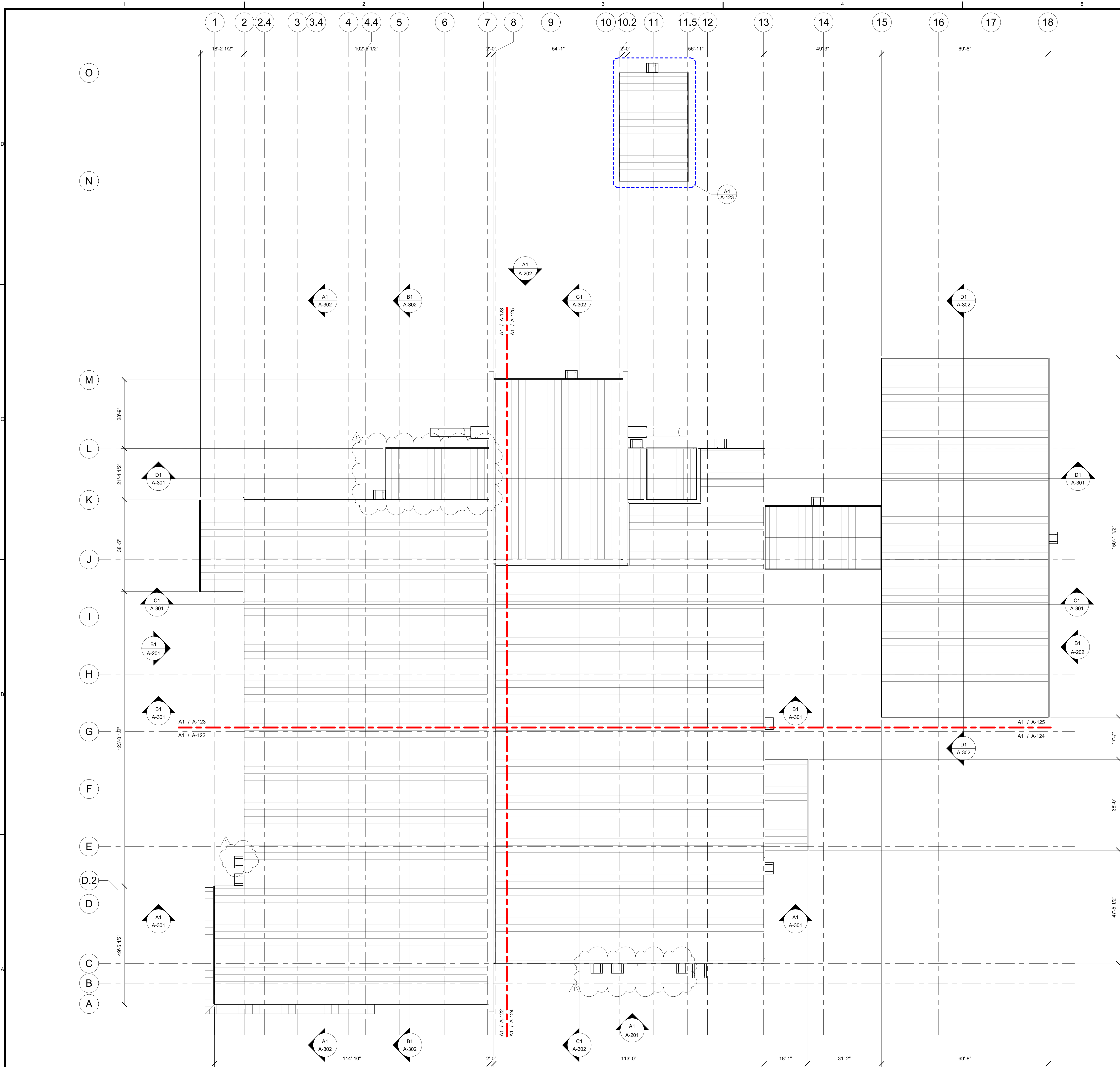
A1 OVERALL ROOF PLAN SCALE 1/16" = 1'-0"
