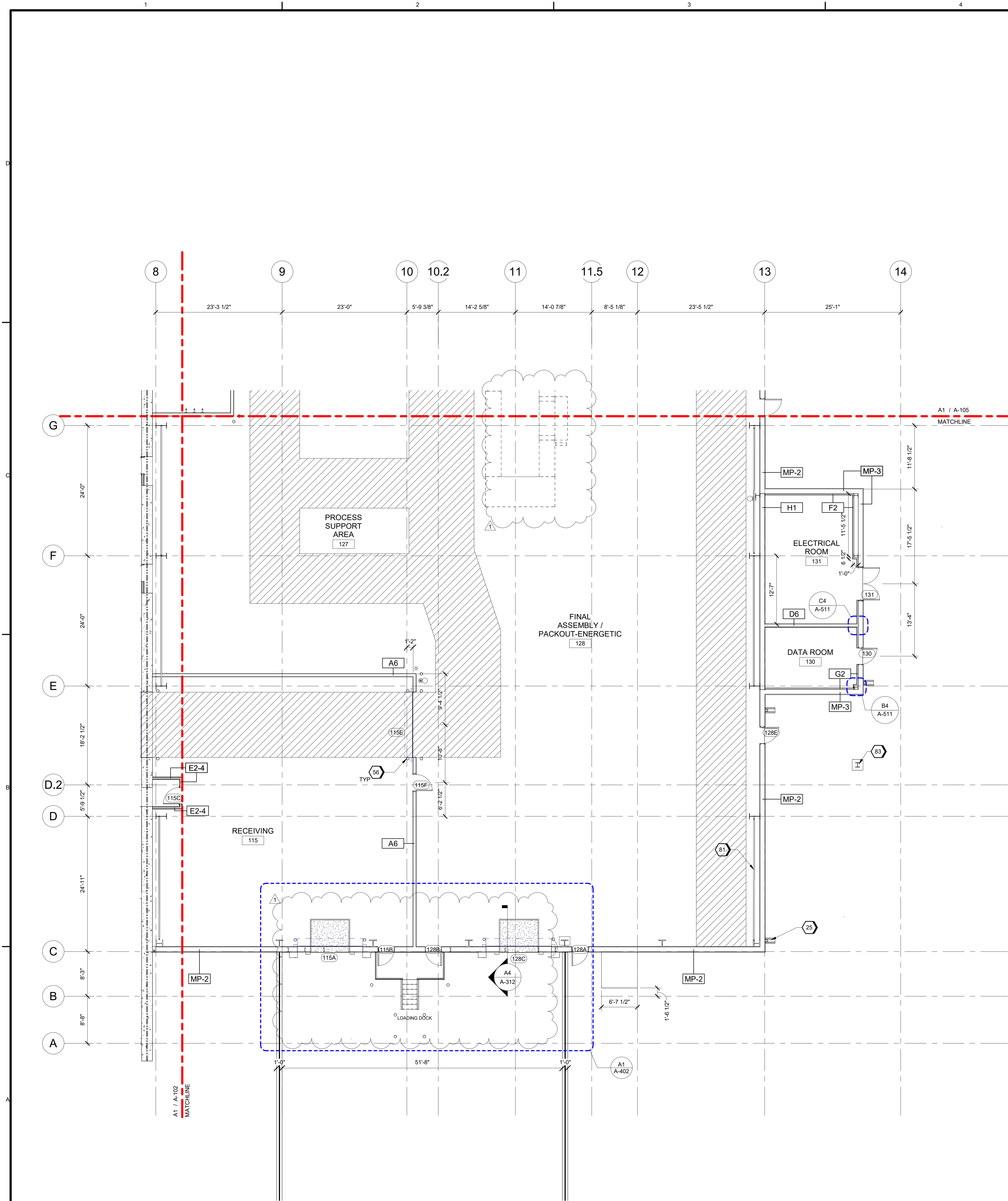
A1 PARTIAL FLOOR PLAN - AREA C SCALE 1/8" = 1'-0"
