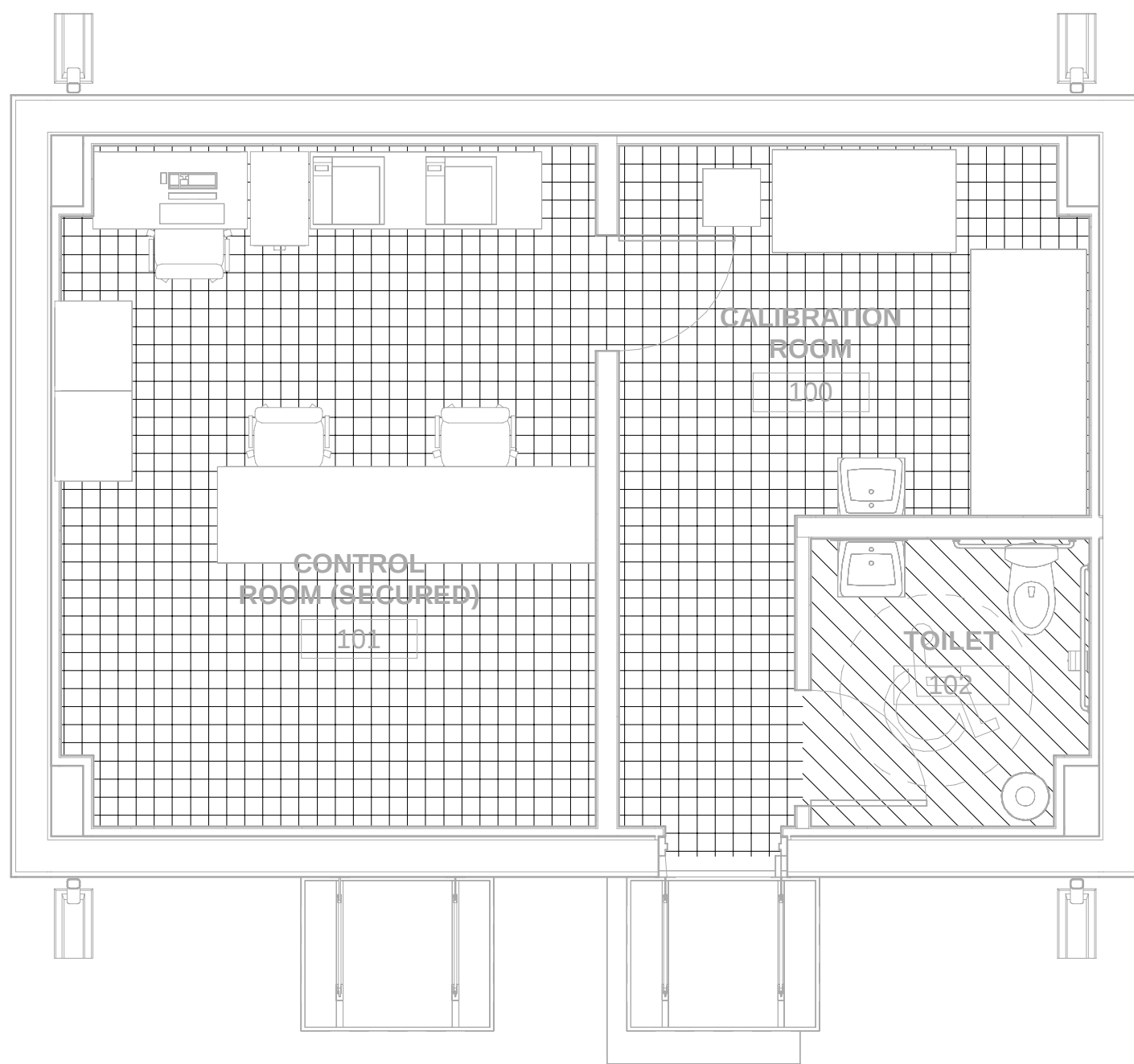
A1 HVAC ZONE MAP SCALE 1/4" = 1'-0"
