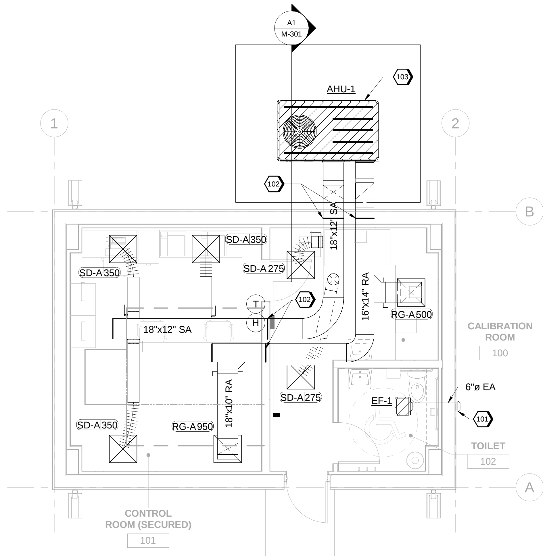
A3 MECHANICAL FLOOR PLAN SCALE 1/4" = 1'-0"
