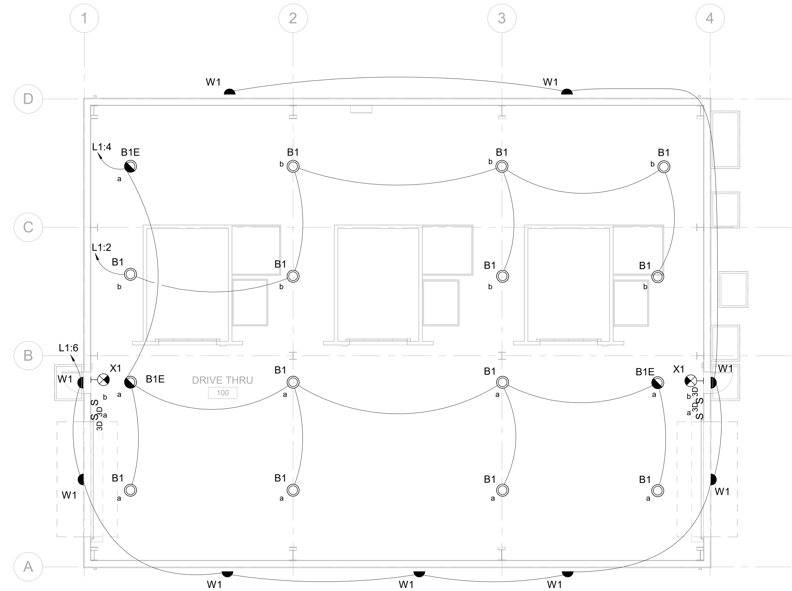
(A1) LIGHTING PLAN SCALE 1/8" = 1'-0"
