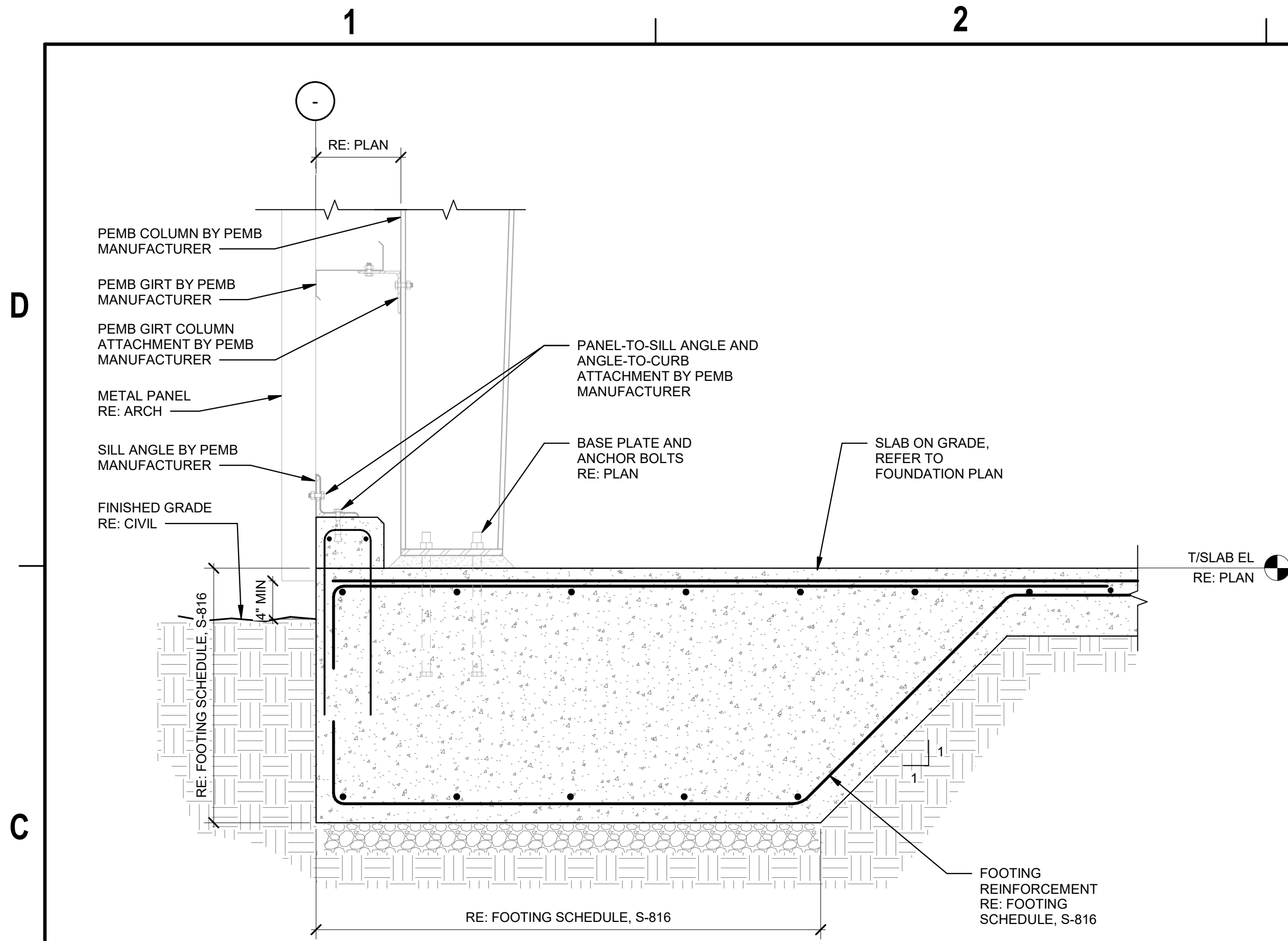
C1 THICKENED SLAB SCALE 1" = 1'-0"
