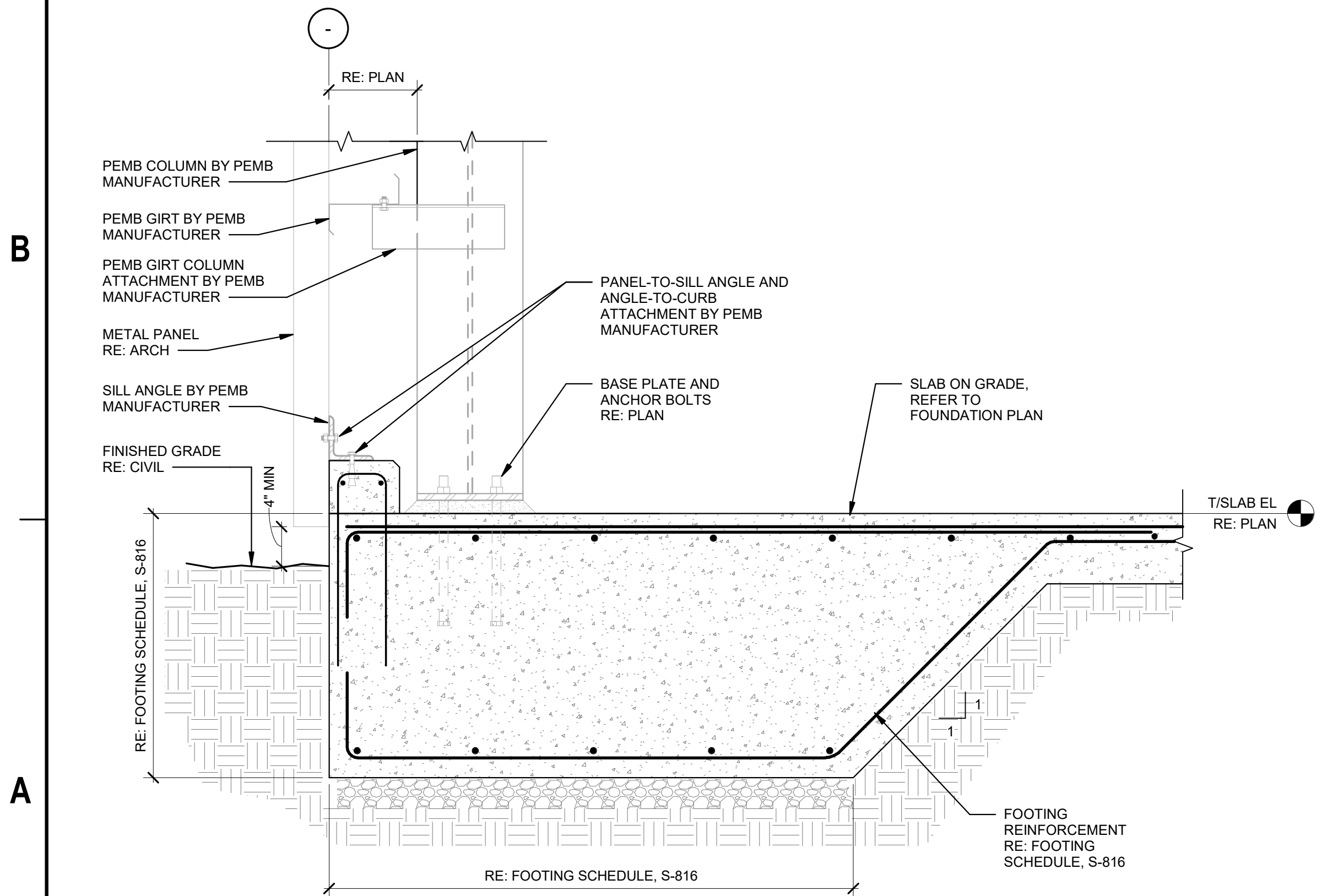
A1 THICKENED SLAB SCALE 1" = 1'-0"
