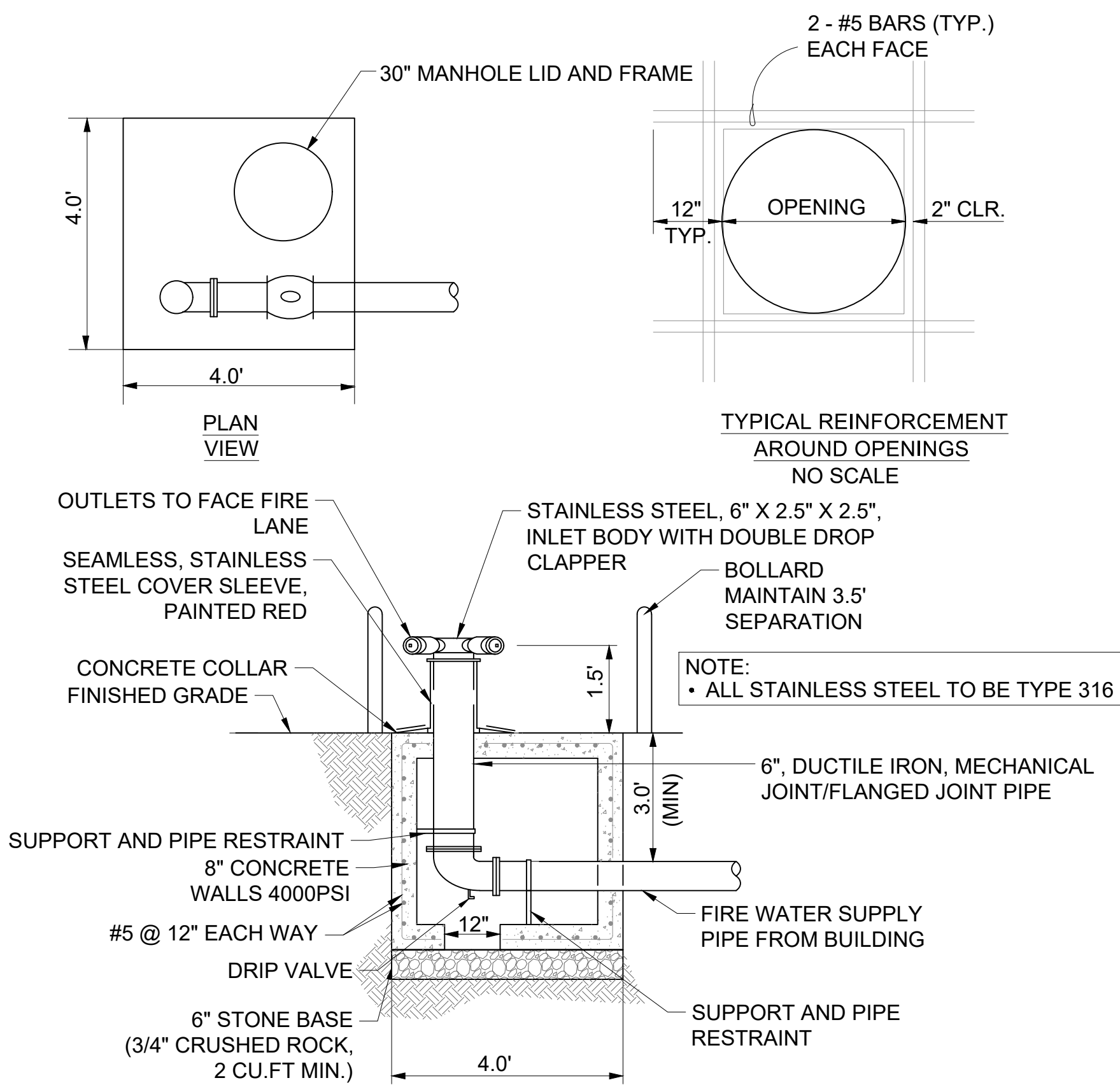
B1 FREE STANDING FIRE DEPARTMENT CONNECTION SCALE N.T.S.
