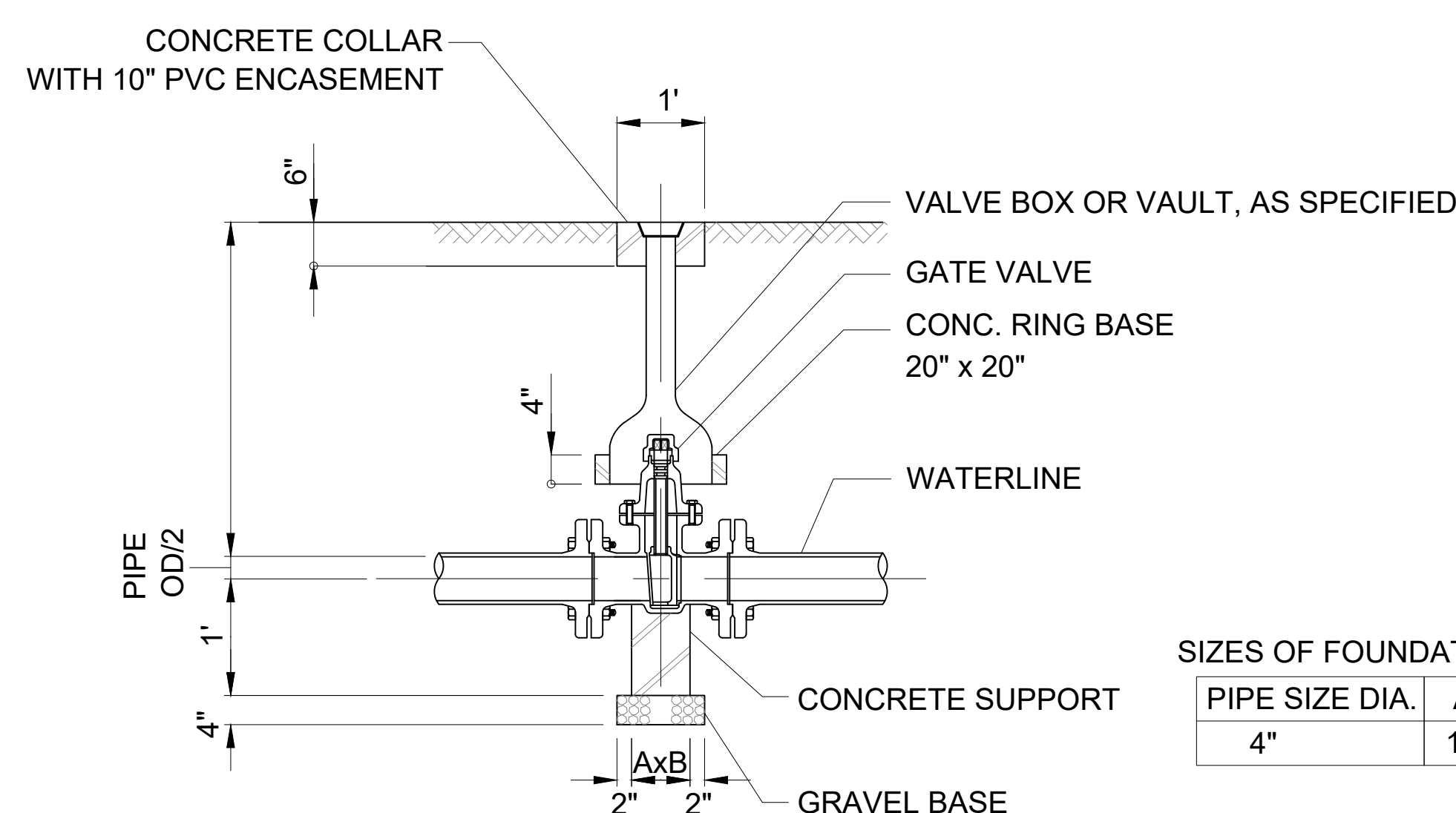
A3 GATE VALVE DETAIL SCALE NTS
