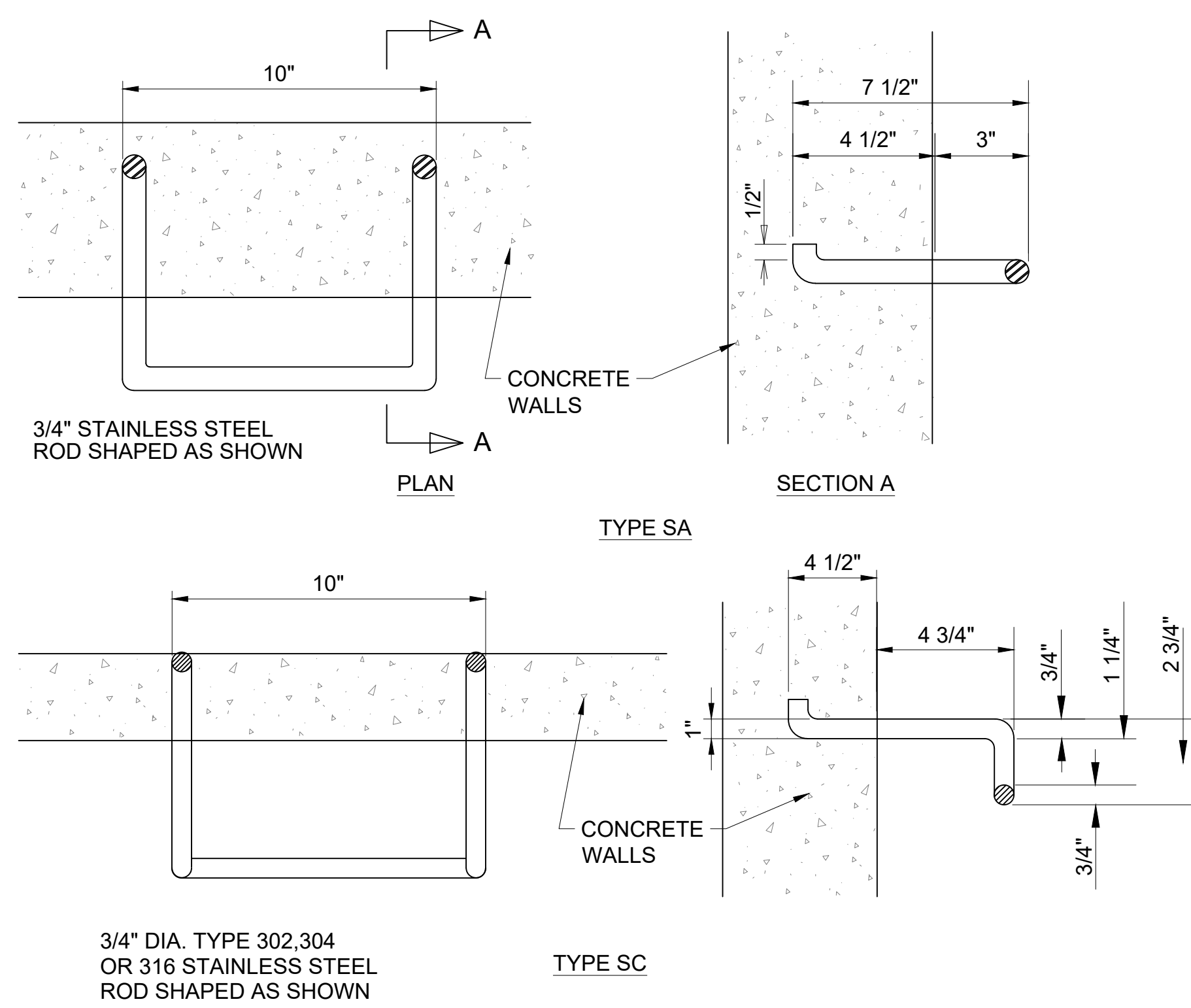
C3 MANHOLE RUNG DETAIL SCALE NTS
