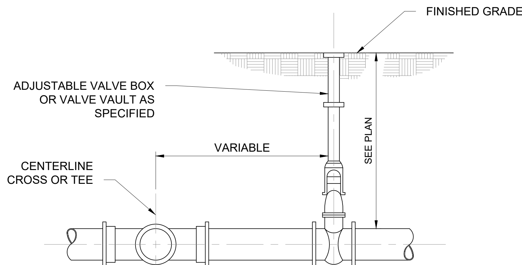
A1 TYPICAL VALVE SETTING SCALE N.T.S.
