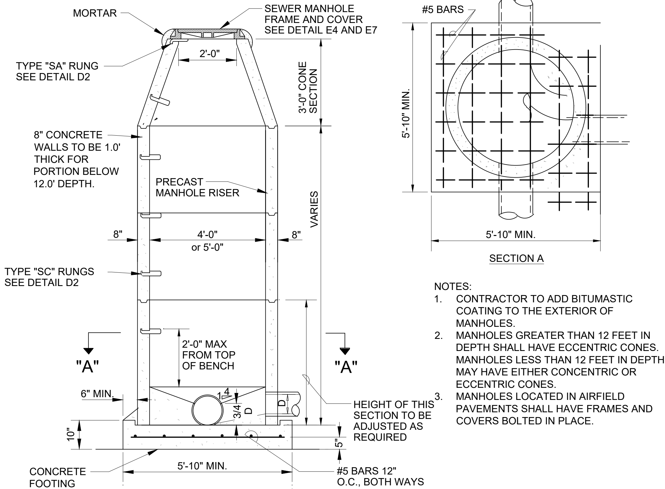
C1 SANITARY SEWER PRECAST MANHOLE (TYPE B) DETAIL SCALE NTS
