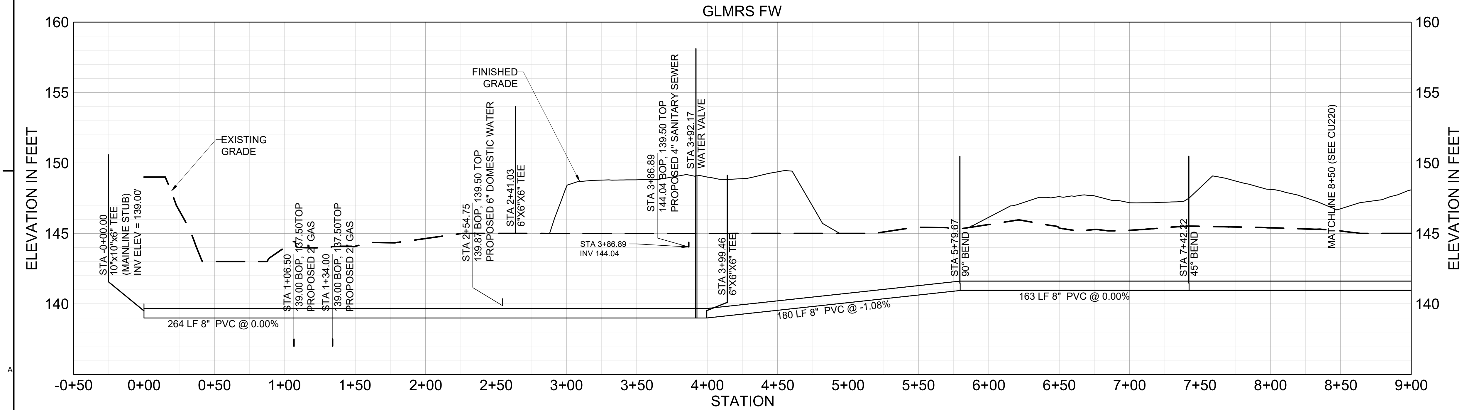
A1 FIRELINE PROFILE - GMLRS 1 VERTICAL SCALE 1"=4' HORIZONTAL SCALE 1"=40'
