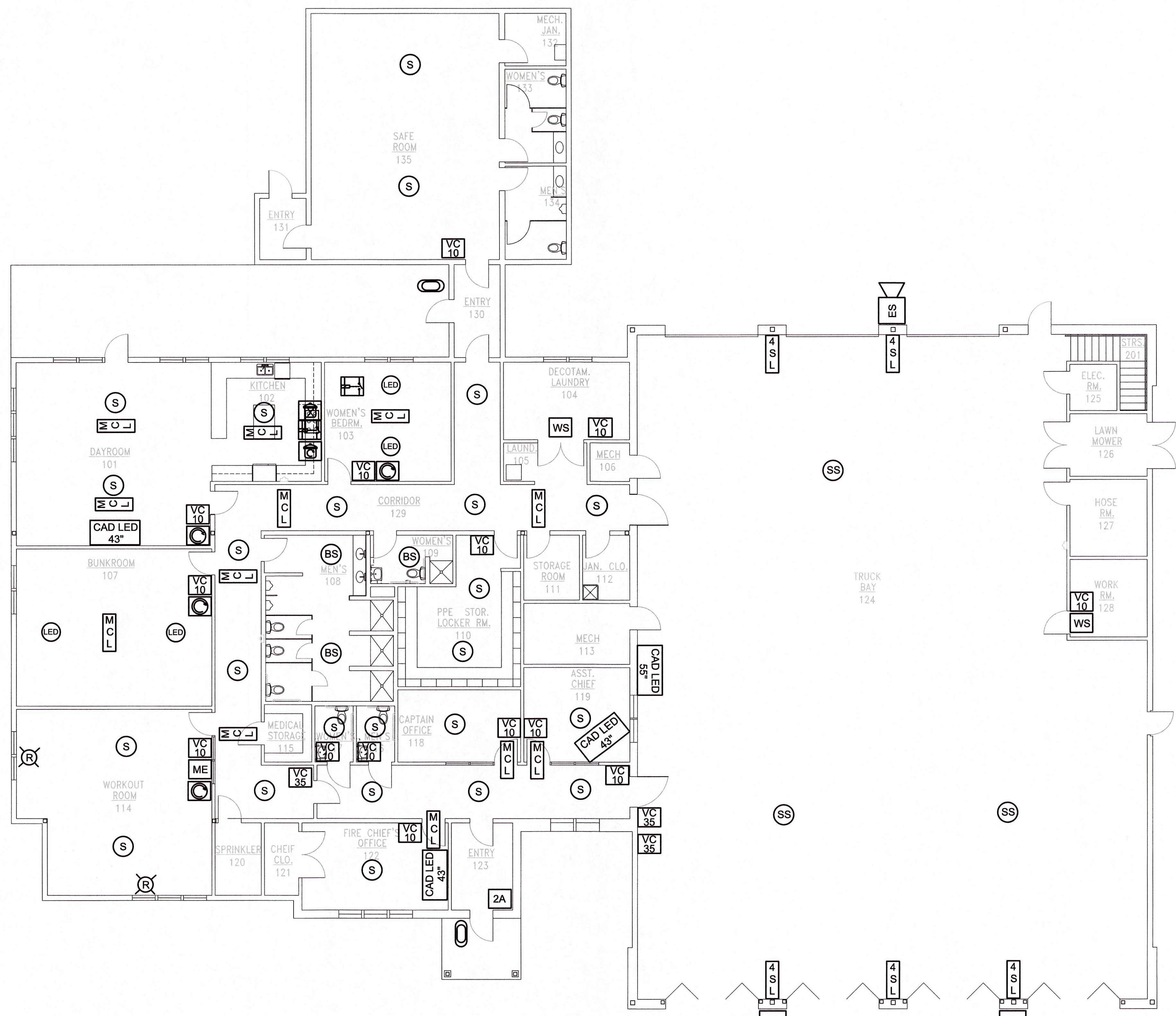
FIRE STATION ALERTING SYSTEM SCALE: 1/8" = 1'-0"
