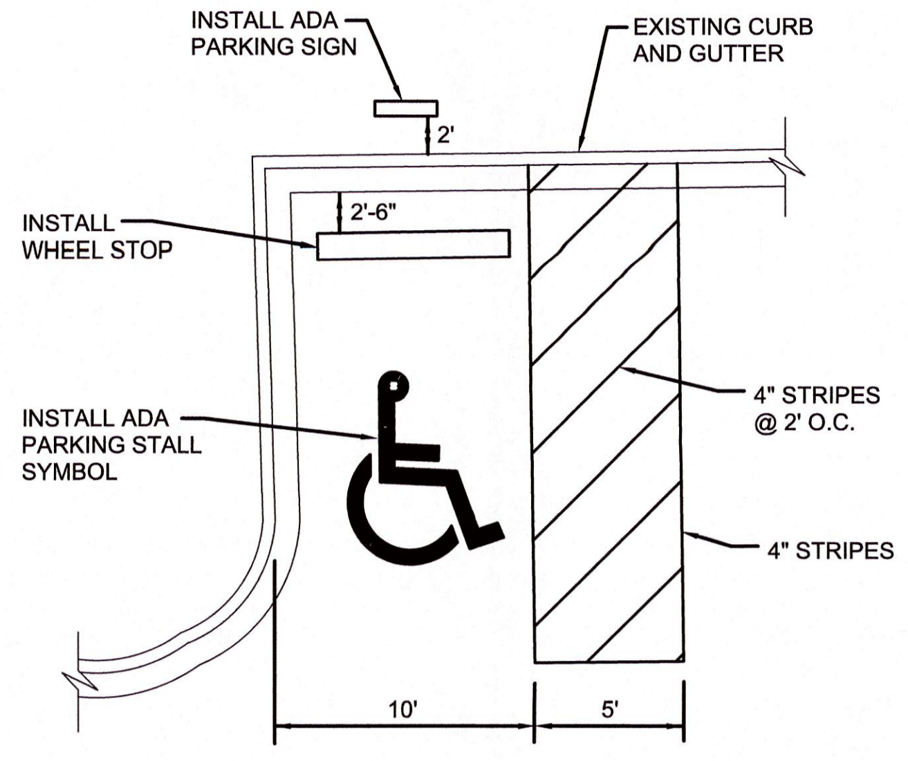
ADA PARKING STRIPING DETAIL B
