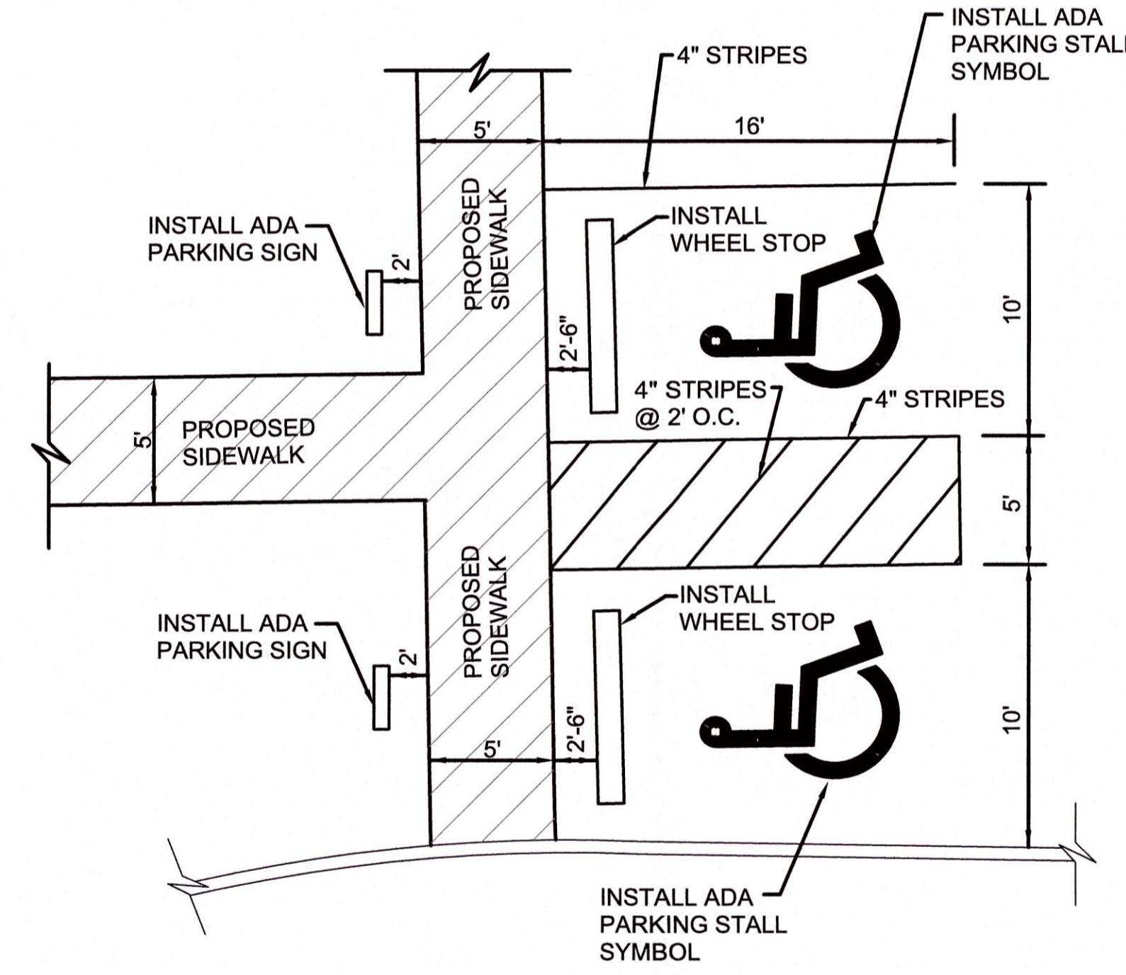
ADA PARKING STRIPING DETAIL A
