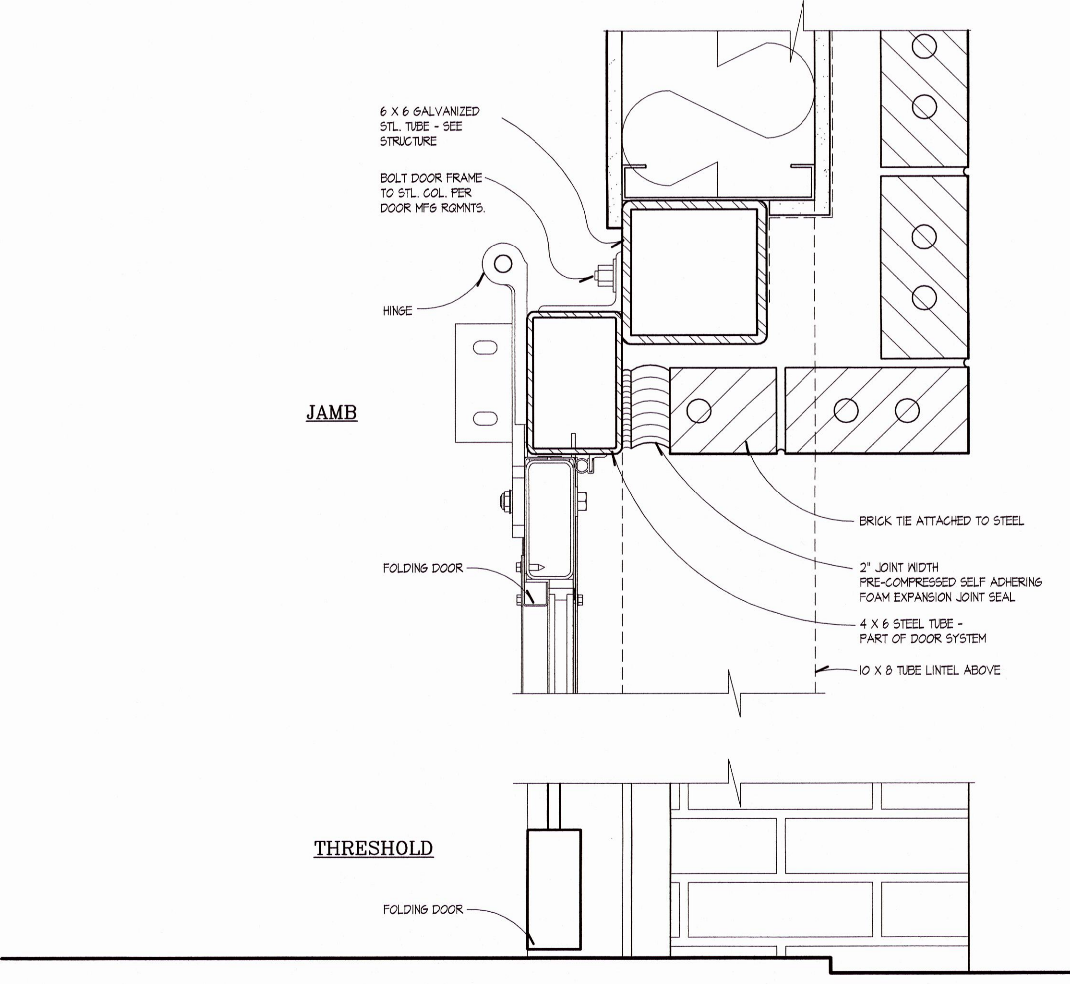
4 FOLDING DOOR HJS DETAIL A603 SCALE: 3" = 1'-0"
