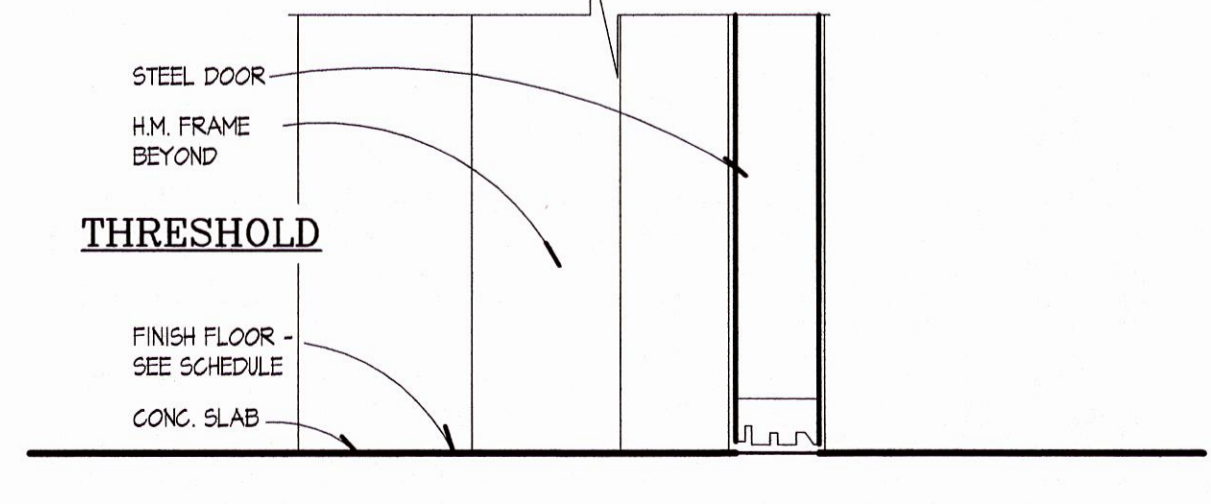
2 DOOR HJS DETAIL A603 SCALE: 3" = 1'-0"
