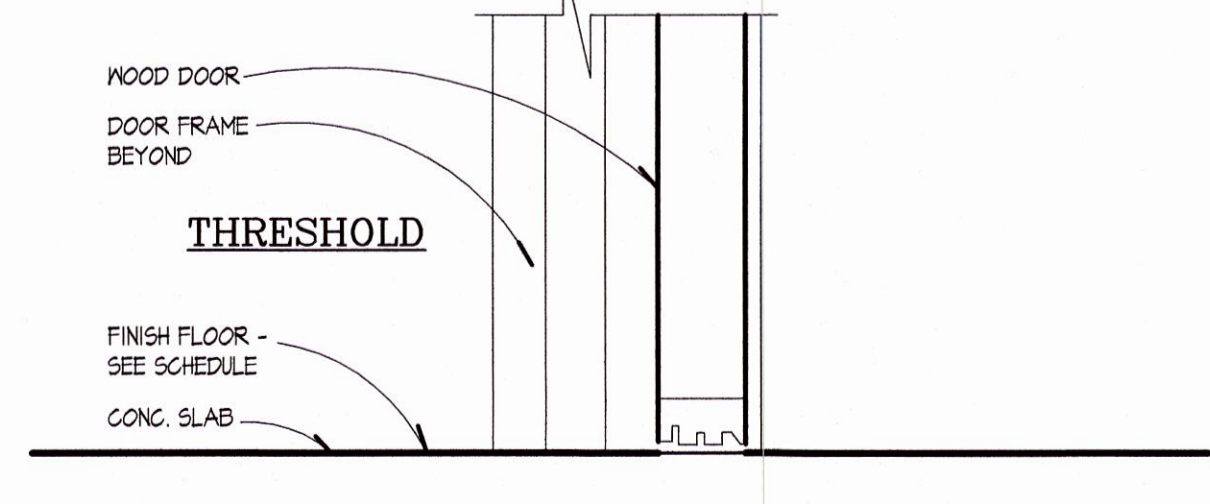
1 DOOR HJS DETAIL A603 SCALE: 3" = 1'-0"
