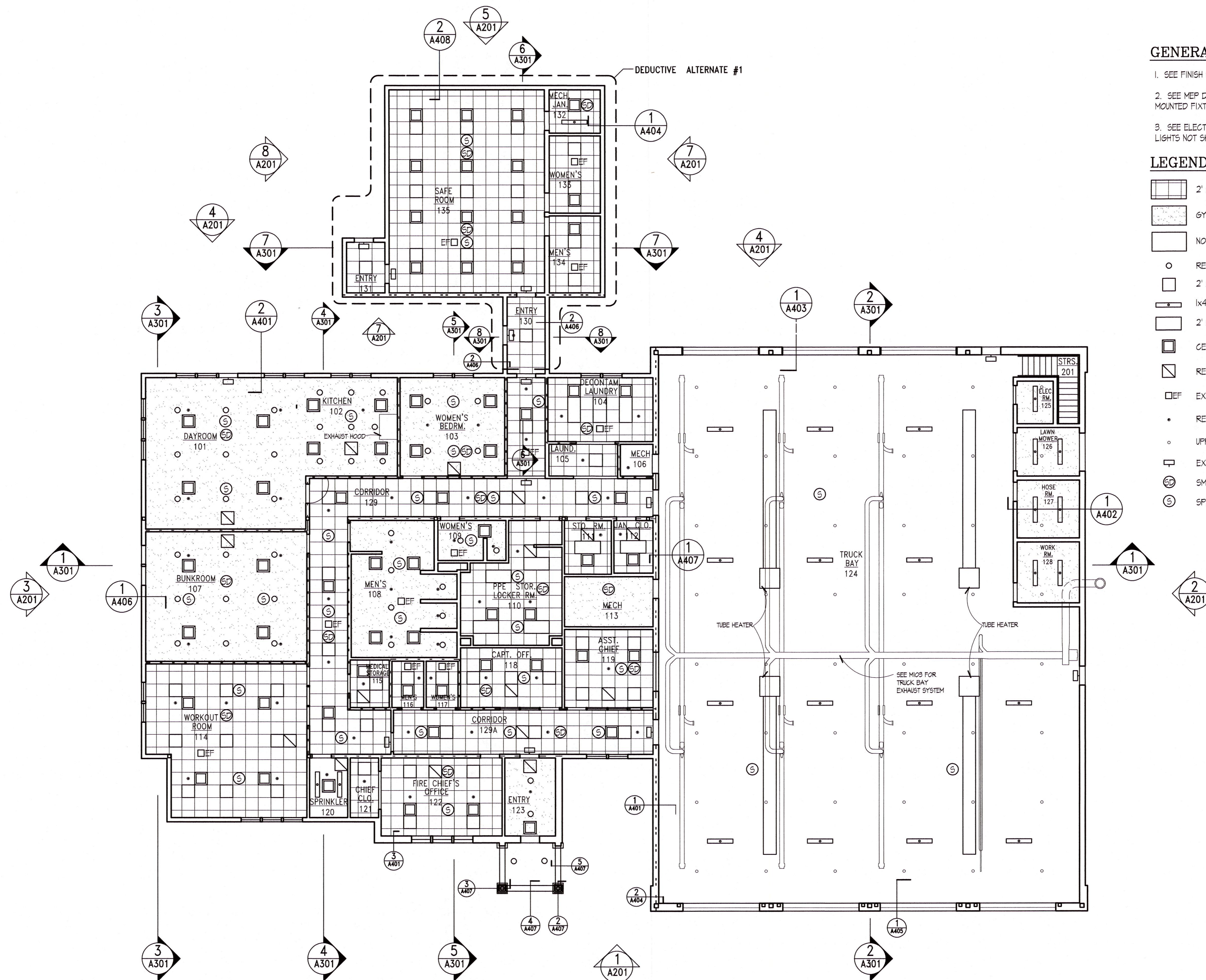
1 REFLECTED CEILING PLAN A101 SCALE: 1/8" = 1'-0"
