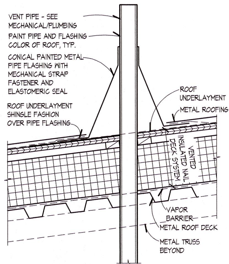
2 ROOF VENT PIPE A102 SCALE: 1 1/2" = 1'-0"
