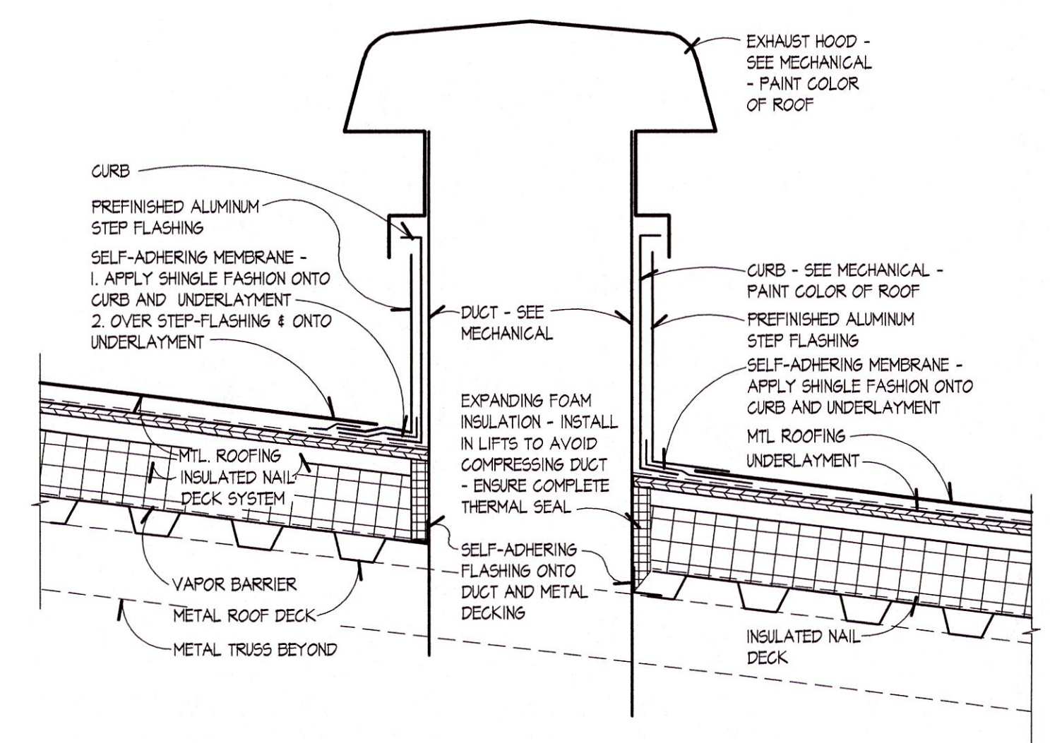
3 ROOF EXHAUST HOOD A102 SCALE: 1 1/2" = 1'-0"
